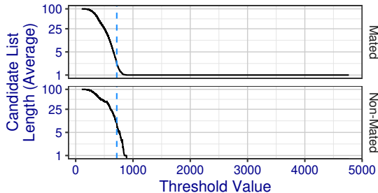
The similarity score indicated in blue is the threshold at which griale+100F achieves 10% FPIR.
