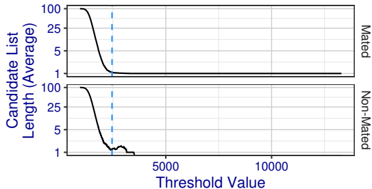
The similarity score indicated in blue is the threshold at which idemia+0004 achieves 10% FPIR.
