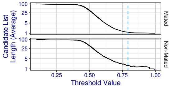
The similarity score indicated in blue is the threshold at which roc+0016 achieves 10% FPIR.
