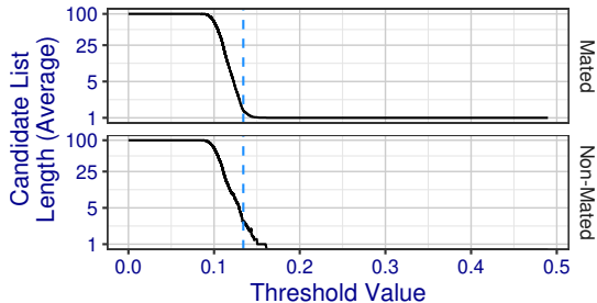
The similarity score indicated in blue is the threshold at which tech5impl+0004 achieves 10% FPIR.
