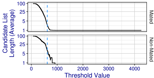
The similarity score indicated in blue is the threshold at which griaule+100D achieves 10% FPIR.
