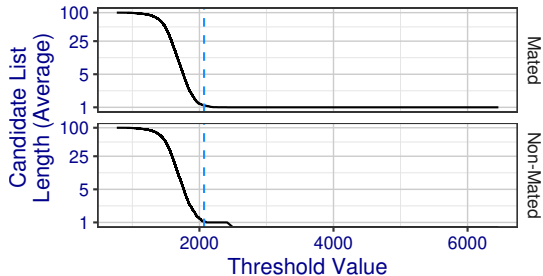
The similarity score indicated in blue is the threshold at which idemia+0008 achieves 10% FPIR.
