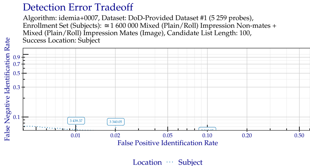
Figure 19: DET when searching DoD-Provided Dataset #1 probes. Annotated values indicate similarity scores from the Subject line.
