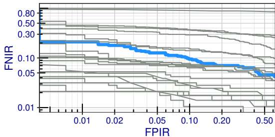
griaule+1011 is highlighted in blue, alongside all other algorithms in gray (algorithms target the lower-left).
