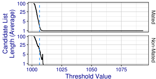
The similarity score indicated in blue is the threshold at which griaule+1011 achieves 10% FPIR.
