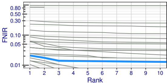
griaule+1011 is highlighted in blue, alongside all other algorithms in gray (lower is better).
