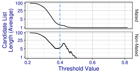
The similarity score indicated in blue is the threshold at which papil111+0010 achieves 10% FPIR.
