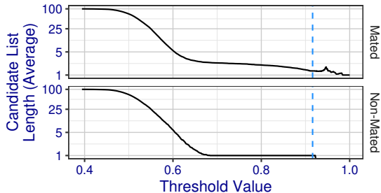
The similarity score indicated in blue is the threshold at which Hisignimpl+0017 achieves 10% FPIR.
