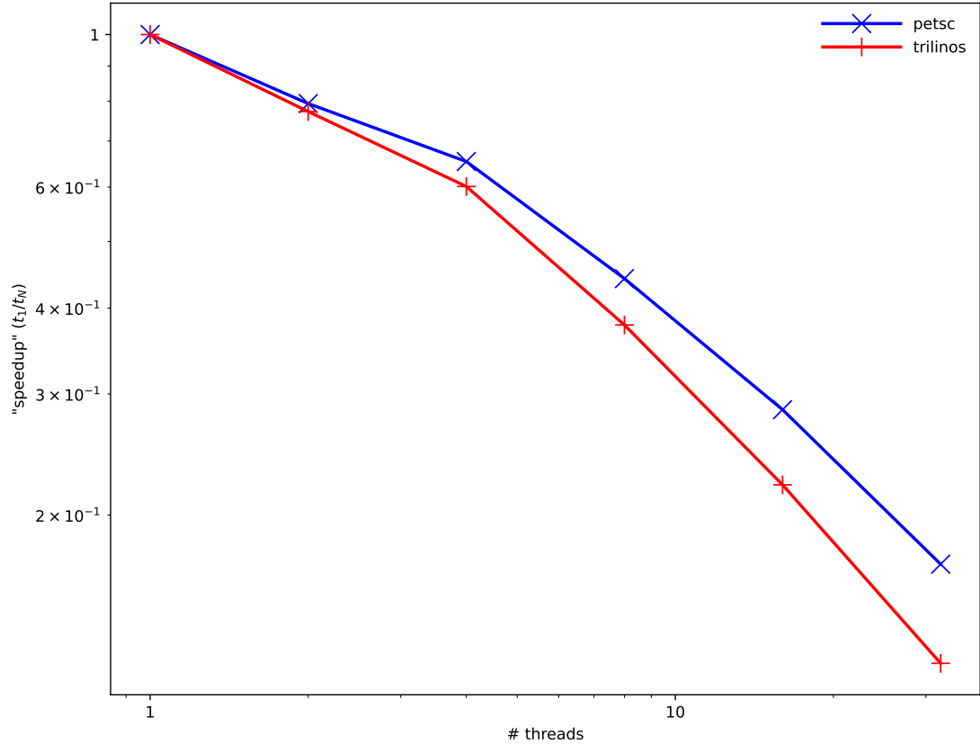
Fig. 1: Effect of having more OpenMP threads for each MPI rank Page 20, 1 .
