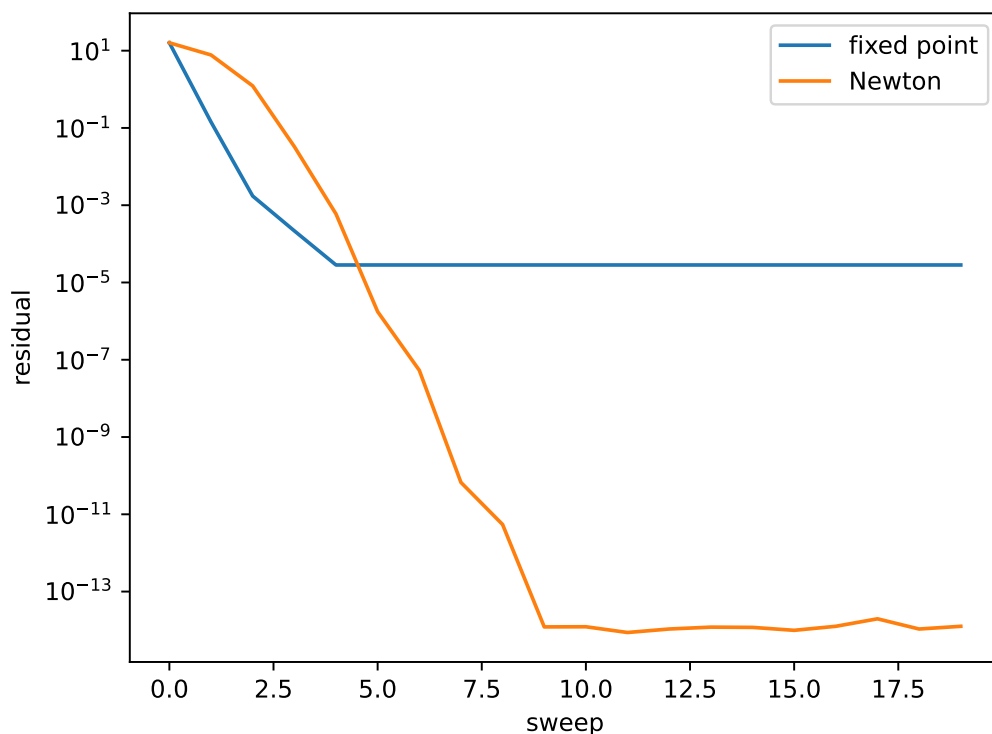
Fig. 4: Convergence of coupled non-linear diffusion problem evolved by fixed point and Newton iterations.
