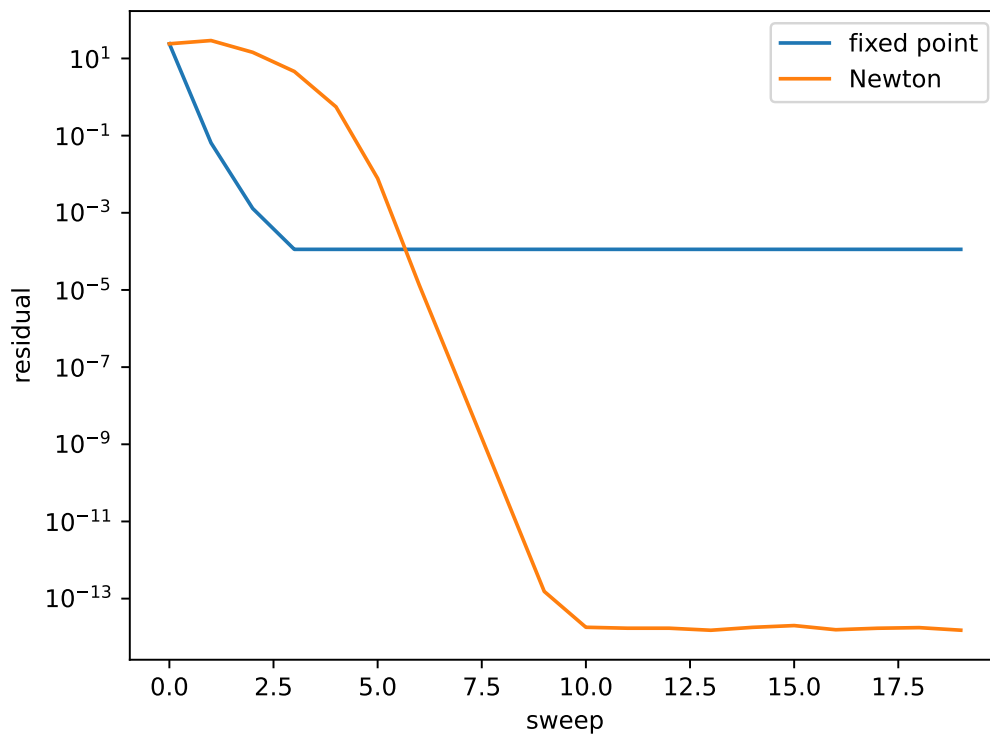
Fig. 2: Convergence of non-linear diffusion problem evolved by fixed point and Newton iterations.
