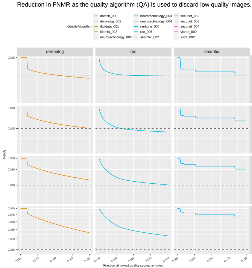
(c) Reduction in FNMR as the quality algorithm (QA) is used to discard low quality images.
