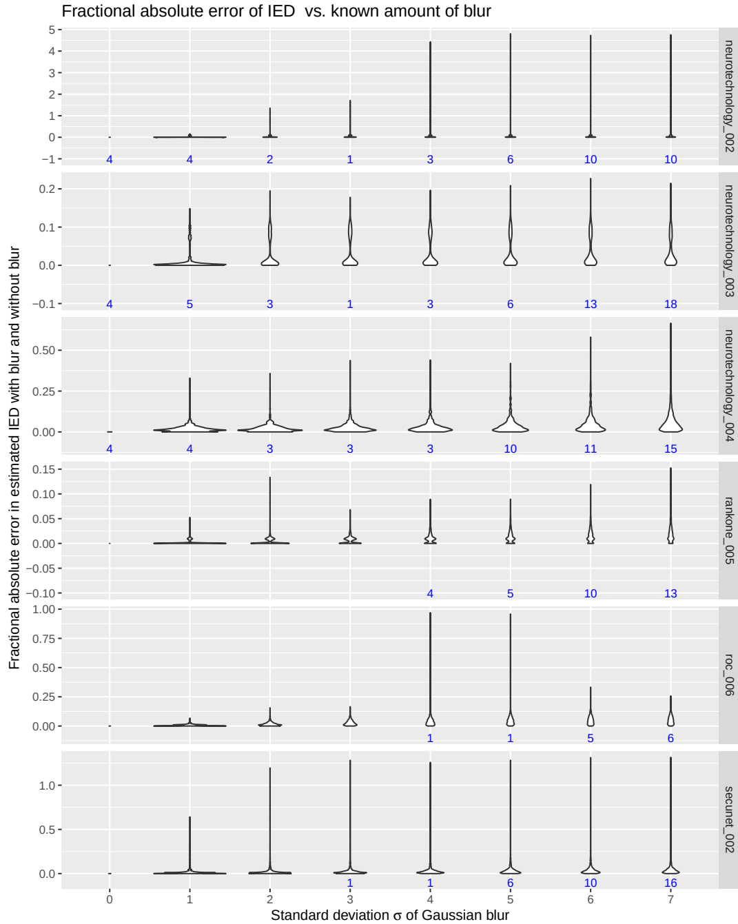
(b) Fractional absolute value of error in inter-eye distance estimates vs. \sigma parameter of Gaussian blur.
