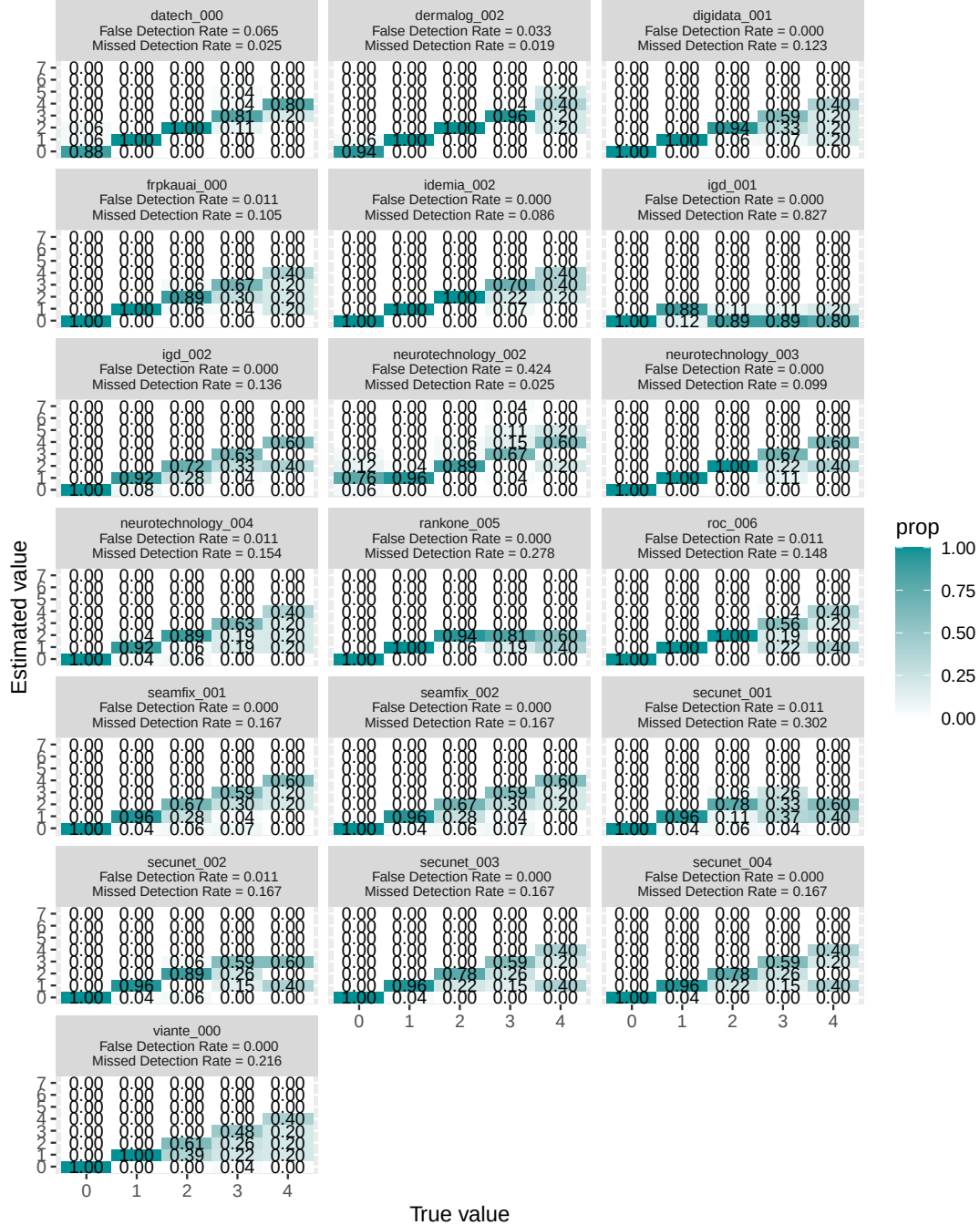
Fig. 2. Estimated number of faces vs. known number of faces. Perfect performance corresponds to zero on off-diagonal entries and 1 on each of the diagonal entries. Each column is normalized by the sum along that column, so that the numbers give estimates of the rate at which the software gives a false detection (above the diagonal), missed detection (below the diagonal), and correct detection (on the diagonal). Missed detections can occur because algorithms are configured to only detect faces larger than a certain size. The value at (x,y) is the proportion of images with known number of faces x and detected number of faces y . Missed detection rate is the number of missed faces divided by the total number of faces; false detection rate is the average number of wrong detections per image.
