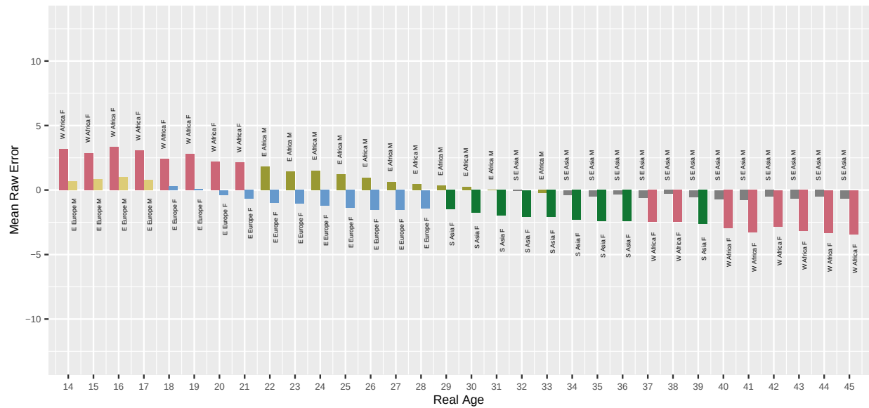
Fig. 16. For algorithm cognitec-000 applied to Application photos, the bar chart shows which demographic groups have the highest and lowest mean age estimation error, by age. Values closer to zero are better. Positive values are overestimate and negative values are underestimate.
