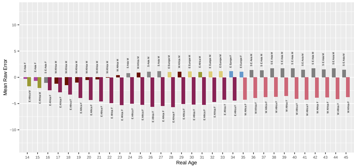
Fig. 82. For algorithm paravision-000 applied to Application photos, the bar chart shows which demographic groups have the highest and lowest mean age estimation error, by age. Values closer to zero are better. Positive values are overestimate and negative values are underestimate.
