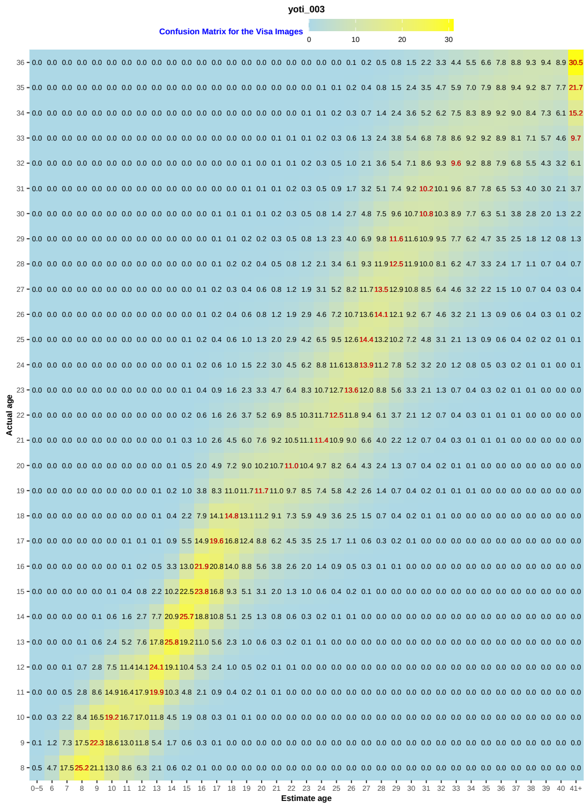
Fig. 180. Confusion matrix showing percentage of subjects aged 8 to 36 (rows) estimated as ages 0-5 to 41 and above (columns). Red values indicate the age most frequently estimated for each actual age.
