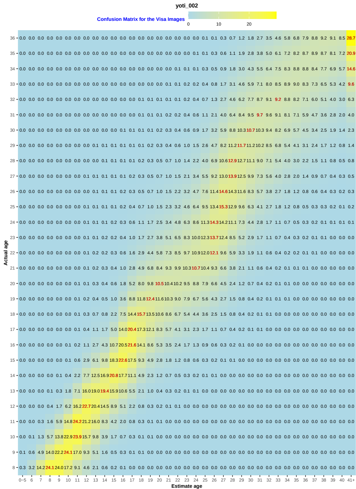
Fig. 179. Confusion matrix showing percentage of subjects aged 8 to 36 (rows) estimated as ages 0-5 to 41 and above (columns). Red values indicate the age most frequently estimated for each actual age.
