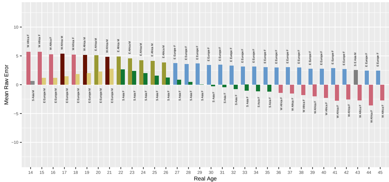
Fig. 101. For algorithm yoti-001 applied to Border photos, the bar chart shows which demographic groups have the highest and lowest mean age estimation error, by age. Values closer to zero are better. Positive values are overestimate and negative values are underestimate.
