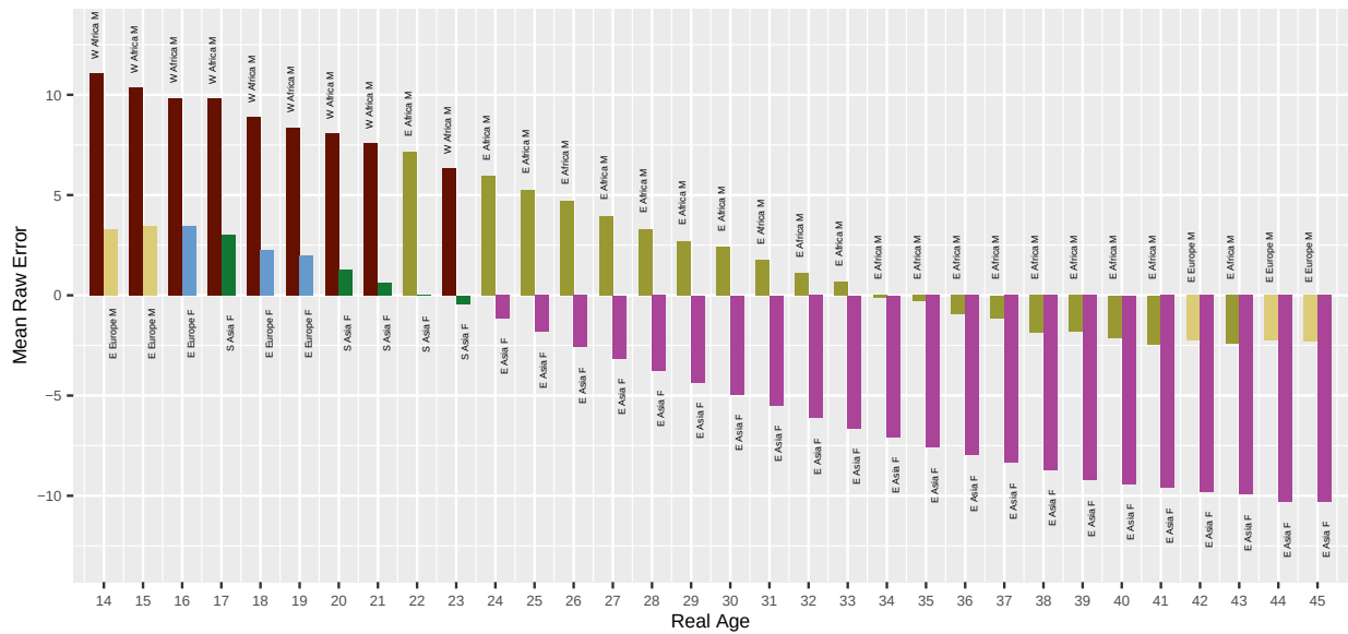
Fig. 68. For algorithm neurotechnology-000 applied to Application photos, the bar chart shows which demographic groups have the highest and lowest mean age estimation error, by age. Values closer to zero are better. Positive values are overestimate and negative values are underestimate.
