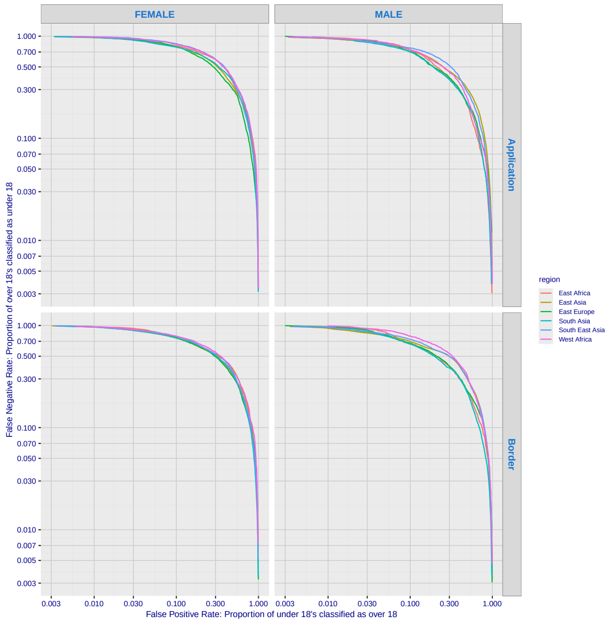
Fig. 239. For algorithm facehawk-001 the error tradeoff characteristics show tradeoff between false positive and negative rates as the score confidence threshold is swept across it's full range. FPR quantifies how often the underage are classified above 18; FNR quantifies how those over age are not.
