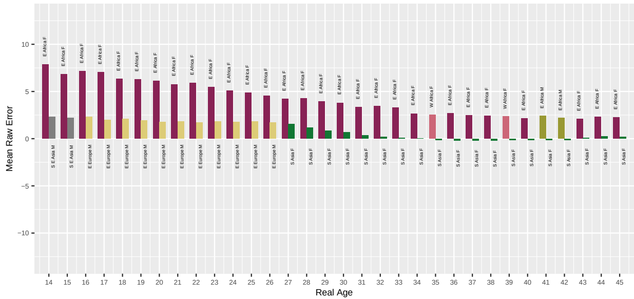
Fig. 81. For algorithm onfido-000 applied to Border photos, the bar chart shows which demographic groups have the highest and lowest mean age estimation error, by age. Values closer to zero are better. Positive values are overestimate and negative values are underestimate.
