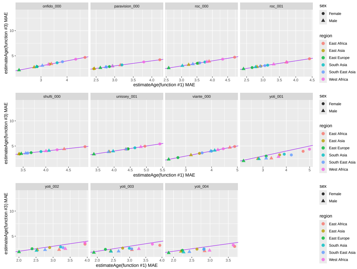
Fig. 133. In this figure, some algorithms show an improved MAE when given a prior image of known age to the second age estimate function. The x-axis represents the MAE for the first age estimation function, which returns the age estimate of a single image. In contrast, the y-axis represents the MAE for the second age estimation function, which returns the age estimate of an image when both the prior image and the known age of the same individual were provided.
