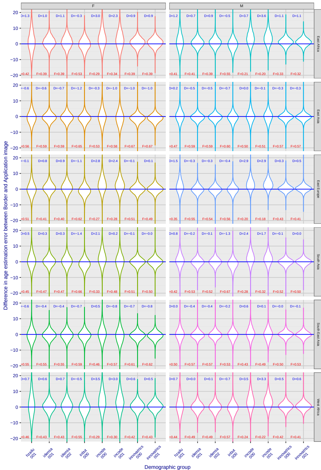
Fig. 112. Distribution of the pairwise age estimation error difference for Border and Application images. Positive values indicate larger error on Border images.
