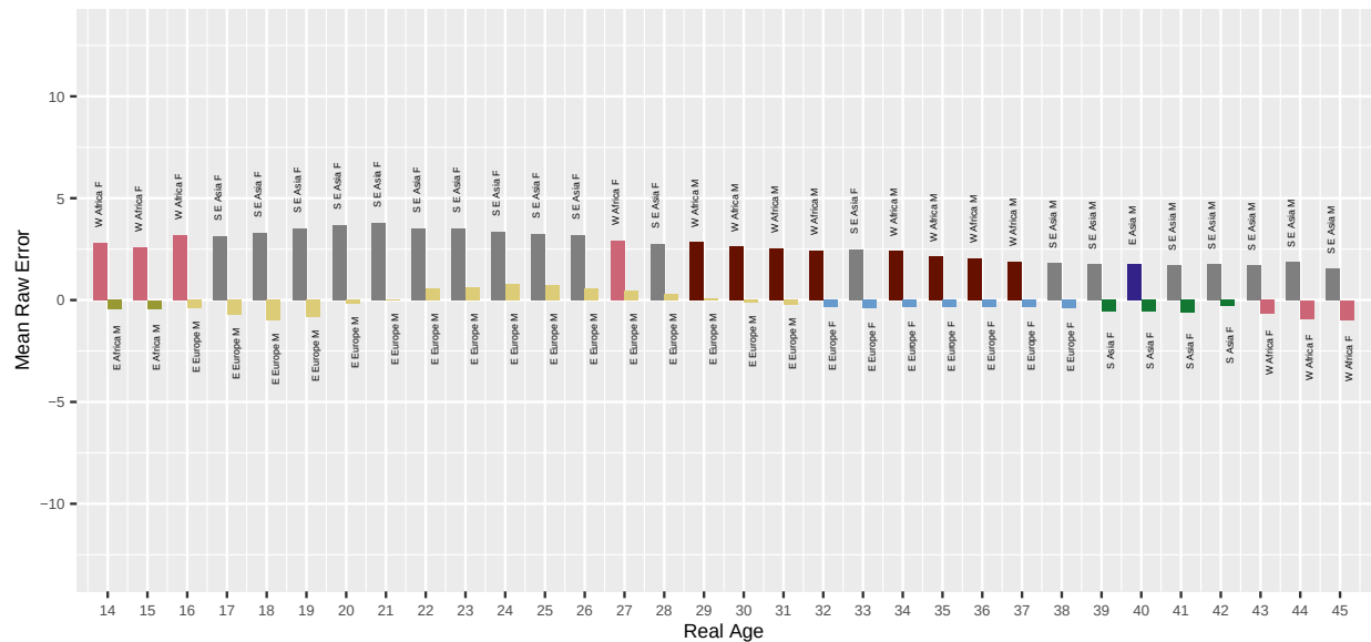
Fig. 102. For algorithm yoti-002 applied to Application photos, the bar chart shows which demographic groups have the highest and lowest mean age estimation error, by age. Values closer to zero are better. Positive values are overestimate and negative values are underestimate.
