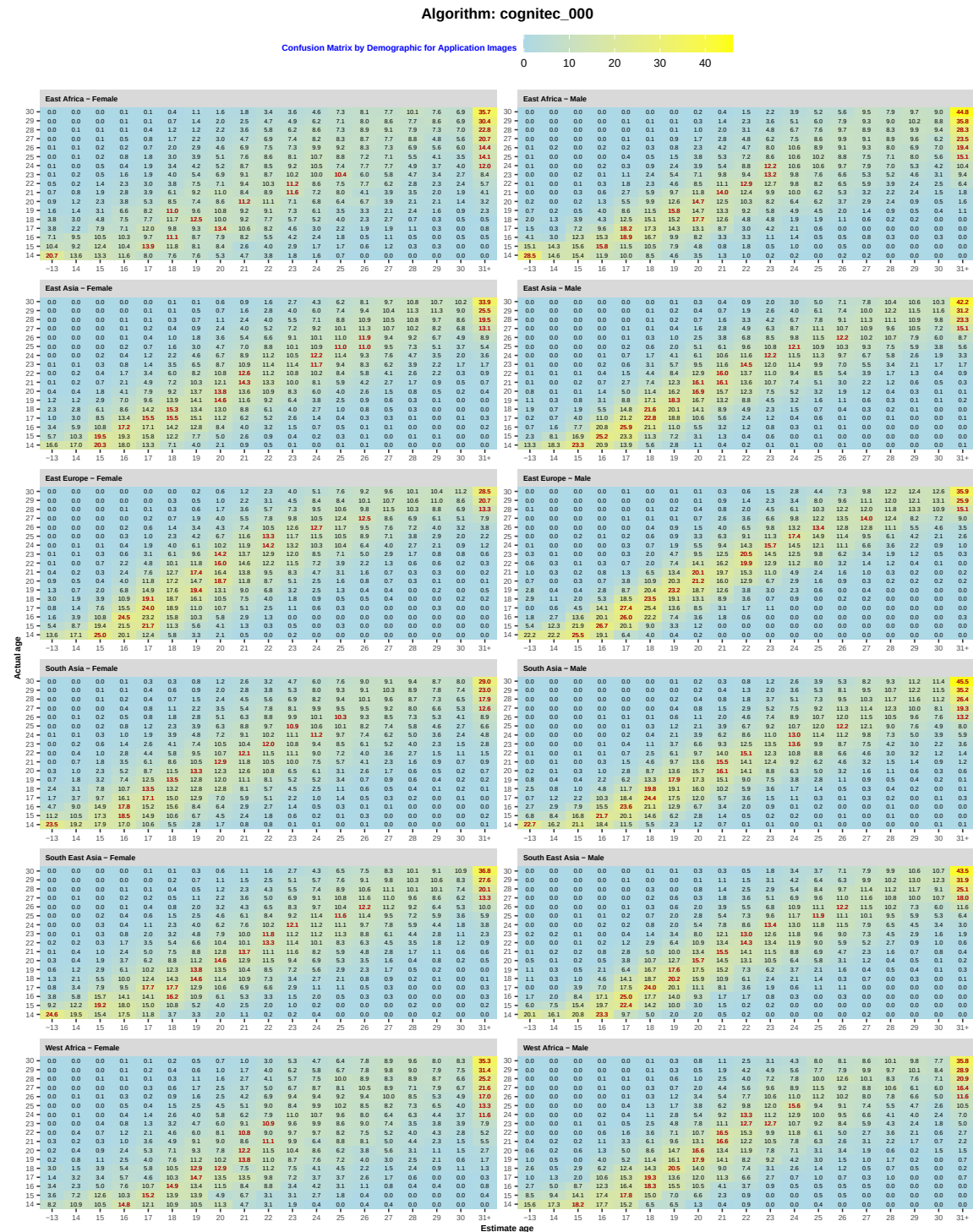
Fig. 185. Confusion matrices showing the percentage of subjects of true age (rows) estimated as ages ranging from 13 and below to 31 and above (columns -13 to 31+), broken down by 12 demographic groups (region and sex), for application images. Red values indicate the age most frequently estimated for each actual age.
