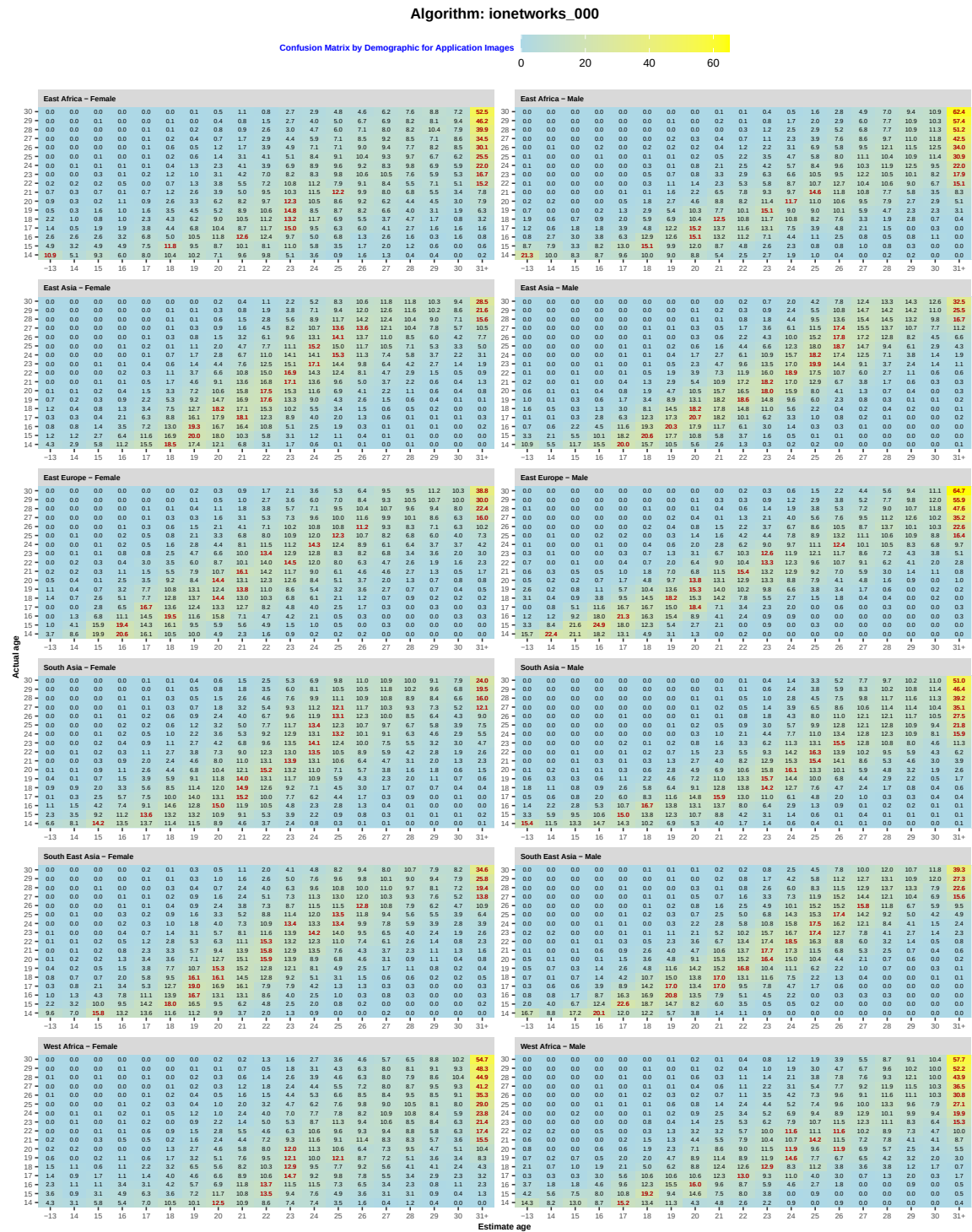
Fig. 209. Confusion matrices showing the percentage of subjects of true age (rows) estimated as ages ranging from 13 and below to 31 and above (columns -13 to 31+), broken down by 12 demographic groups (region and sex), for application images. Red values indicate the age most frequently estimated for each actual age.
