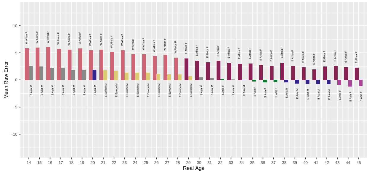
Fig. 66. For algorithm jumio-000 applied to Application photos, the bar chart shows which demographic groups have the highest and lowest mean age estimation error, by age. Values closer to zero are better. Positive values are overestimate and negative values are underestimate.
