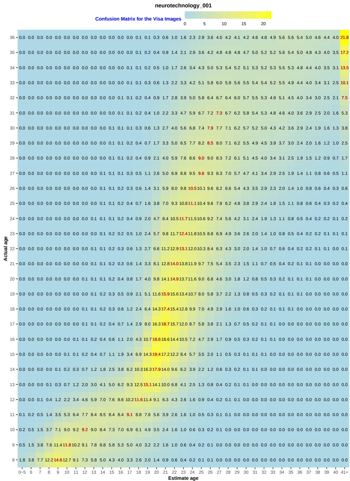
Fig. 163. Confusion matrix showing percentage of subjects aged 8 to 36 (rows) estimated as ages 0-5 to 41 and above (columns). Red values indicate the age most frequently estimated for each actual age.
