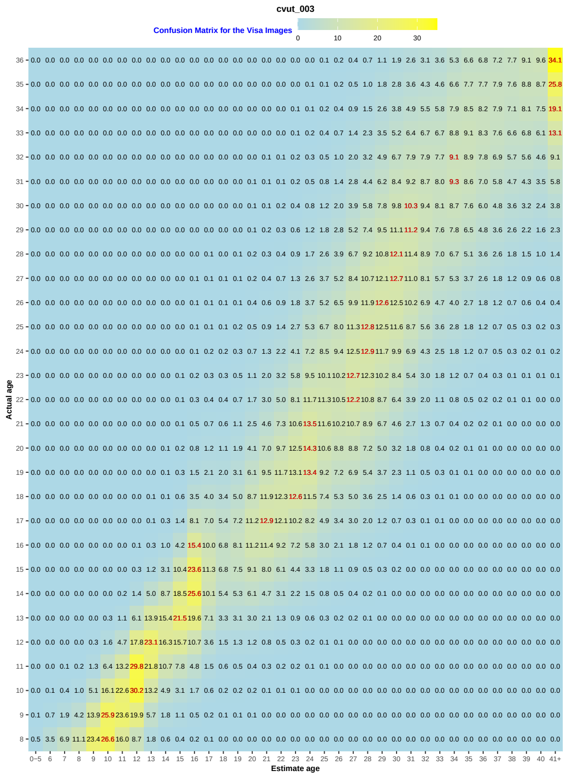
Fig. 140. Confusion matrix showing percentage of subjects aged 8 to 36 (rows) estimated as ages 0-5 to 41 and above (columns). Red values indicate the age most frequently estimated for each actual age.
