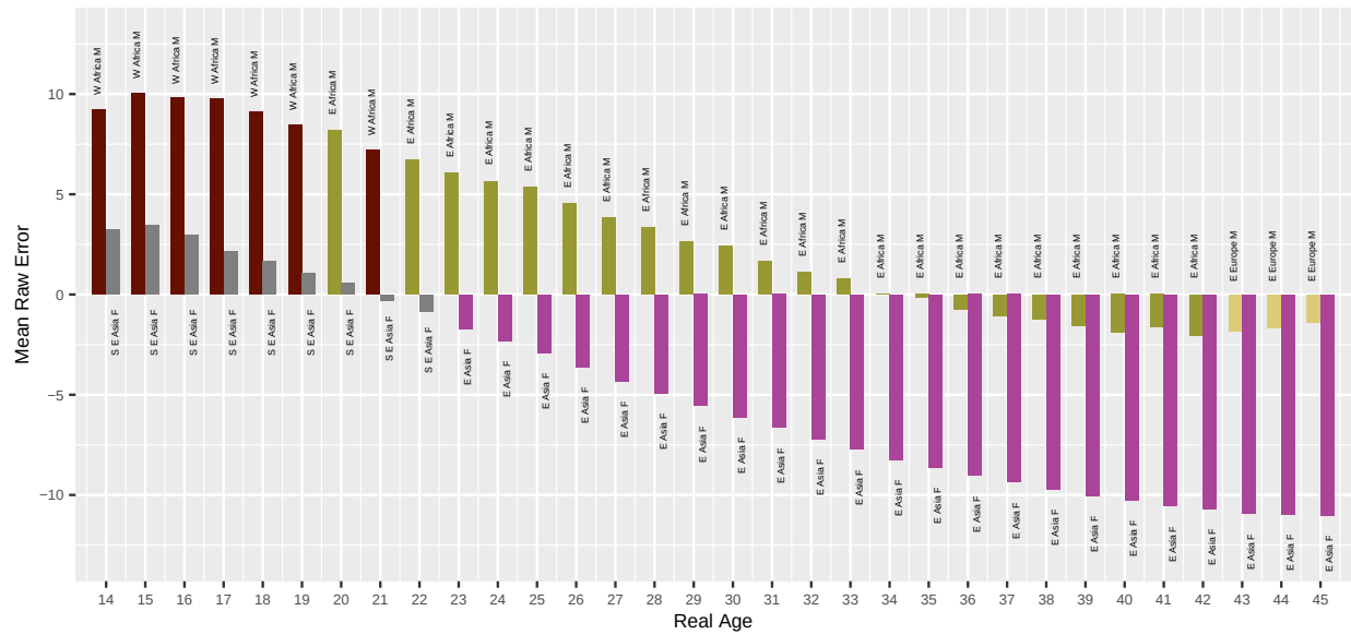
Fig. 69. For algorithm neurotechnology-000 applied to Border photos, the bar chart shows which demographic groups have the highest and lowest mean age estimation error, by age. Values closer to zero are better. Positive values are overestimate and negative values are underestimate.
