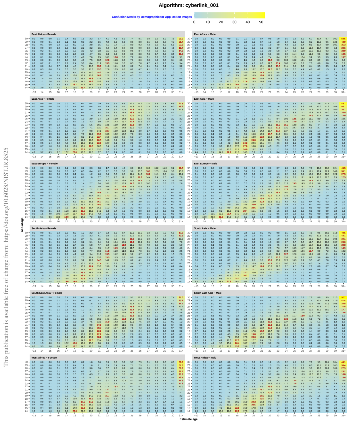
Fig. 191. Confusion matrices showing the percentage of subjects of true age (rows) estimated as ages ranging from 13 and below to 31 and above (columns -13 to 31+), broken down by 12 demographic groups (region and sex), for application images. Red values indicate the age most frequently estimated for each actual age.
