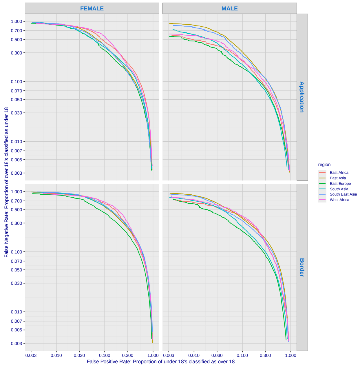
Fig. 233. For algorithm bynn-000 the error tradeoff characteristics show tradeoff between false positive and negative rates as the score confidence threshold is swept across it's full range. FPR quantifies how often the underage are classified above 18; FNR quantifies how those over age are not.
