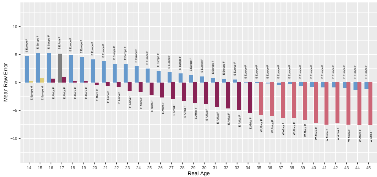
Fig. 32. For algorithm dermalog-002 applied to Application photos, the bar chart shows which demographic groups have the highest and lowest mean age estimation error, by age. Values closer to zero are better. Positive values are overestimate and negative values are underestimate.
