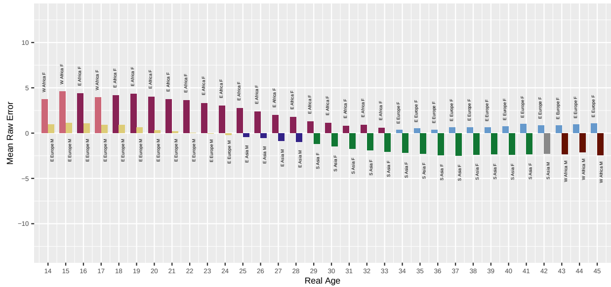
Fig. 75. For algorithm regula-000 applied to Border photos, the bar chart shows which demographic groups have the highest and lowest mean age estimation error, by age. Values closer to zero are better. Positive values are overestimate and negative values are underestimate.
