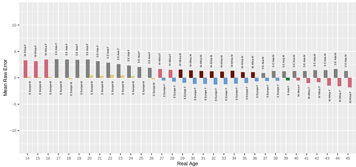
Fig. 94. For algorithm yoti-004 applied to Application photos, the bar chart shows which demographic groups have the highest and lowest mean age estimation error, by age. Values closer to zero are better. Positive values are overestimate and negative values are underestimate.
