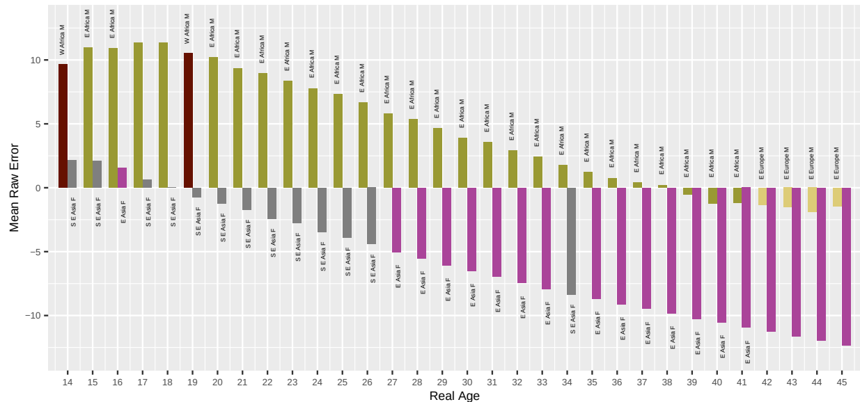
Fig. 97. For algorithm youverse-000 applied to Border photos, the bar chart shows which demographic groups have the highest and lowest mean age estimation error, by age. Values closer to zero are better. Positive values are overestimate and negative values are underestimate.
