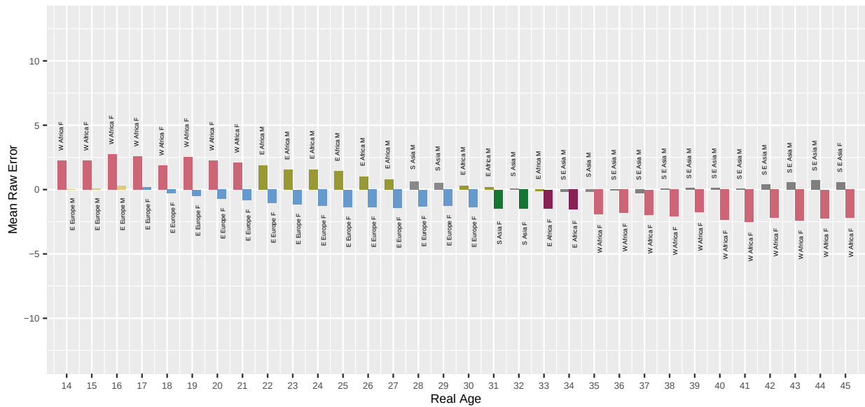
Fig. 14. For algorithm cognitec-001 applied to Application photos, the bar chart shows which demographic groups have the highest and lowest mean age estimation error, by age. Values closer to zero are better. Positive values are overestimate and negative values are underestimate.
