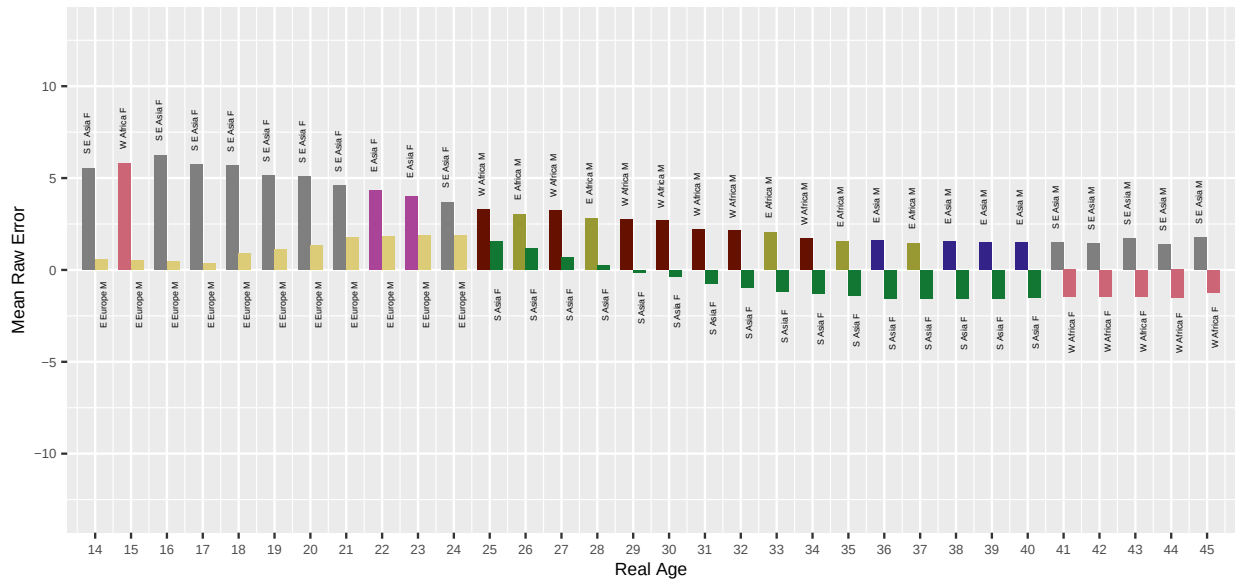
Fig. 93. For algorithm yoti-003 applied to Border photos, the bar chart shows which demographic groups have the highest and lowest mean age estimation error, by age. Values closer to zero are better. Positive values are overestimate and negative values are underestimate.
