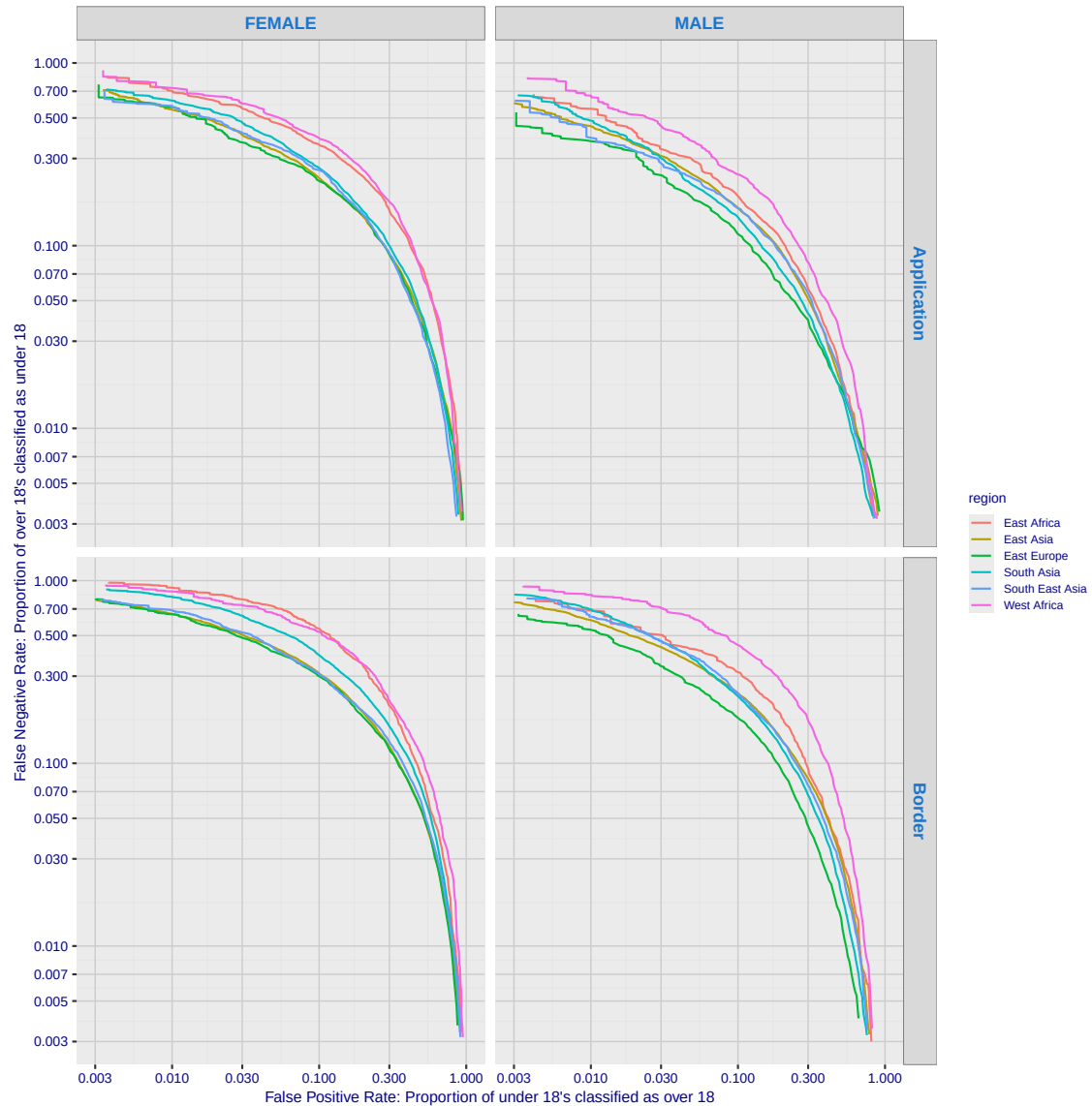
Fig. 118. For algorithm cognitec-000 the error tradeoff characteristics show tradeoff between false positive and negative rates as the score confidence threshold is swept across it's full range. FPR quantifies how often the underage are classified above 18; FNR quantifies how those over age are not.
