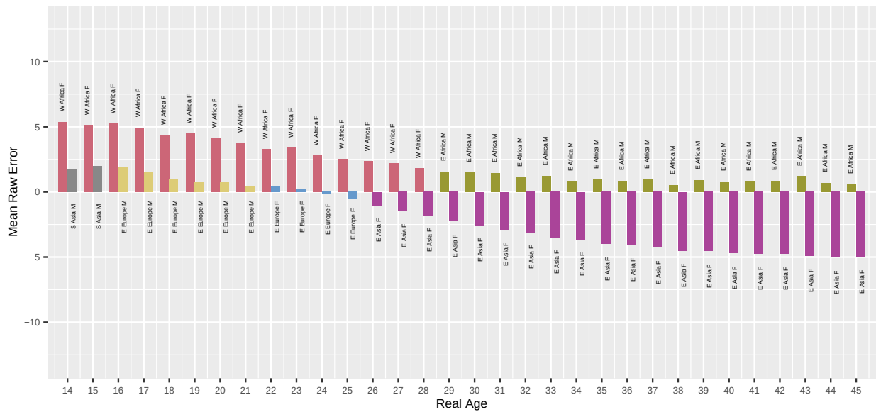
Fig. 64. For algorithm nominder-001 applied to Application photos, the bar chart shows which demographic groups have the highest and lowest mean age estimation error, by age. Values closer to zero are better. Positive values are overestimate and negative values are underestimate.
