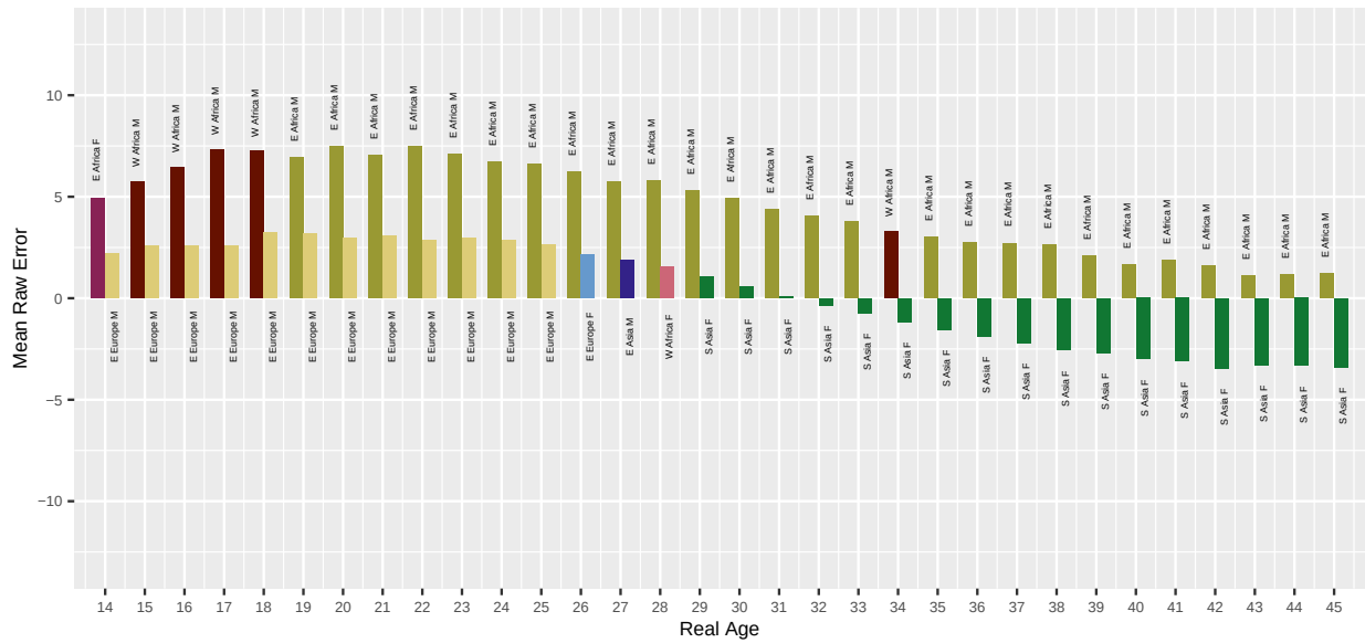
Fig. 31. For algorithm dermalog-001 applied to Border photos, the bar chart shows which demographic groups have the highest and lowest mean age estimation error, by age. Values closer to zero are better. Positive values are overestimate and negative values are underestimate.
