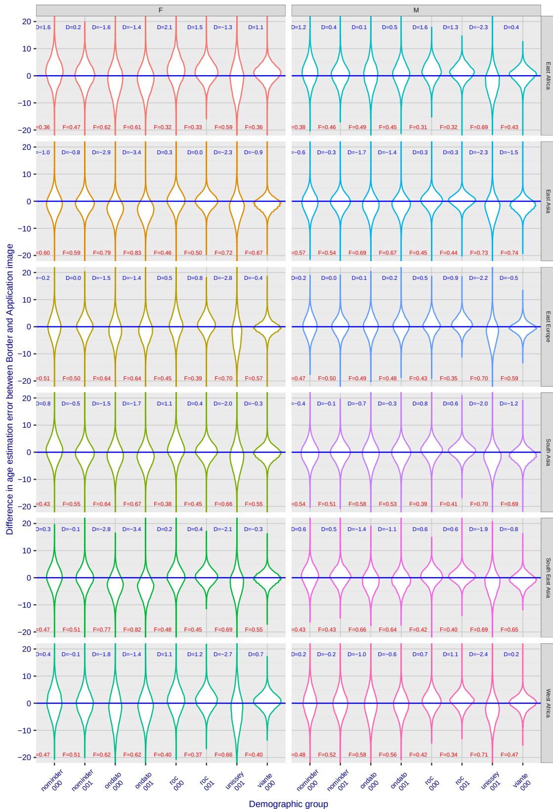
Fig. 66. Distribution of the pairwise age estimation error difference for Border and Application images. Positive values indicate larger error on Border images.
