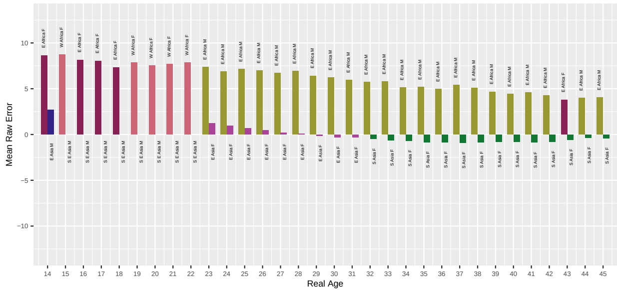
Fig. 35. For algorithm inc001 applied to Border photos, the bar chart shows which demographic groups have the highest and lowest mean age estimation error, by age. Values closer to zero are better. Positive values are overestimate and negative values are underestimate.
