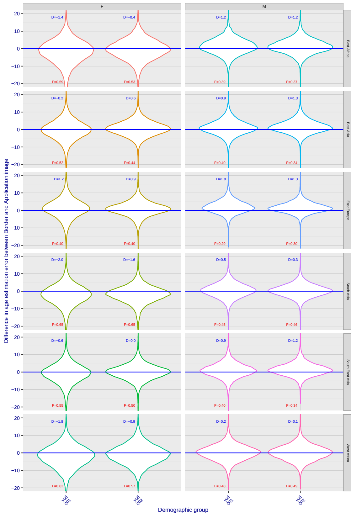
Fig. 67. Distribution of the pairwise age estimation error difference for Border and Application images. Positive values indicate larger error on Border images.
