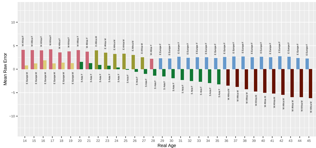
Fig. 56. For algorithm unissey-001 applied to Application photos, the bar chart shows which demographic groups have the highest and lowest mean age estimation error, by age. Values closer to zero are better. Positive values are overestimate and negative values are underestimate.
