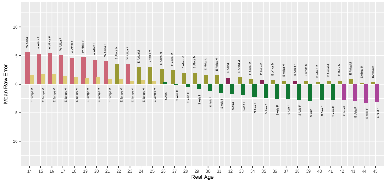
Fig. 50. For algorithm ondato-001 applied to Application photos, the bar chart shows which demographic groups have the highest and lowest mean age estimation error, by age. Values closer to zero are better. Positive values are overestimate and negative values are underestimate.
