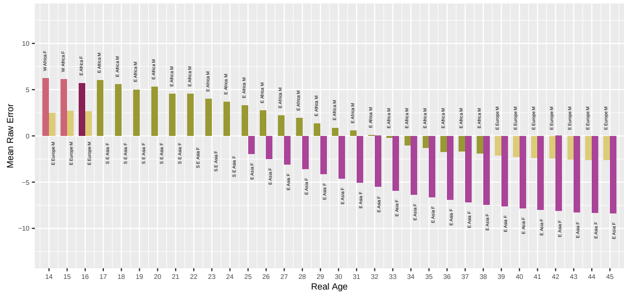
Fig. 51. For algorithm ondato-001 applied to Border photos, the bar chart shows which demographic groups have the highest and lowest mean age estimation error, by age. Values closer to zero are better. Positive values are overestimate and negative values are underestimate.
