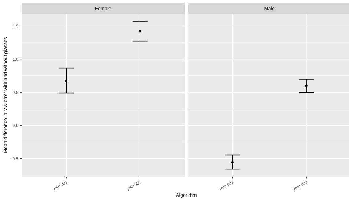
Fig. 75. Difference in age estimation error for border crossing subjects with and without eyeglasses.
