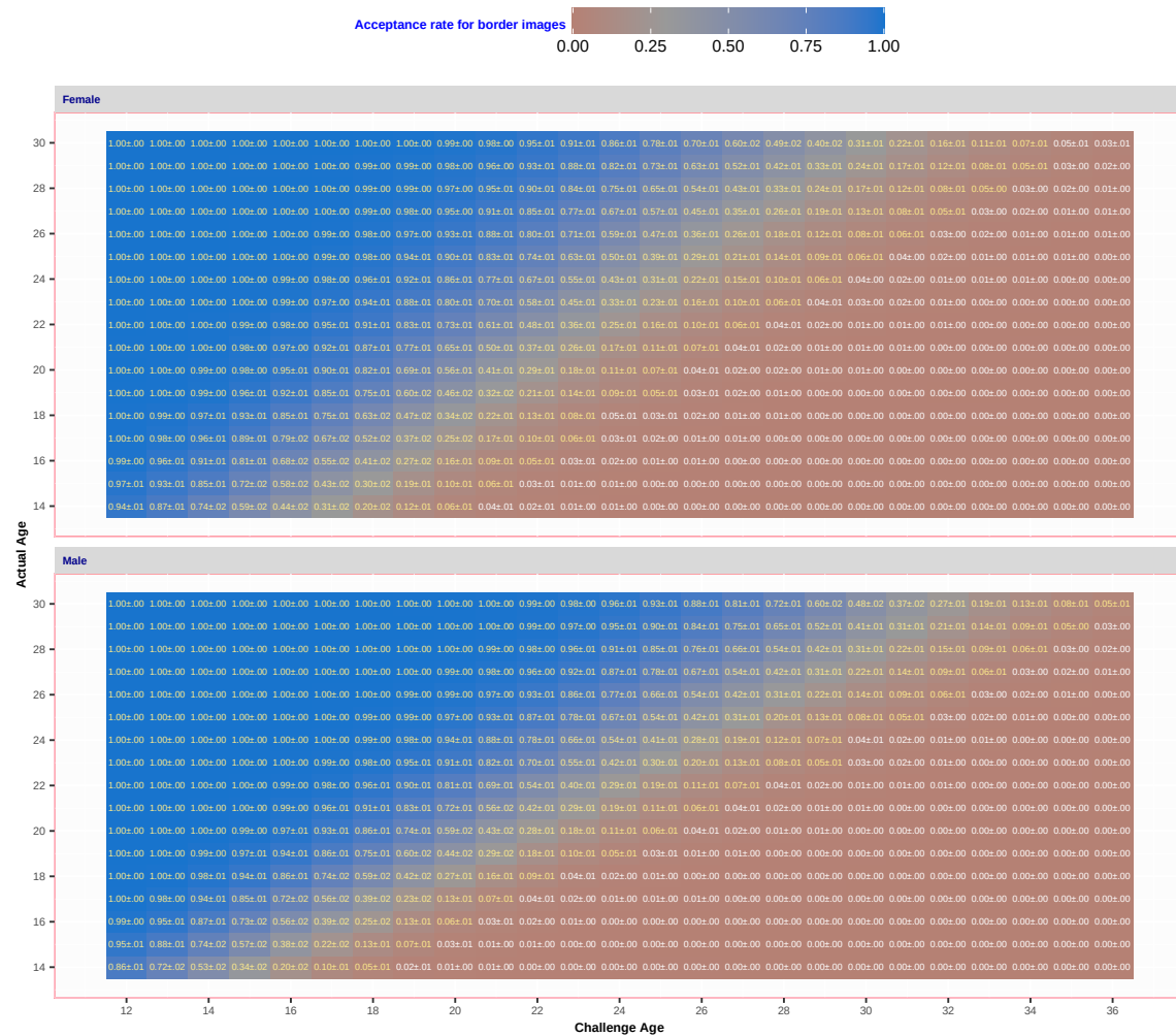
Fig. 80. For algorithm Idemia 001 applied border-crossing photos, the heatmap and text shows proportion of photos of the persons of an actual age are accepted at a particular challenge age.
