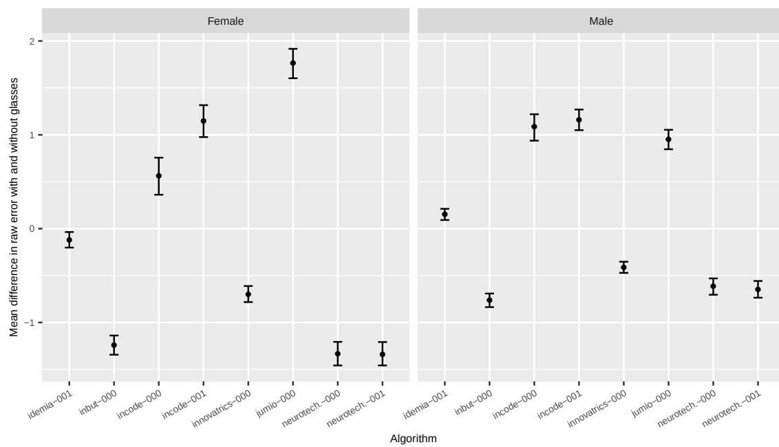
Fig. 73. Difference in age estimation error for border crossing subjects with and without eyeglasses.
