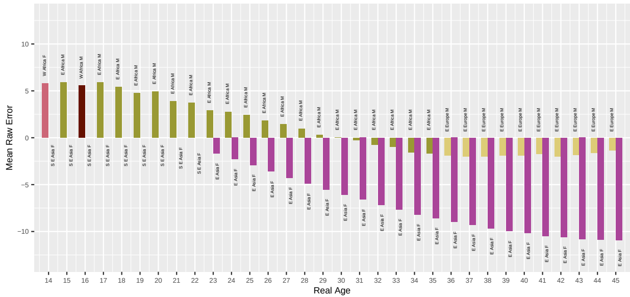
Fig. 43. For algorithm neurotechnology-001 applied to Border photos, the bar chart shows which demographic groups have the highest and lowest mean age estimation error, by age. Values closer to zero are better. Positive values are overestimate and negative values are underestimate.
