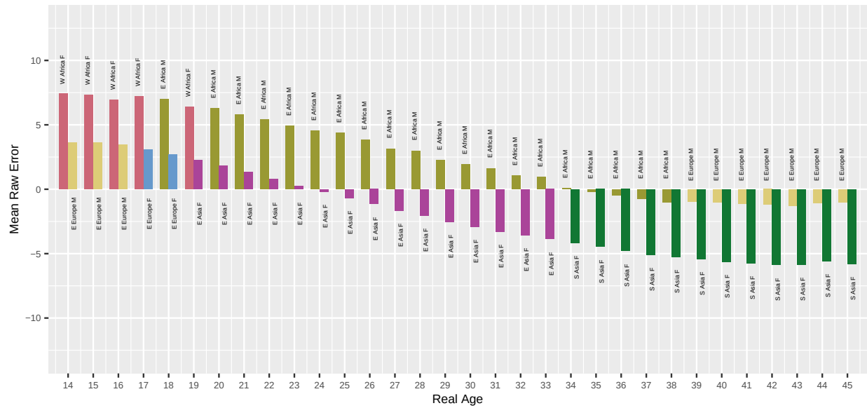
Fig. 45. For algorithm nominder-000 applied to Border photos, the bar chart shows which demographic groups have the highest and lowest mean age estimation error, by age. Values closer to zero are better. Positive values are overestimate and negative values are underestimate.
