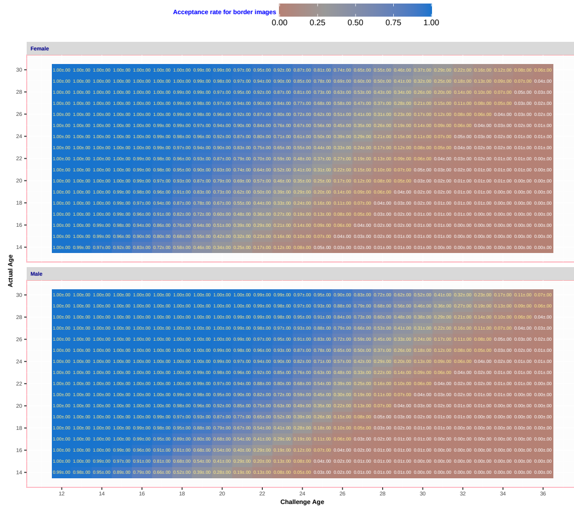
Fig. 84. For algorithm Nominder 000 applied border-crossing photos, the heatmap and text shows proportion of photos of the persons of an actual age are accepted at a particular challenge age.
