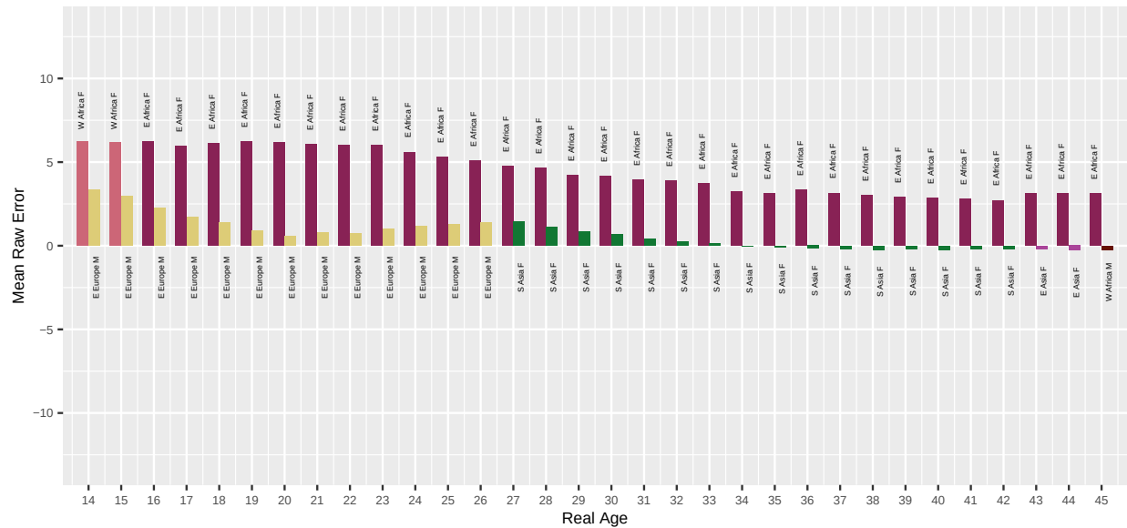
Fig. 55. For algorithm roc-001 applied to Border photos, the bar chart shows which demographic groups have the highest and lowest mean age estimation error, by age. Values closer to zero are better. Positive values are overestimate and negative values are underestimate.
