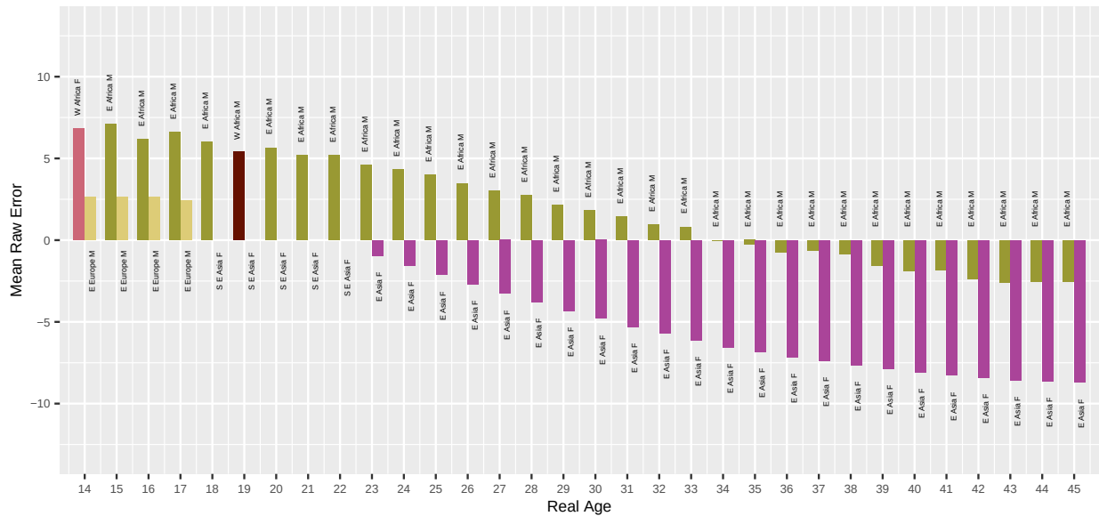
Fig. 49. For algorithm ondato-000 applied to Border photos, the bar chart shows which demographic groups have the highest and lowest mean age estimation error, by age. Values closer to zero are better. Positive values are overestimate and negative values are underestimate.
