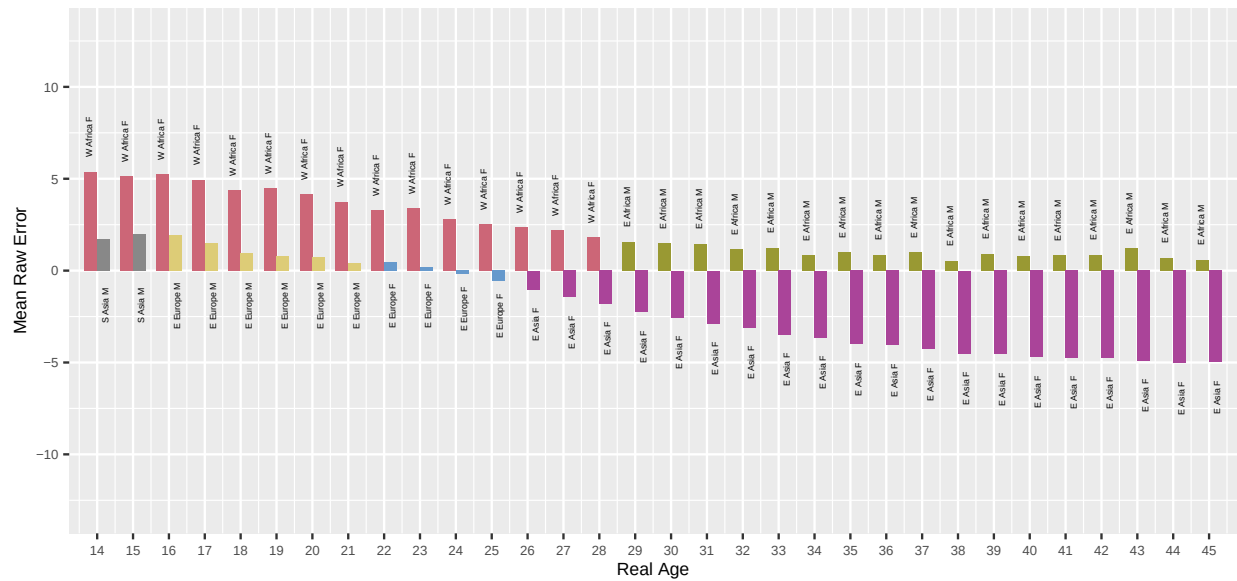
Fig. 46. For algorithm nominder-001 applied to Application photos, the bar chart shows which demographic groups have the highest and lowest mean age estimation error, by age. Values closer to zero are better. Positive values are overestimate and negative values are underestimate.
