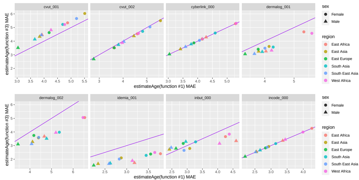
Fig. 76. In this figure, some algorithms show an improved MAE when given a prior image of known age to the second age estimate function. The x-axis represents the MAE for the first age estimation function, which returns the age estimate of a single image. In contrast, the y-axis represents the MAE for the second age estimation function, which returns the age estimate of an image when both the prior image and the known age of the same individual were provided.
