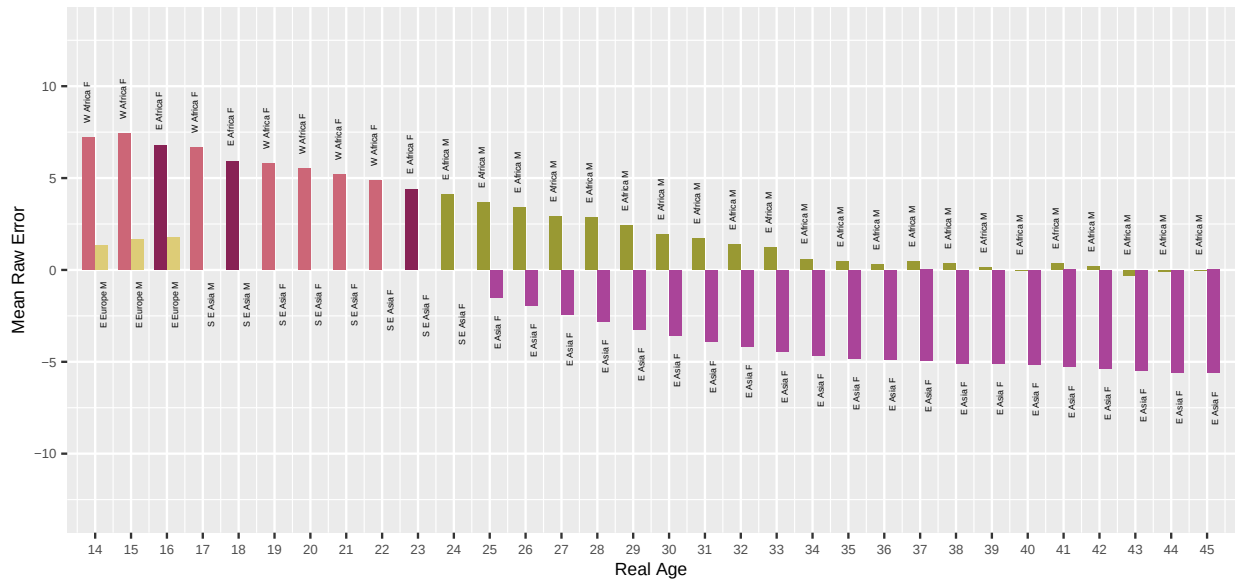
Fig. 37. For algorithm innovatrics-000 applied to Border photos, the bar chart shows which demographic groups have the highest and lowest mean age estimation error, by age. Values closer to zero are better. Positive values are overestimate and negative values are underestimate.
