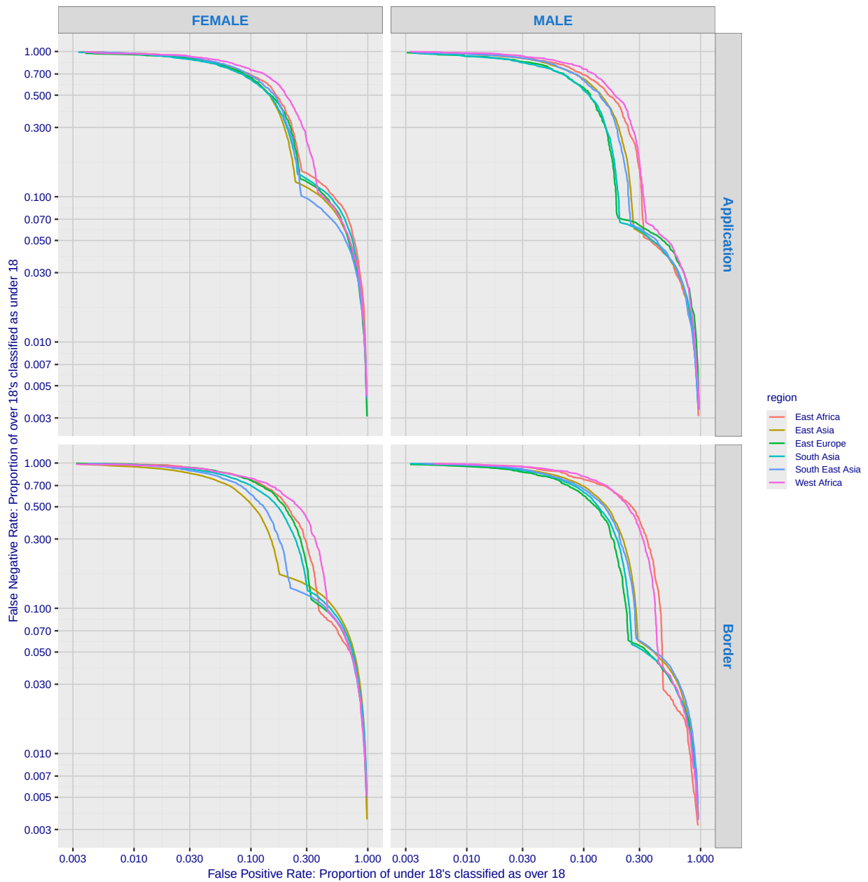
Fig. 111. For algorithm idemia-002 the error tradeoff characteristics show tradeoff between false positive and negative rates as the score confidence threshold is swept across it's full range. FPR quantifies how often the underage are classified above 18; FNR quantifies how those over age are not.
