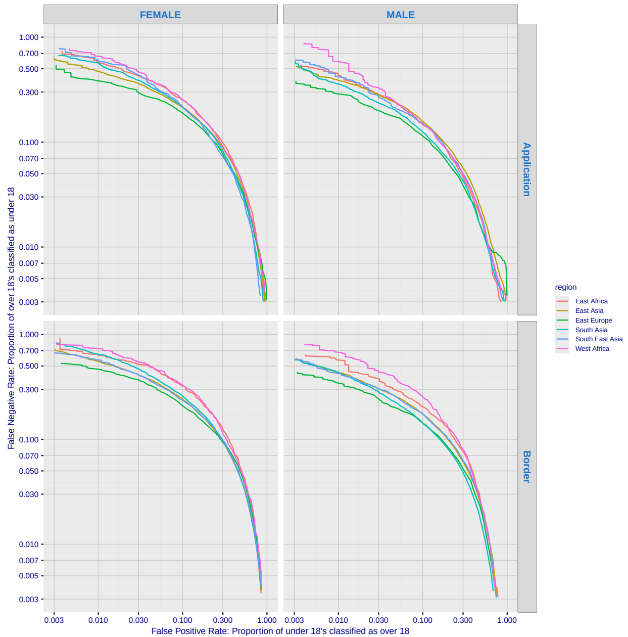
Fig. 114. For algorithm roc-002 the error tradeoff characteristics show tradeoff between false positive and negative rates as the score confidence threshold is swept across it's full range. FPR quantifies how often the underage are classified above 18; FNR quantifies how those over age are not.
