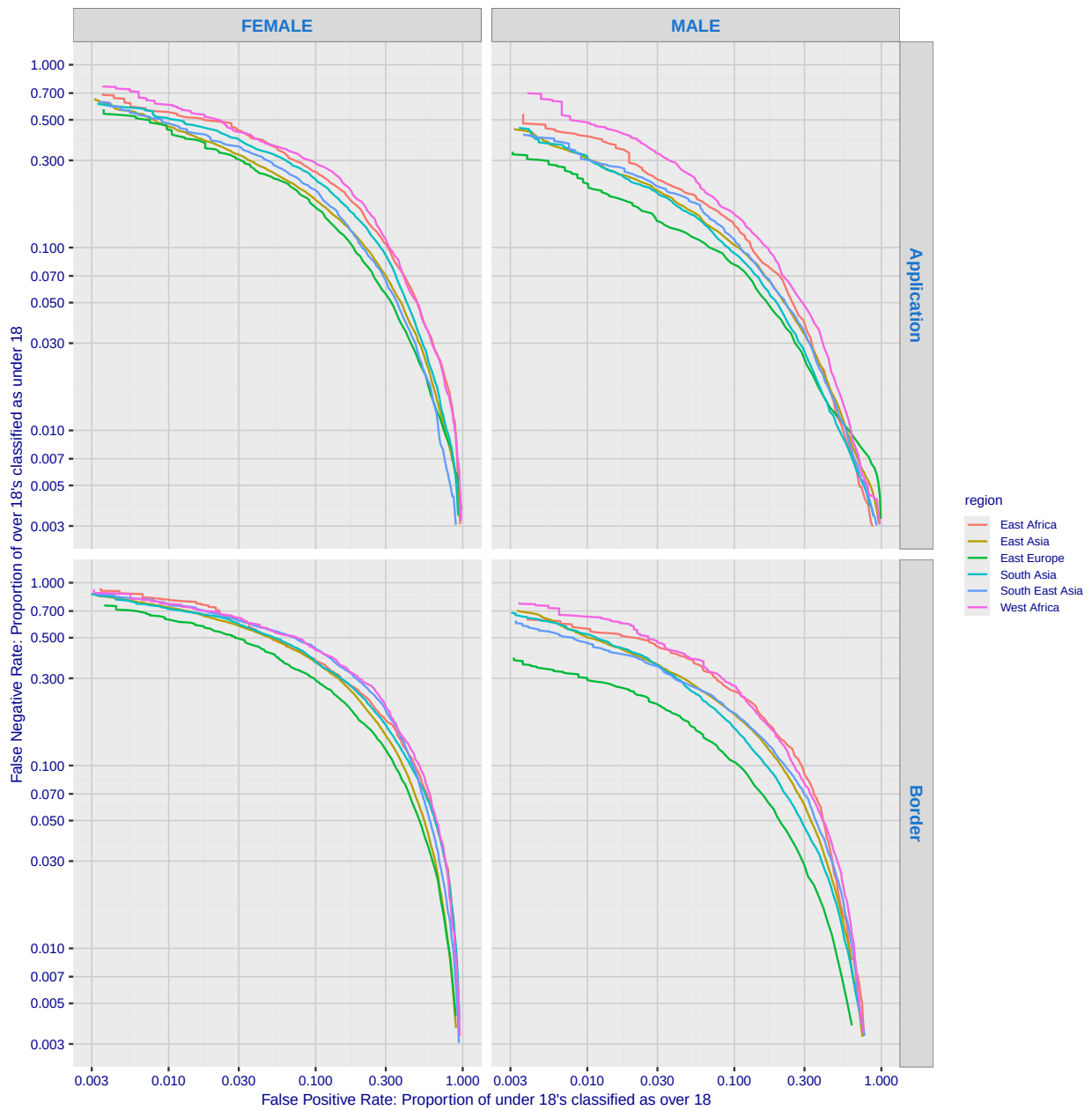
Fig. 117. For algorithm yoti-004 the error tradeoff characteristics show tradeoff between false positive and negative rates as the score confidence threshold is swept across it's full range. FPR quantifies how often the underage are classified above 18; FNR quantifies how those over age are not.
