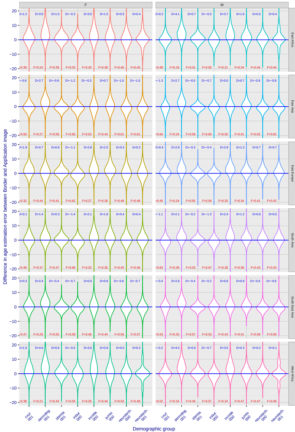
Fig. 37. Distribution of the pairwise age estimation error difference for Border and Application images. Positive values indicate larger error on Border images.
