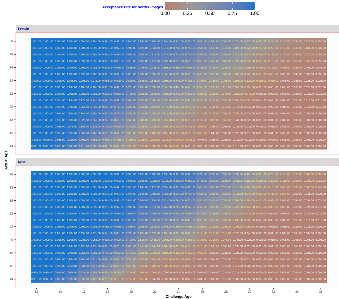
Fig. 49. For algorithm Unissey 001 applied border-crossing photos, the heatmap and text shows proportion of photos of the persons of an actual age are accepted at a particular challenge age.
