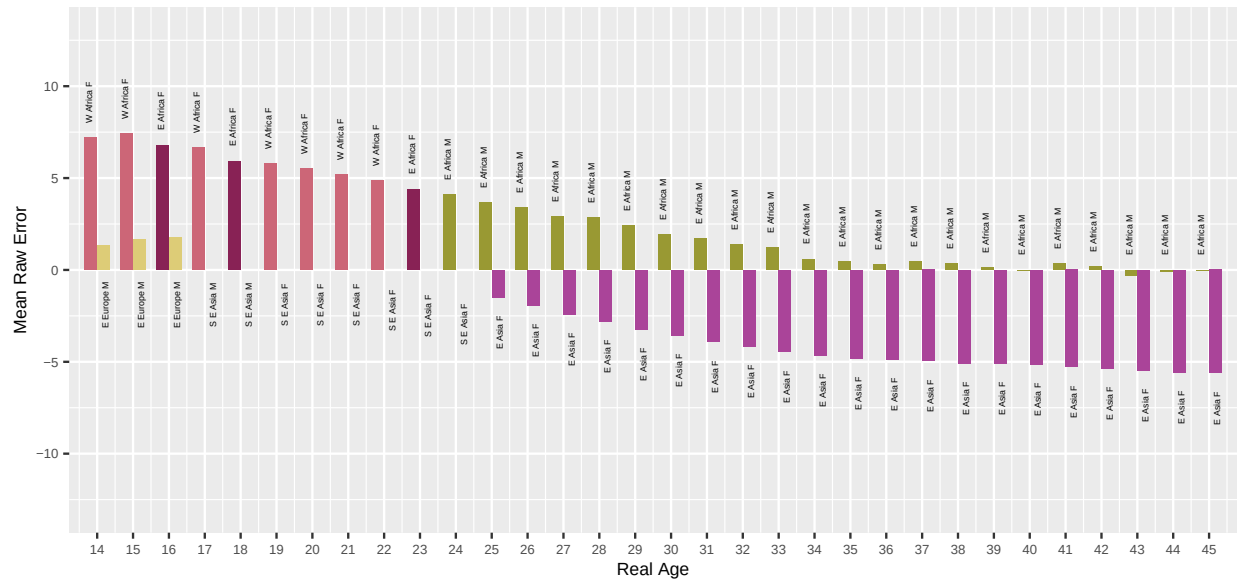
Fig. 27. For algorithm innovatrics-000 applied to Border photos, the bar chart shows which demographic groups have the highest and lowest mean age estimation error, by age. Values closer to zero are better. Positive values are overestimate and negative values are underestimate.
