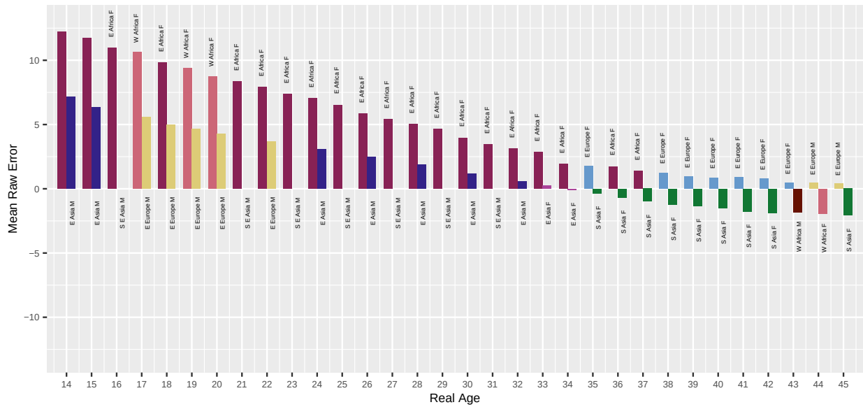
Fig. 29. For algorithm jumio-000 applied to Border photos, the bar chart shows which demographic groups have the highest and lowest mean age estimation error, by age. Values closer to zero are better. Positive values are overestimate and negative values are underestimate.
