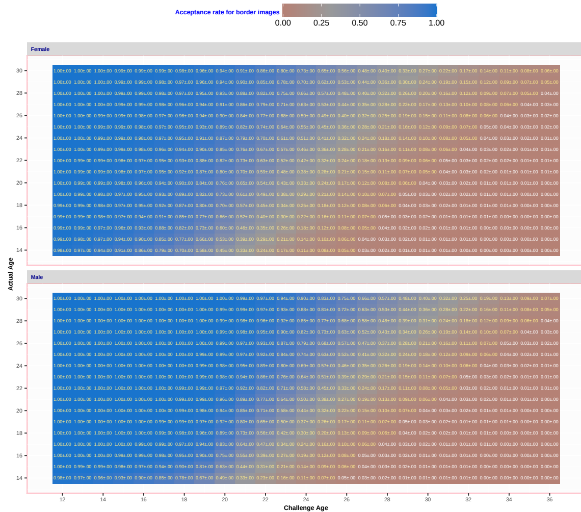
Fig. 61. For algorithm Neurotechnology 000 applied border-crossing photos, the heatmap and text shows proportion of photos of the persons of an actual age are accepted at a particular challenge age.
