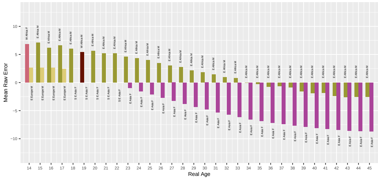
Fig. 39. For algorithm ondato-000 applied to Border photos, the bar chart shows which demographic groups have the highest and lowest mean age estimation error, by age. Values closer to zero are better. Positive values are overestimate and negative values are underestimate.
