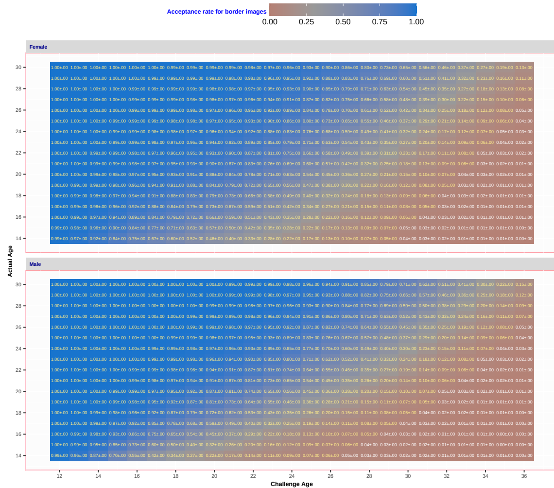
Fig. 58. For algorithm Dermalog 001 applied border-crossing photos, the heatmap and text shows proportion of photos of the persons of an actual age are accepted at a particular challenge age.
