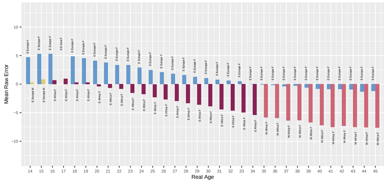
Fig. 18. For algorithm dermalog-002 applied to Application photos, the bar chart shows which demographic groups have the highest and lowest mean age estimation error, by age. Values closer to zero are better. Positive values are overestimate and negative values are underestimate.
