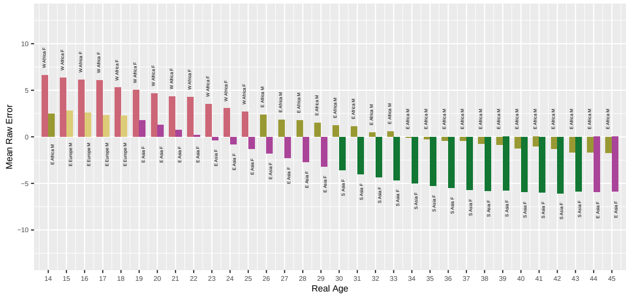
Fig. 37. For algorithm nominder-001 applied to Border photos, the bar chart shows which demographic groups have the highest and lowest mean age estimation error, by age. Values closer to zero are better. Positive values are overestimate and negative values are underestimate.
