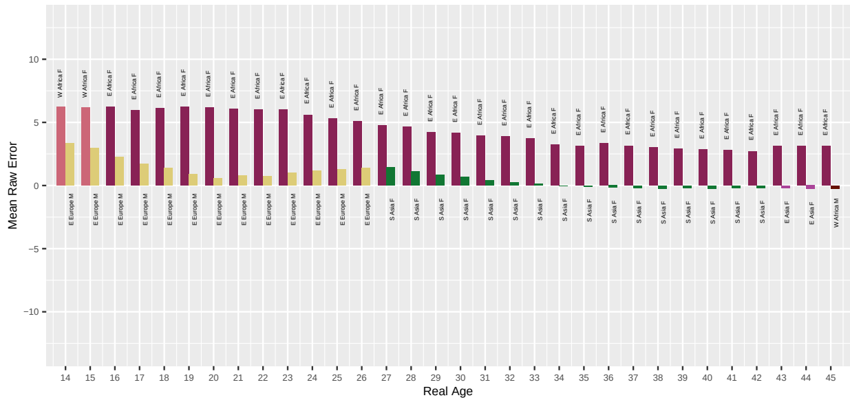
Fig. 43. For algorithm roc-001 applied to Border photos, the bar chart shows which demographic groups have the highest and lowest mean age estimation error, by age. Values closer to zero are better. Positive values are overestimate and negative values are underestimate.
