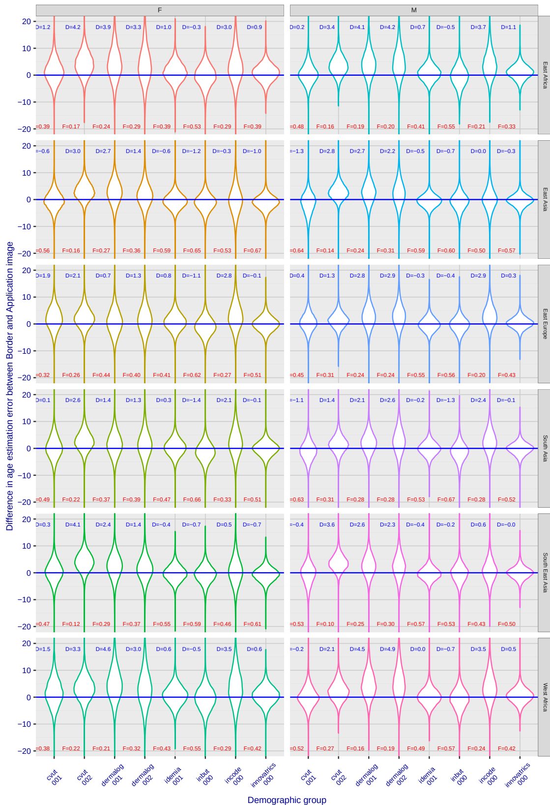
Fig. 52. Distribution of the pairwise age estimation error difference for Border and Application images. Positive values indicate larger error on Border images.
