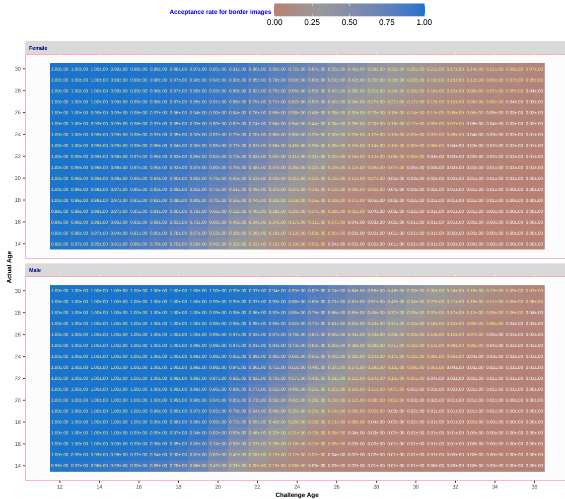
Fig. 62. For algorithm Neurotechnology 001 applied border-crossing photos, the heatmap and text shows proportion of photos of the persons of an actual age are accepted at a particular challenge age.
