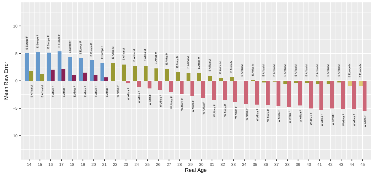
Fig. 16. For algorithm dermalog-001 applied to Application photos, the bar chart shows which demographic groups have the highest and lowest mean age estimation error, by age. Values closer to zero are better. Positive values are overestimate and negative values are underestimate.
