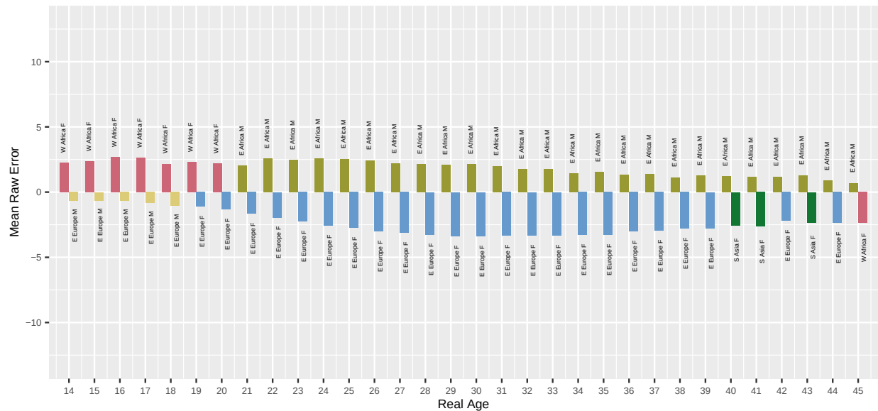
Fig. 20. For algorithm idemia-001 applied to Application photos, the bar chart shows which demographic groups have the highest and lowest mean age estimation error, by age. Values closer to zero are better. Positive values are overestimate and negative values are underestimate.
