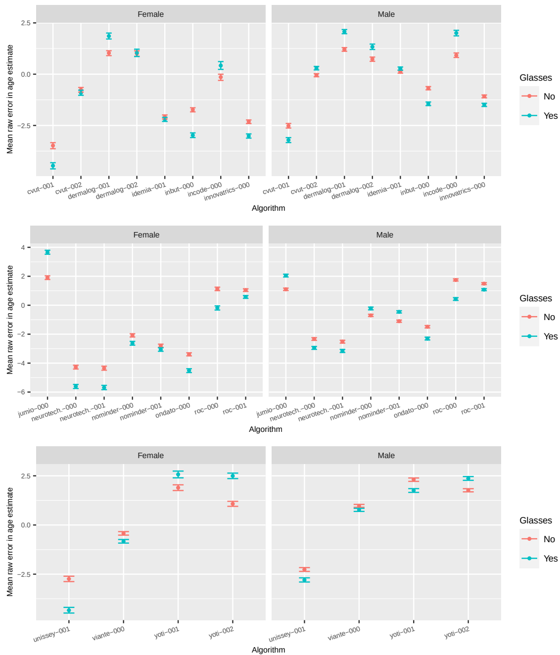
Fig. 55. Mean raw age estimation error for border crossing subjects for whom we have images with and without eyeglasses.
