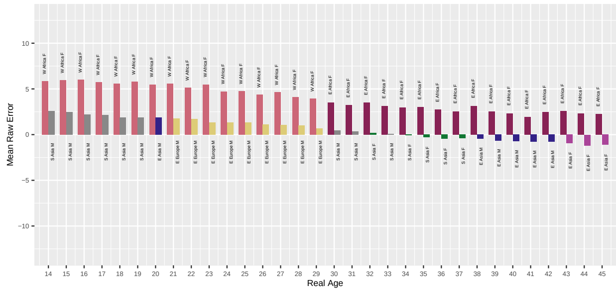
Fig. 28. For algorithm jumio-000 applied to Application photos, the bar chart shows which demographic groups have the highest and lowest mean age estimation error, by age. Values closer to zero are better. Positive values are overestimate and negative values are underestimate.
