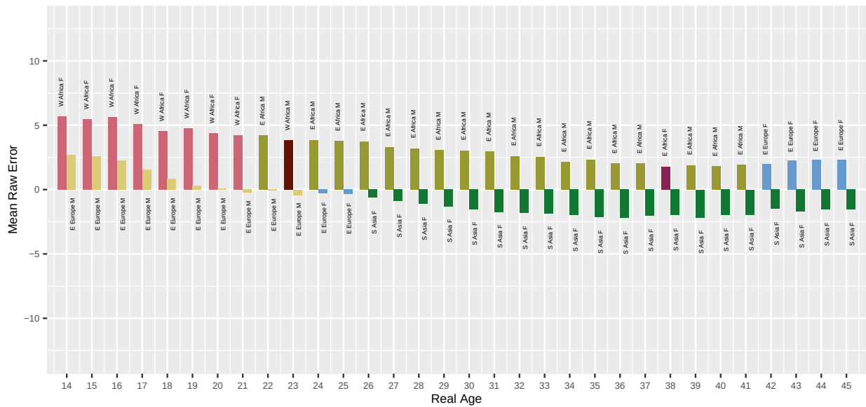
Fig. 40. For algorithm roc-000 applied to Application photos, the bar chart shows which demographic groups have the highest and lowest mean age estimation error, by age. Values closer to zero are better. Positive values are overestimate and negative values are underestimate.
