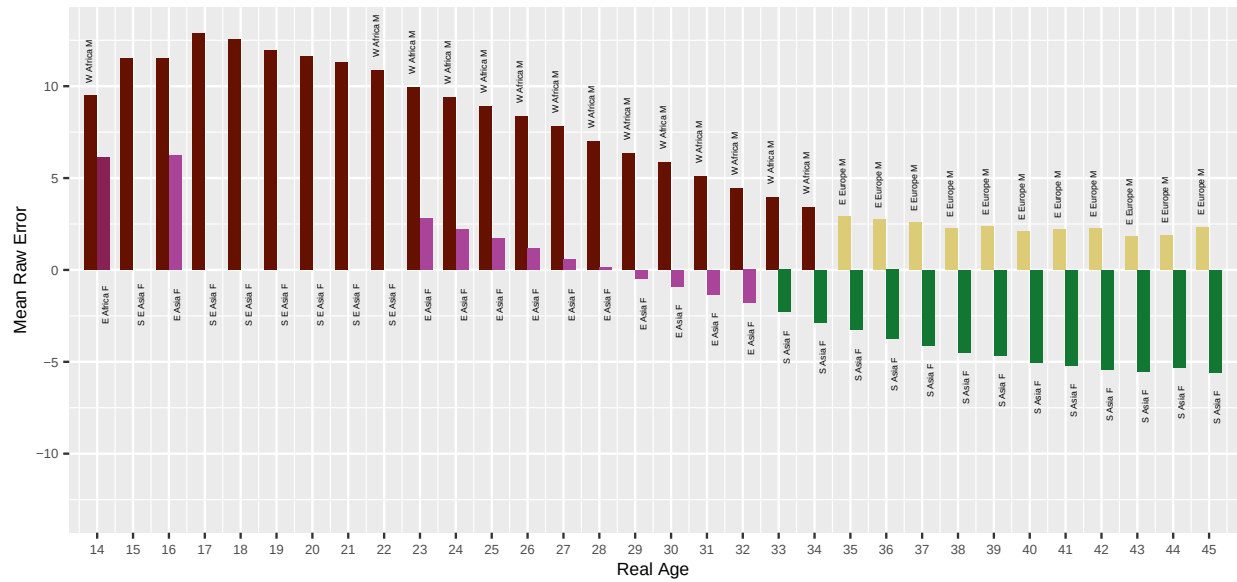
Fig. 23. For algorithm hzailu-001 applied to Border photos, the bar chart shows which demographic groups have the highest and lowest mean age estimation error, by age. Values closer to zero are better. Positive values are overestimate and negative values are underestimate.
