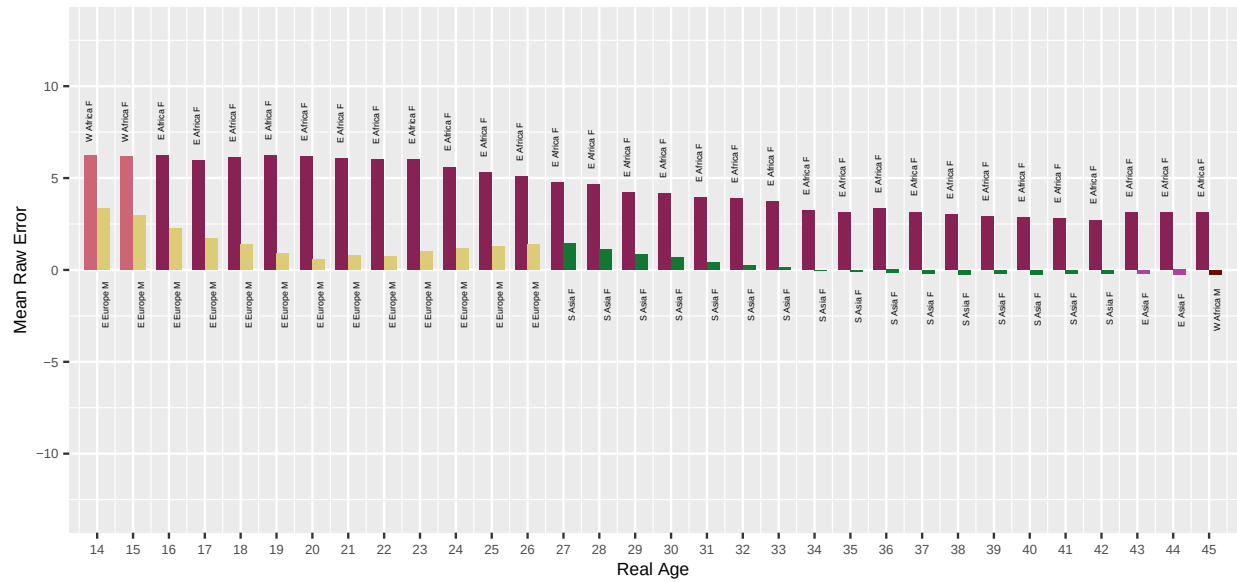
Fig. 49. For algorithm roc-001 applied to Border photos, the bar chart shows which demographic groups have the highest and lowest mean age estimation error, by age. Values closer to zero are better. Positive values are overestimate and negative values are underestimate.
