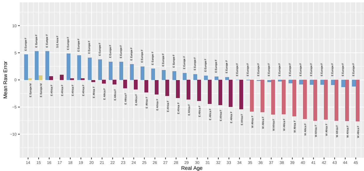
Fig. 20. For algorithm dermalog-002 applied to Application photos, the bar chart shows which demographic groups have the highest and lowest mean age estimation error, by age. Values closer to zero are better. Positive values are overestimate and negative values are underestimate.
