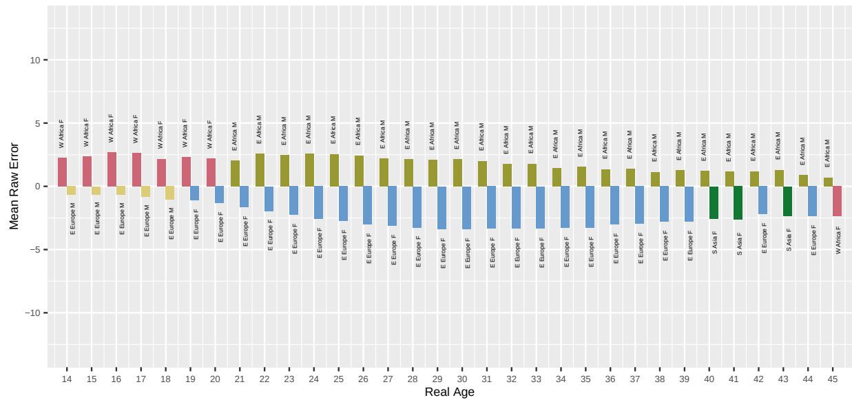
Fig. 24. For algorithm idemia-001 applied to Application photos, the bar chart shows which demographic groups have the highest and lowest mean age estimation error, by age. Values closer to zero are better. Positive values are overestimate and negative values are underestimate.
