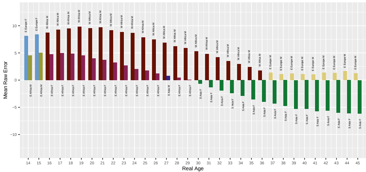
Fig. 22. For algorithm hzailu-001 applied to Application photos, the bar chart shows which demographic groups have the highest and lowest mean age estimation error, by age. Values closer to zero are better. Positive values are overestimate and negative values are underestimate.
