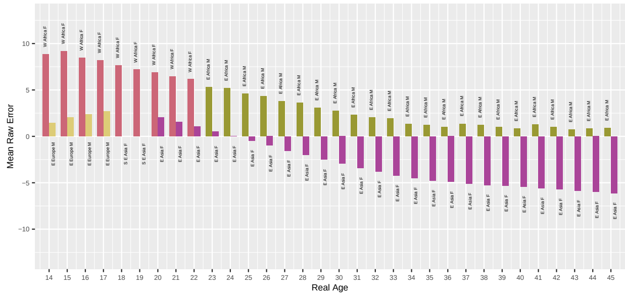
Fig. 27. For algorithm inbut-000 applied to Border photos, the bar chart shows which demographic groups have the highest and lowest mean age estimation error, by age. Values closer to zero are better. Positive values are overestimate and negative values are underestimate.
