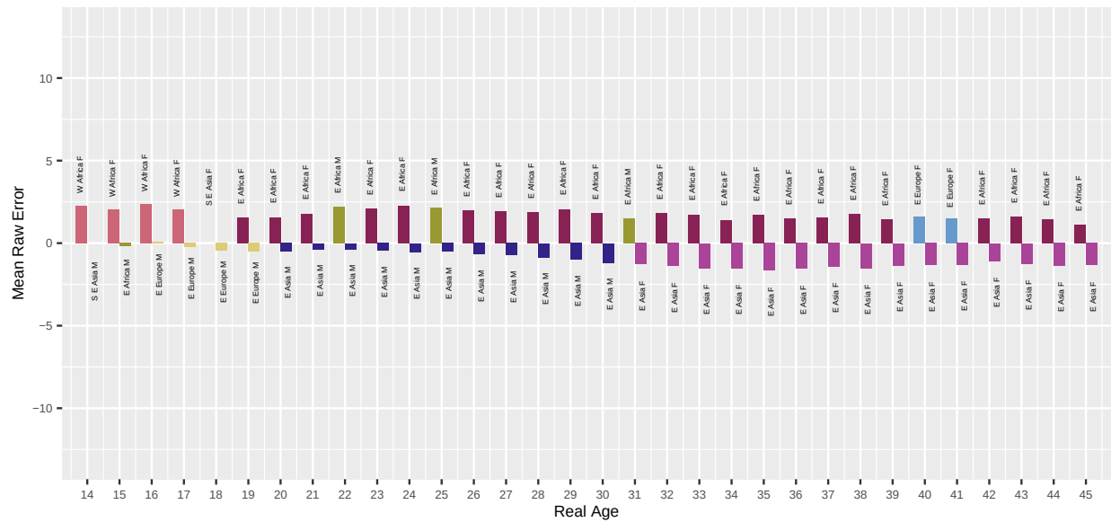
Fig. 28. For algorithm incode-000 applied to Application photos, the bar chart shows which demographic groups have the highest and lowest mean age estimation error, by age. Values closer to zero are better. Positive values are overestimate and negative values are underestimate.
