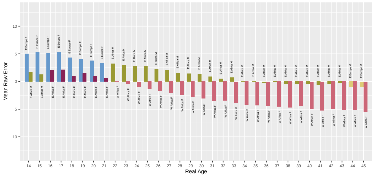
Fig. 18. For algorithm dermalog-001 applied to Application photos, the bar chart shows which demographic groups have the highest and lowest mean age estimation error, by age. Values closer to zero are better. Positive values are overestimate and negative values are underestimate.
