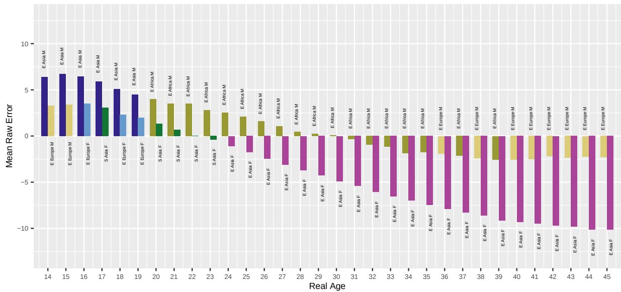
Fig. 36. For algorithm neurotechnology-001 applied to Application photos, the bar chart shows which demographic groups have the highest and lowest mean age estimation error, by age. Values closer to zero are better. Positive values are overestimate and negative values are underestimate.
