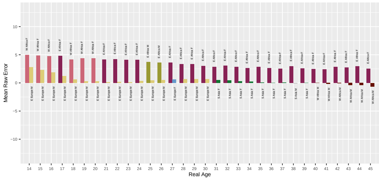
Fig. 48. For algorithm roc-001 applied to Application photos, the bar chart shows which demographic groups have the highest and lowest mean age estimation error, by age. Values closer to zero are better. Positive values are overestimate and negative values are underestimate.
