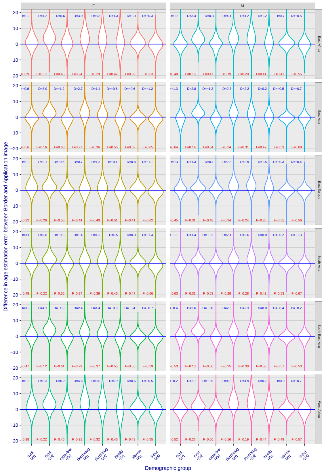
Fig. 58. Distribution of the pairwise age estimation error difference for Border and Application images. Positive values indicate larger error on Border images.
