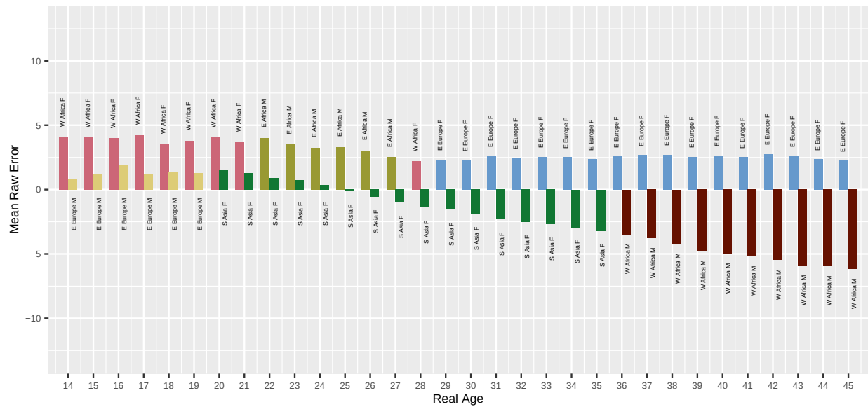
Fig. 50. For algorithm unissey-001 applied to Application photos, the bar chart shows which demographic groups have the highest and lowest mean age estimation error, by age. Values closer to zero are better. Positive values are overestimate and negative values are underestimate.
