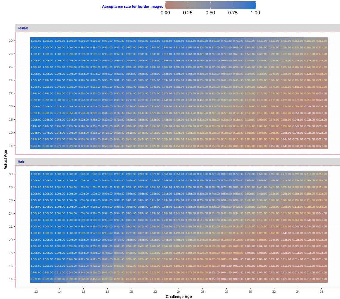
Fig. 68. For algorithm Incode 000 applied border-crossing photos, the heatmap and text shows proportion of photos of the persons of an actual age are accepted at a particular challenge age.
