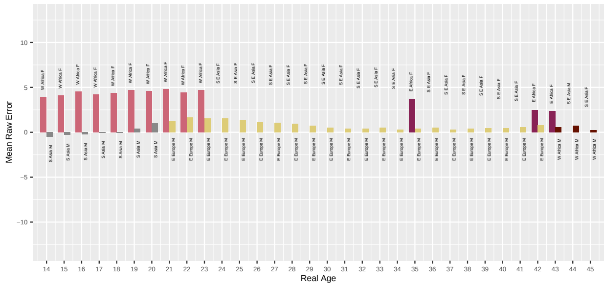
Fig. 54. For algorithm yoti-001 applied to Application photos, the bar chart shows which demographic groups have the highest and lowest mean age estimation error, by age. Values closer to zero are better. Positive values are overestimate and negative values are underestimate.
