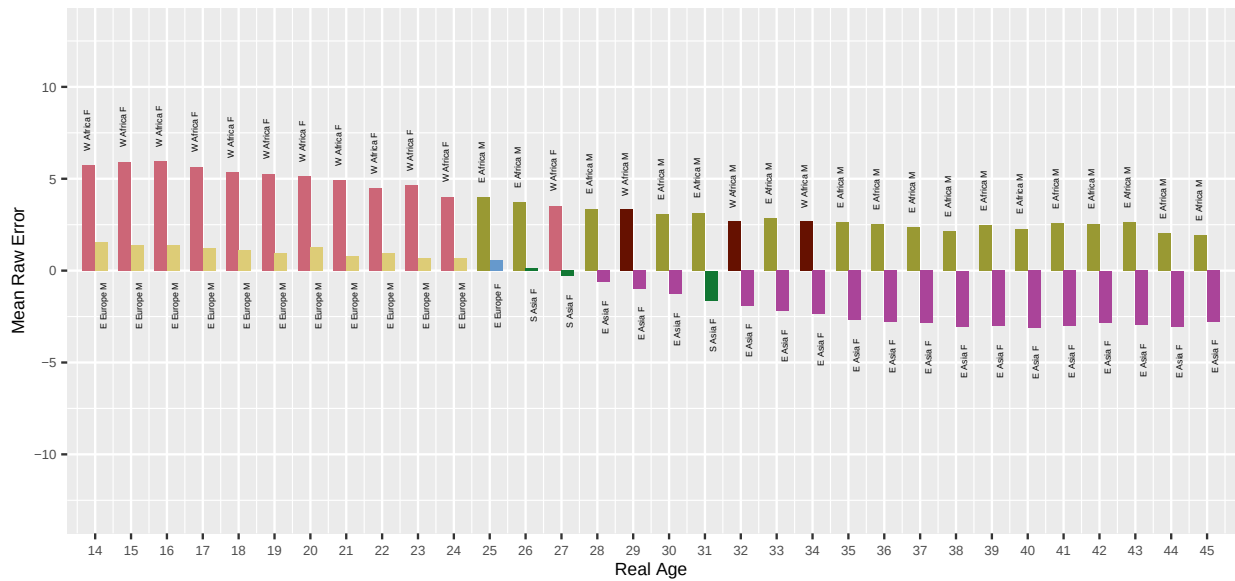
Fig. 42. For algorithm ondato-000 applied to Application photos, the bar chart shows which demographic groups have the highest and lowest mean age estimation error, by age. Values closer to zero are better. Positive values are overestimate and negative values are underestimate.
