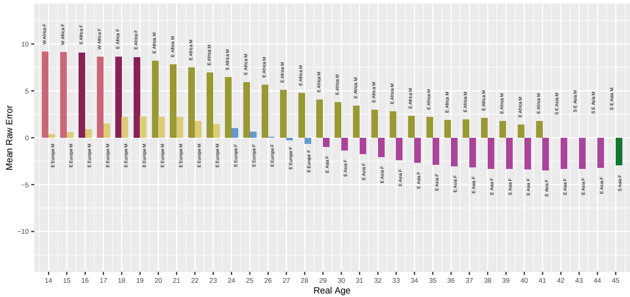
Fig. 53. For algorithm viante-000 applied to Border photos, the bar chart shows which demographic groups have the highest and lowest mean age estimation error, by age. Values closer to zero are better. Positive values are overestimate and negative values are underestimate.
