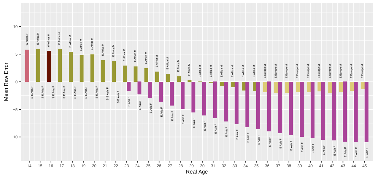
Fig. 37. For algorithm neurotechnology-001 applied to Border photos, the bar chart shows which demographic groups have the highest and lowest mean age estimation error, by age. Values closer to zero are better. Positive values are overestimate and negative values are underestimate.
