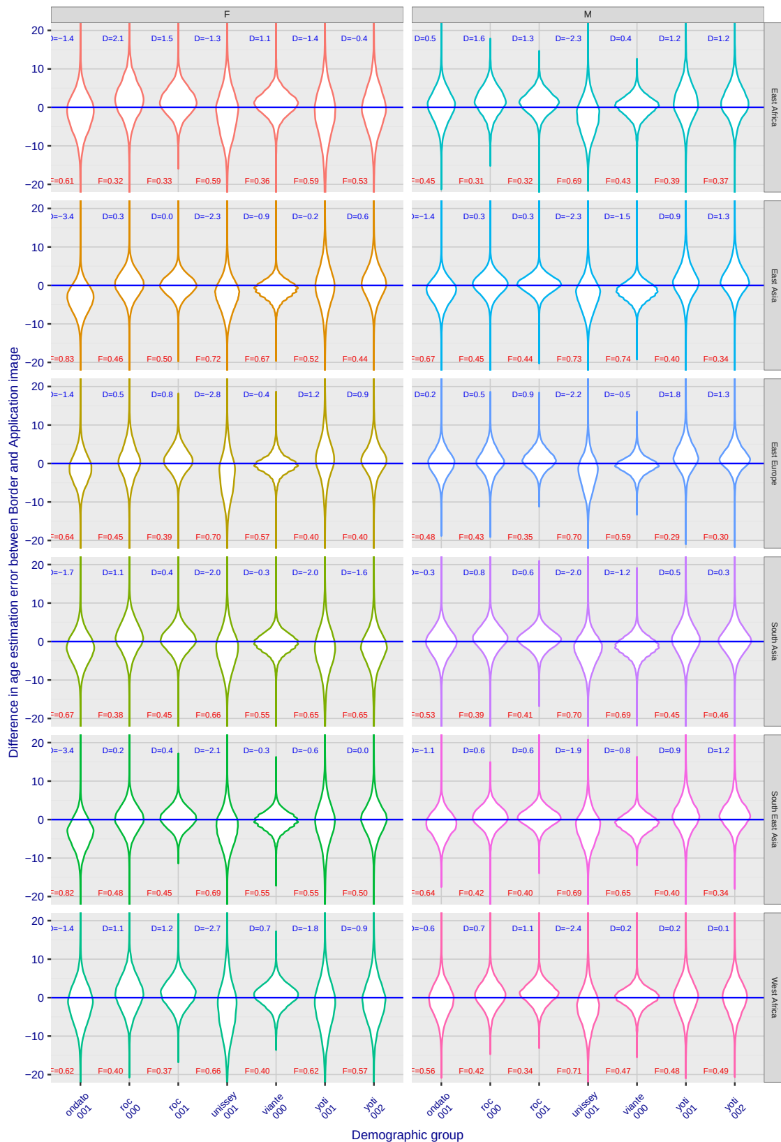
Fig. 60. Distribution of the pairwise age estimation error difference for Border and Application images. Positive values indicate larger error on Border images.
