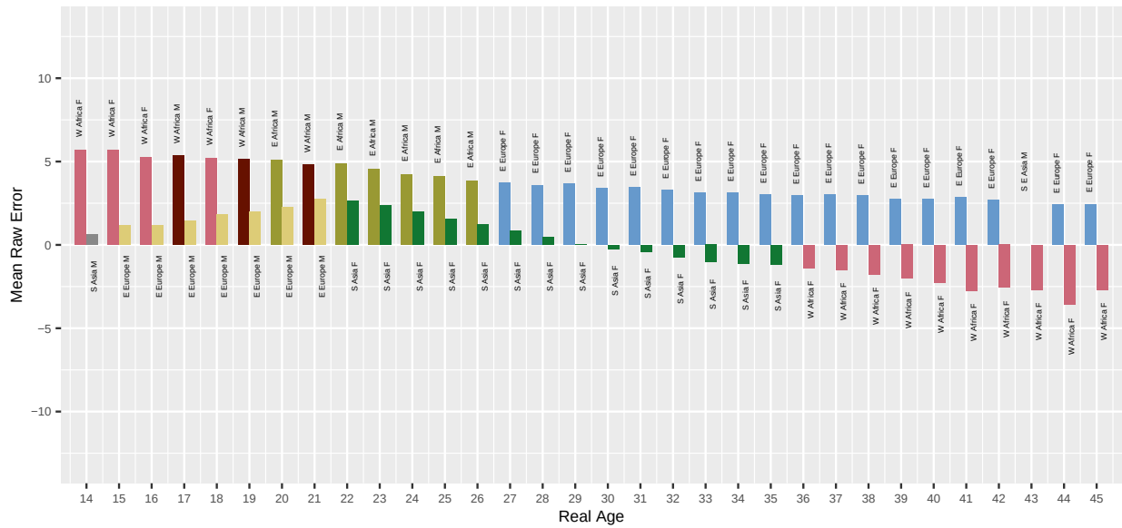
Fig. 55. For algorithm yoti-001 applied to Border photos, the bar chart shows which demographic groups have the highest and lowest mean age estimation error, by age. Values closer to zero are better. Positive values are overestimate and negative values are underestimate.
