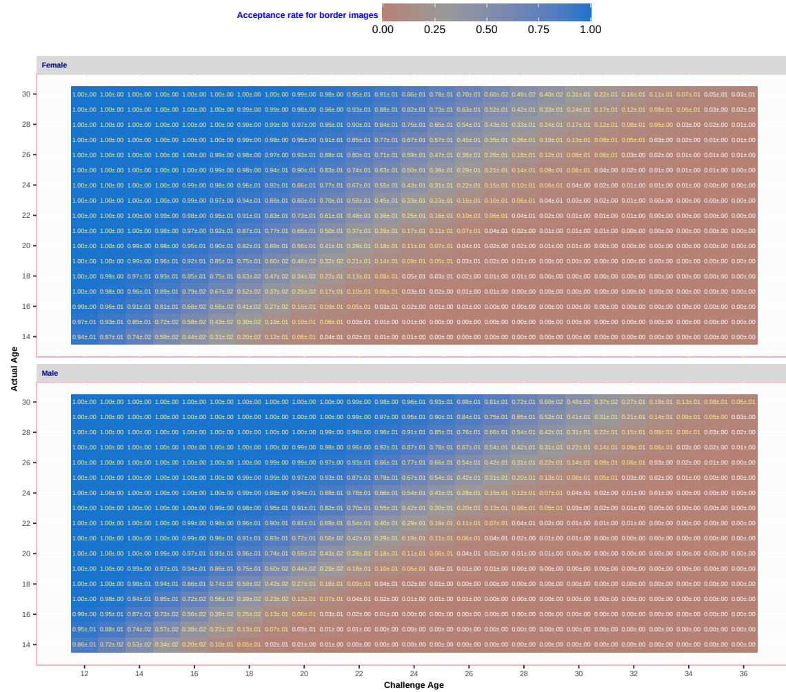
Fig. 67. For algorithm Idemia 001 applied border-crossing photos, the heatmap and text shows proportion of photos of the persons of an actual age are accepted at a particular challenge age.
