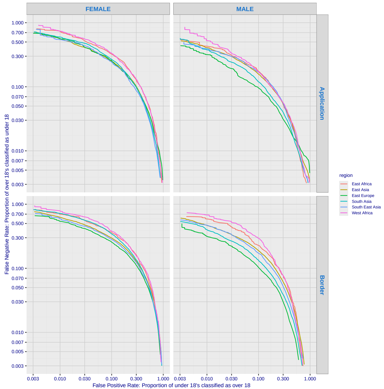
Fig. 122. For algorithm innovatrics-002 the error tradeoff characteristics show tradeoff between false positive and negative rates as the score confidence threshold is swept across it's full range. FPR quantifies how often the underage are classified above 18; FNR quantifies how those over age are not.
