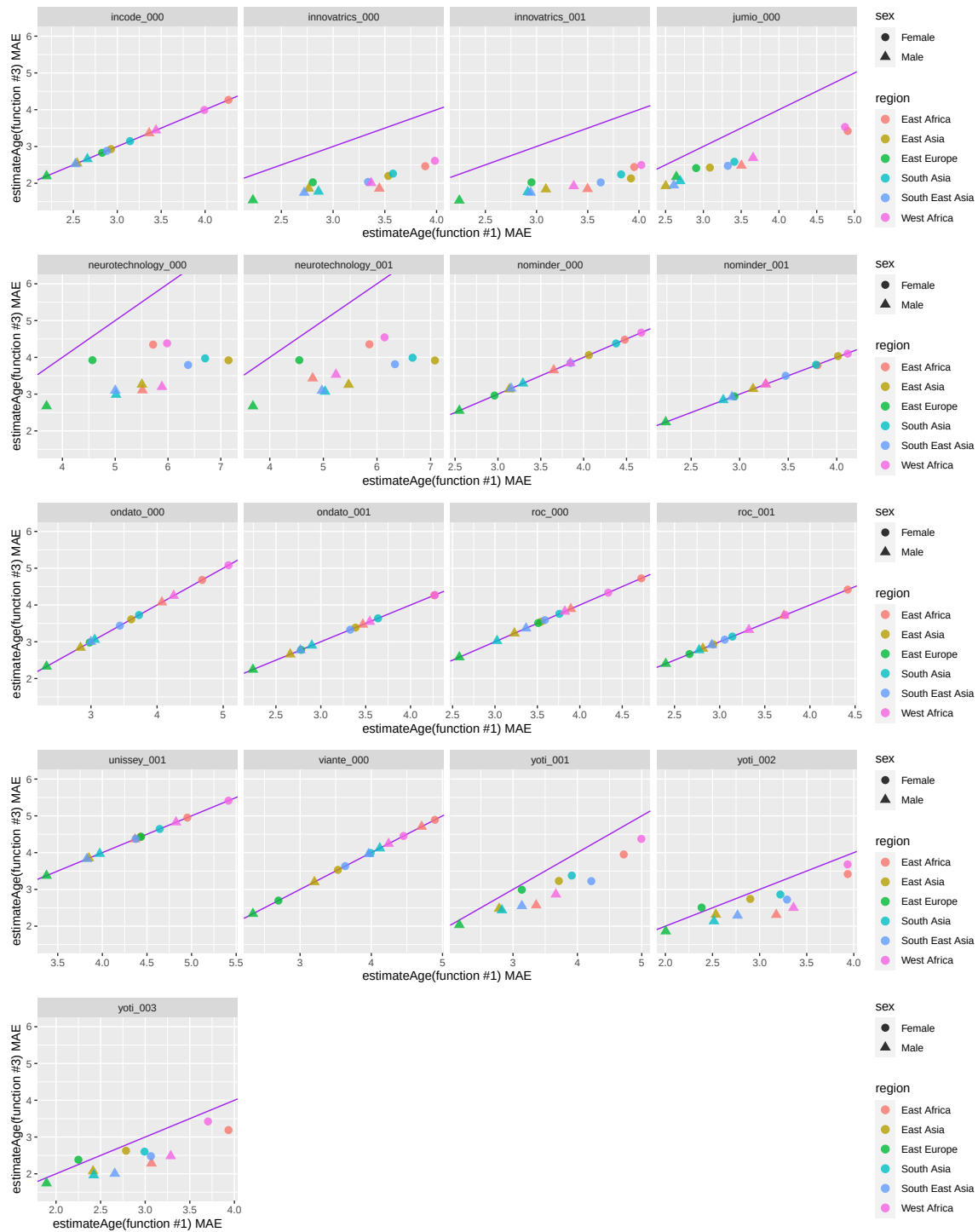
Fig. 115. In this figure, some algorithms show an improved MAE when given a prior image of known age to the second age estimate function. The x-axis represents the MAE for the first age estimation function, which returns the age estimate of a single image. In contrast, the y-axis represents the MAE for the second age estimation function, which returns the age estimate of an image when both the prior image and the known age of the same individual were provided.
