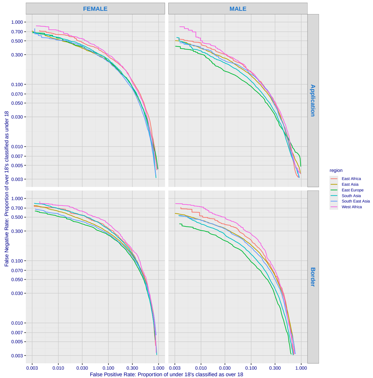
Fig. 123. For algorithm innovatrics-003 the error tradeoff characteristics show tradeoff between false positive and negative rates as the score confidence threshold is swept across it's full range. FPR quantifies how often the underage are classified above 18; FNR quantifies how those over age are not.
