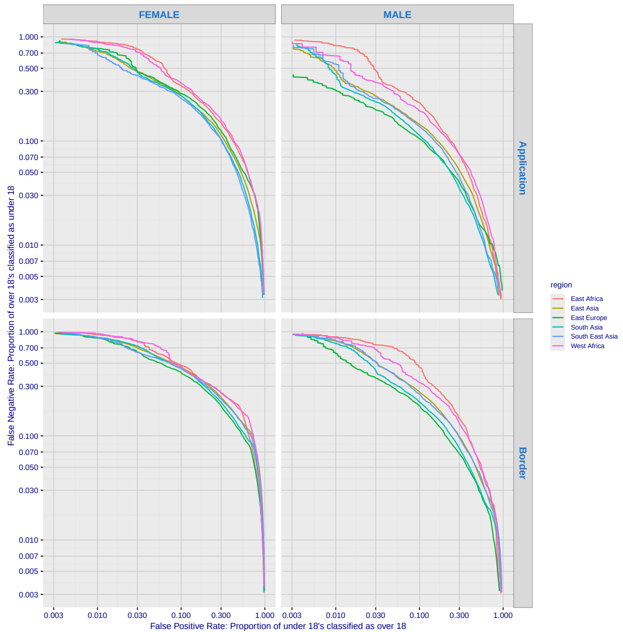
Fig. 126. For algorithm shufti-000 the error tradeoff characteristics show tradeoff between false positive and negative rates as the score confidence threshold is swept across it's full range. FPR quantifies how often the underage are classified above 18; FNR quantifies how those over age are not.
