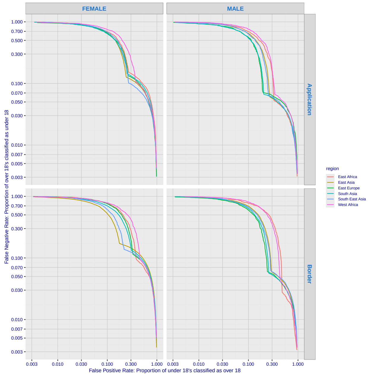
Fig. 120. For algorithm idemia-002 the error tradeoff characteristics show tradeoff between false positive and negative rates as the score confidence threshold is swept across it's full range. FPR quantifies how often the underage are classified above 18; FNR quantifies how those over age are not.
