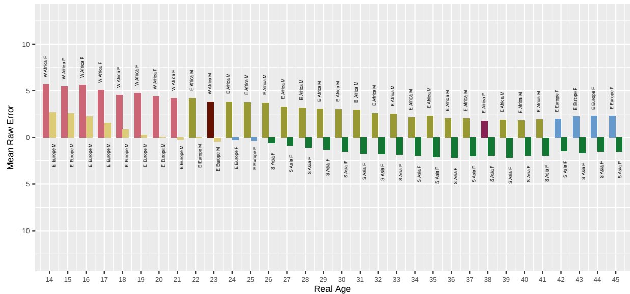
Fig. 74. For algorithm roc-000 applied to Application photos, the bar chart shows which demographic groups have the highest and lowest mean age estimation error, by age. Values closer to zero are better. Positive values are overestimate and negative values are underestimate.
