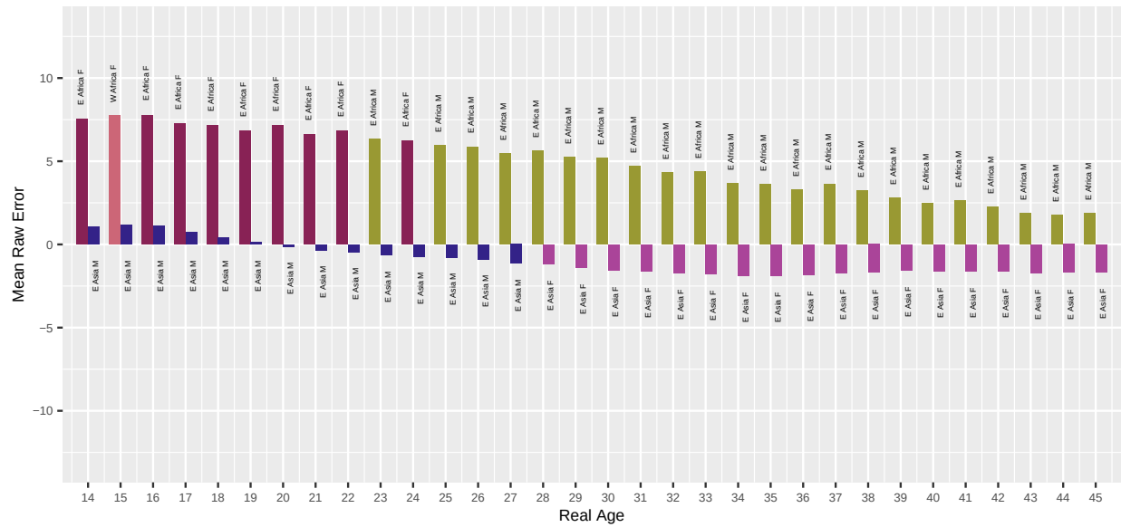
Fig. 43. For algorithm incode-000 applied to Border photos, the bar chart shows which demographic groups have the highest and lowest mean age estimation error, by age. Values closer to zero are better. Positive values are overestimate and negative values are underestimate.
