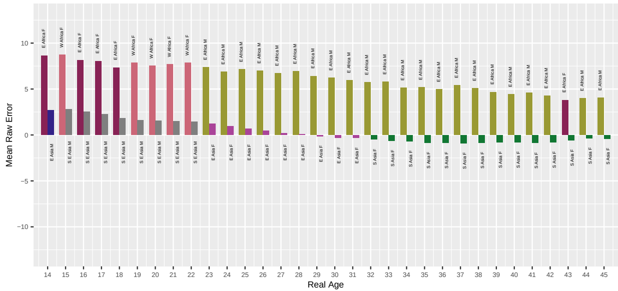
Fig. 45. For algorithm inc001 applied to Border photos, the bar chart shows which demographic groups have the highest and lowest mean age estimation error, by age. Values closer to zero are better. Positive values are overestimate and negative values are underestimate.
