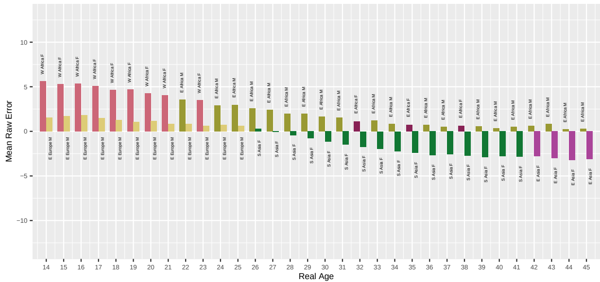
Fig. 66. For algorithm ondato-001 applied to Application photos, the bar chart shows which demographic groups have the highest and lowest mean age estimation error, by age. Values closer to zero are better. Positive values are overestimate and negative values are underestimate.
