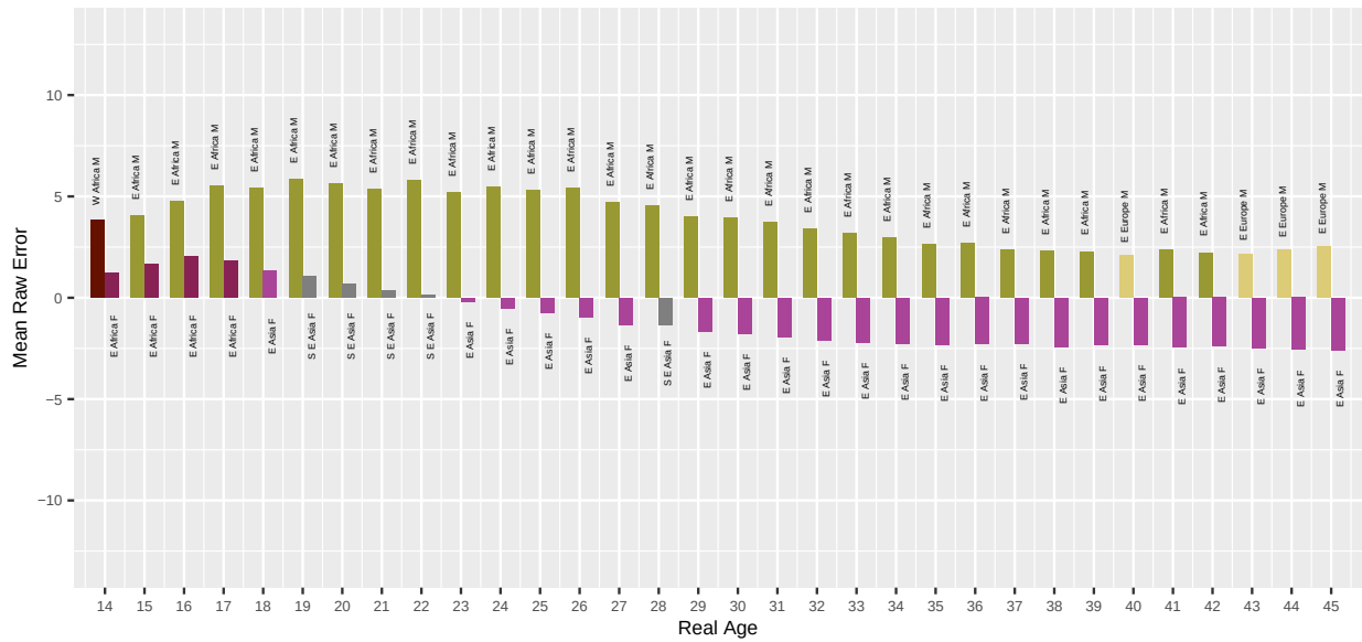
Fig. 81. For algorithm shufti-000 applied to Border photos, the bar chart shows which demographic groups have the highest and lowest mean age estimation error, by age. Values closer to zero are better. Positive values are overestimate and negative values are underestimate.
