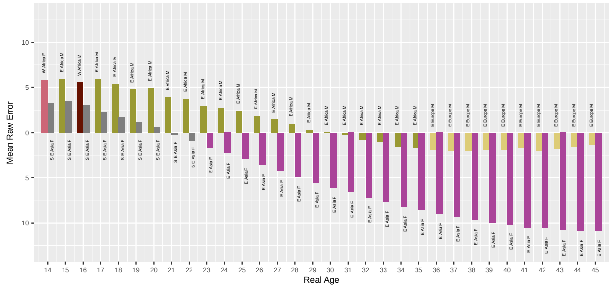
Fig. 59. For algorithm neurotechnology-001 applied to Border photos, the bar chart shows which demographic groups have the highest and lowest mean age estimation error, by age. Values closer to zero are better. Positive values are overestimate and negative values are underestimate.
