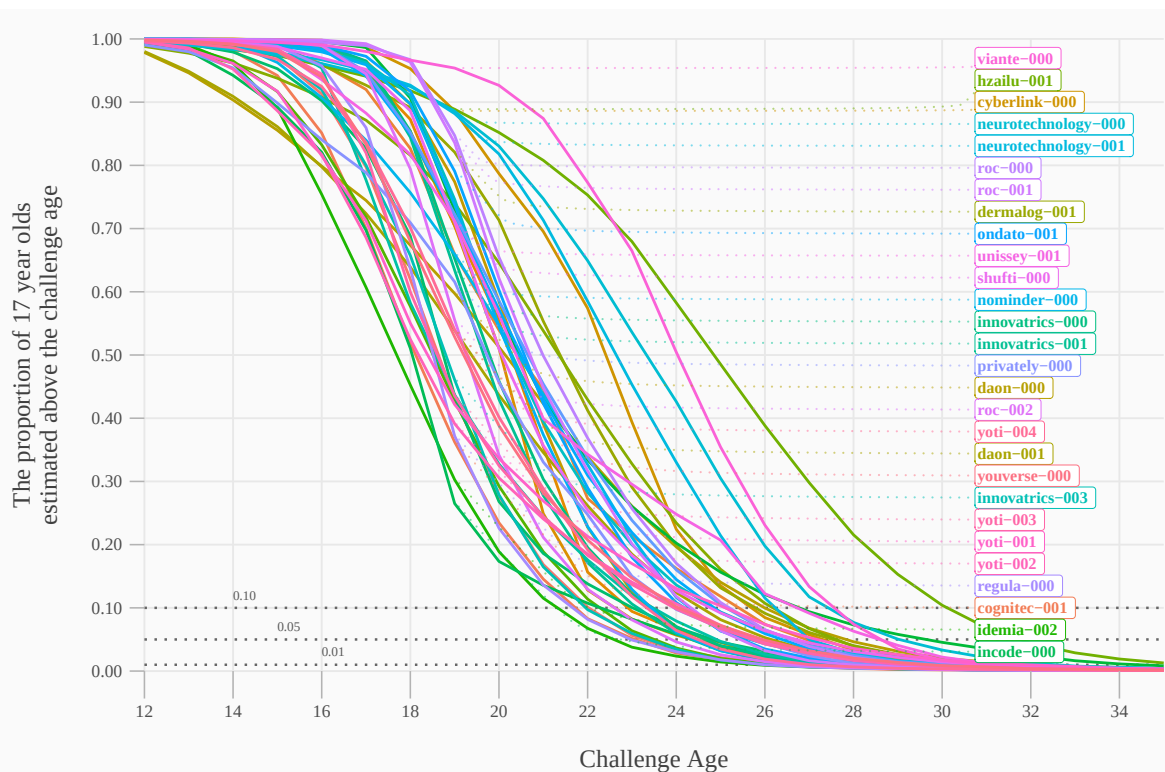
Fig. 9. The proportion of 17 year olds whose age is estimated as at or above the given challenge age. The Application images are of subjects from the set of countries used in the demographics analysis.
