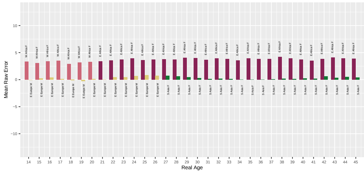
Fig. 44. For algorithm incode-001 applied to Application photos, the bar chart shows which demographic groups have the highest and lowest mean age estimation error, by age. Values closer to zero are better. Positive values are overestimate and negative values are underestimate.
