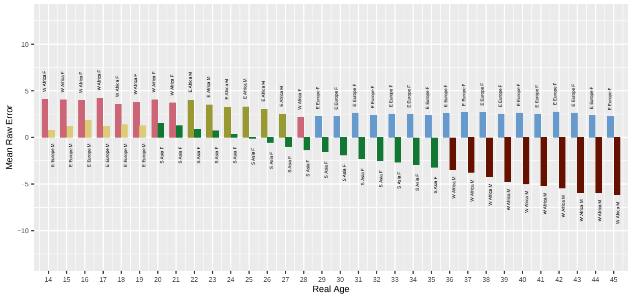
Fig. 82. For algorithm unissey-001 applied to Application photos, the bar chart shows which demographic groups have the highest and lowest mean age estimation error, by age. Values closer to zero are better. Positive values are overestimate and negative values are underestimate.
