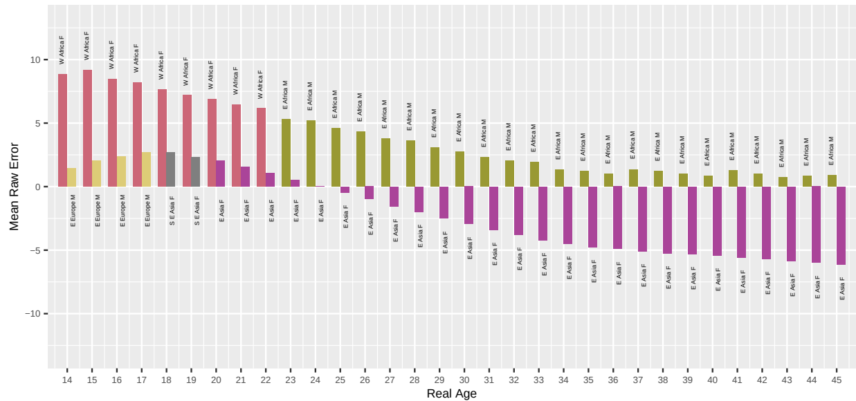
Fig. 41. For algorithm inbut-000 applied to Border photos, the bar chart shows which demographic groups have the highest and lowest mean age estimation error, by age. Values closer to zero are better. Positive values are overestimate and negative values are underestimate.
