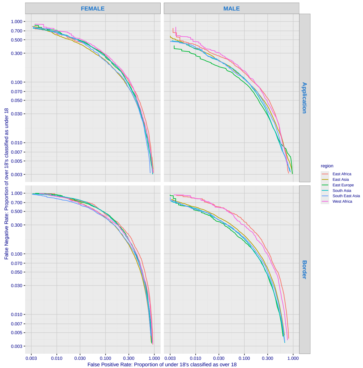
Fig. 124. For algorithm onfido-000 the error tradeoff characteristics show tradeoff between false positive and negative rates as the score confidence threshold is swept across it's full range. FPR quantifies how often the underage are classified above 18; FNR quantifies how those over age are not.
