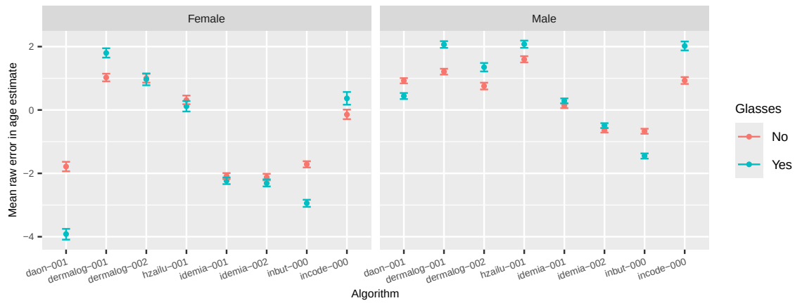
Fig. 103. Mean raw age estimation error for border crossing subjects for whom we have images with and without eyeglasses.
