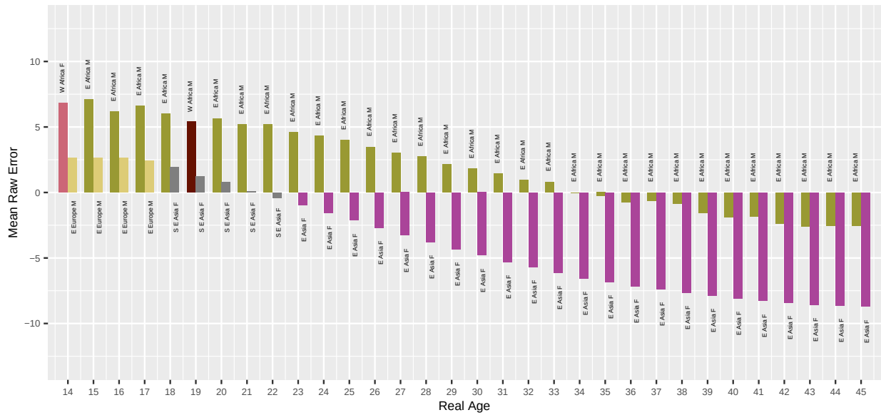
Fig. 65. For algorithm ondato-000 applied to Border photos, the bar chart shows which demographic groups have the highest and lowest mean age estimation error, by age. Values closer to zero are better. Positive values are overestimate and negative values are underestimate.
