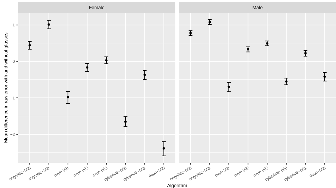
Fig. 108. Difference in age estimation error for border crossing subjects with and without eyeglasses.
