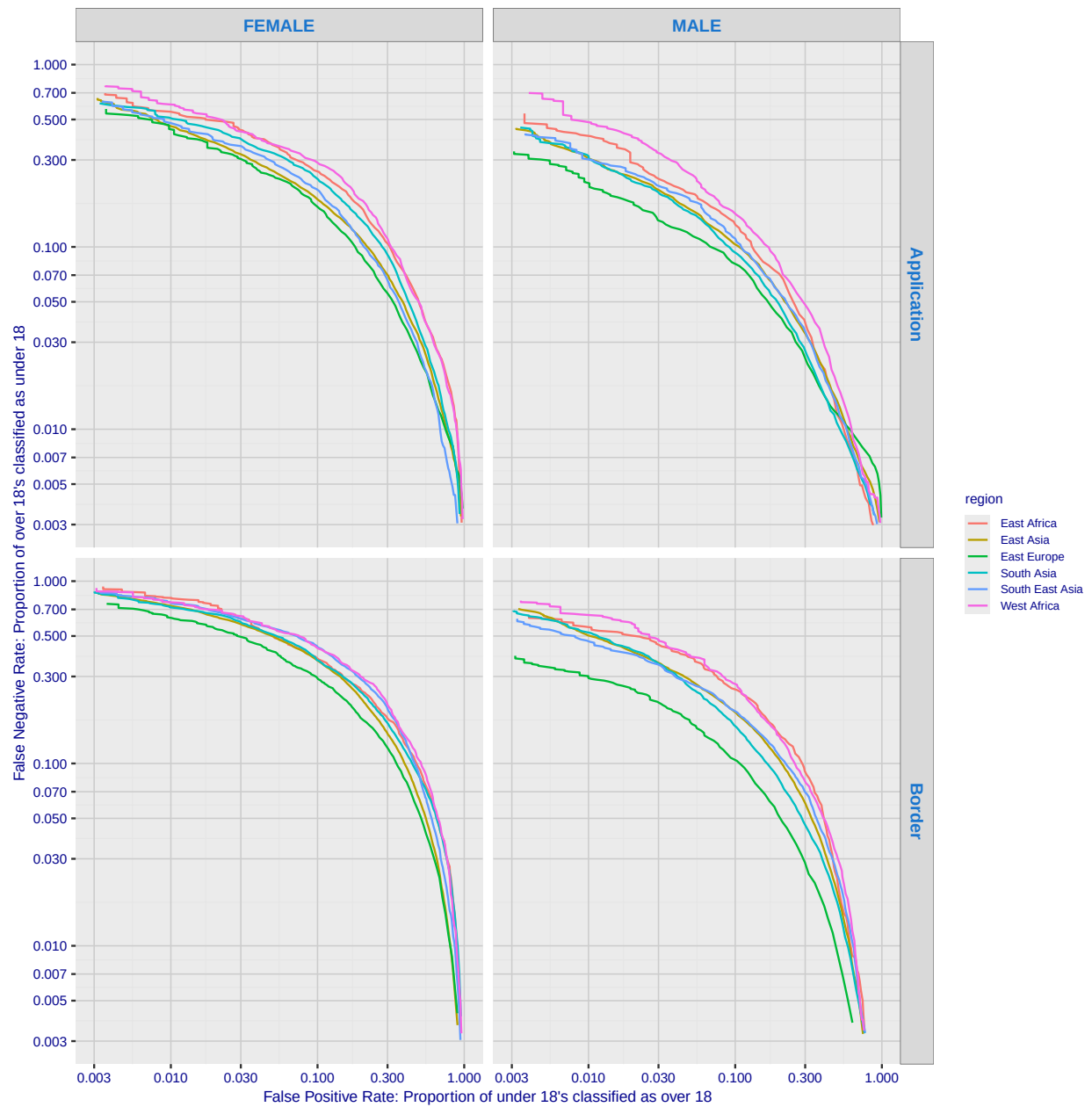
Fig. 128. For algorithm yoti-004 the error tradeoff characteristics show tradeoff between false positive and negative rates as the score confidence threshold is swept across it's full range. FPR quantifies how often the underage are classified above 18; FNR quantifies how those over age are not.
