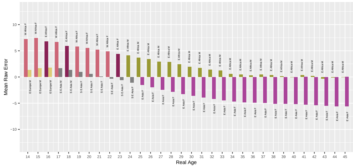
Fig. 47. For algorithm innovatrics-000 applied to Border photos, the bar chart shows which demographic groups have the highest and lowest mean age estimation error, by age. Values closer to zero are better. Positive values are overestimate and negative values are underestimate.
