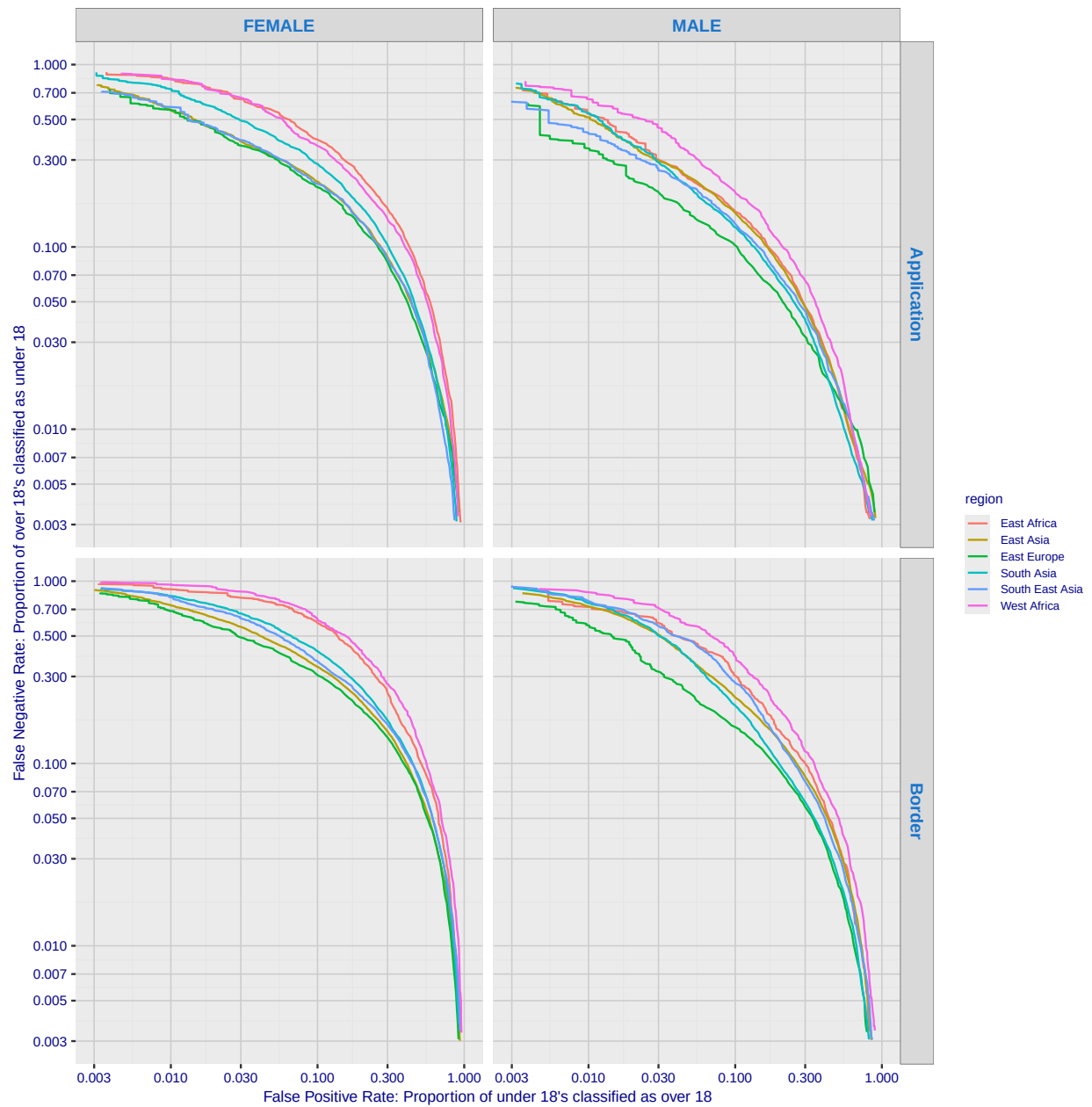
Fig. 117. For algorithm cognitec-001 the error tradeoff characteristics show tradeoff between false positive and negative rates as the score confidence threshold is swept across it's full range. FPR quantifies how often the underage are classified above 18; FNR quantifies how those over age are not.
