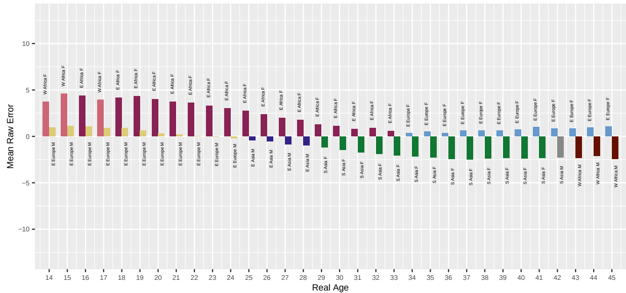
Fig. 73. For algorithm regula-000 applied to Border photos, the bar chart shows which demographic groups have the highest and lowest mean age estimation error, by age. Values closer to zero are better. Positive values are overestimate and negative values are underestimate.
