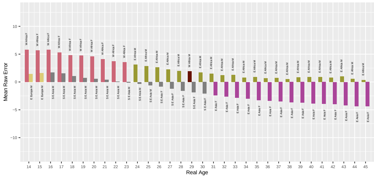
Fig. 46. For algorithm innovatrics-000 applied to Application photos, the bar chart shows which demographic groups have the highest and lowest mean age estimation error, by age. Values closer to zero are better. Positive values are overestimate and negative values are underestimate.
