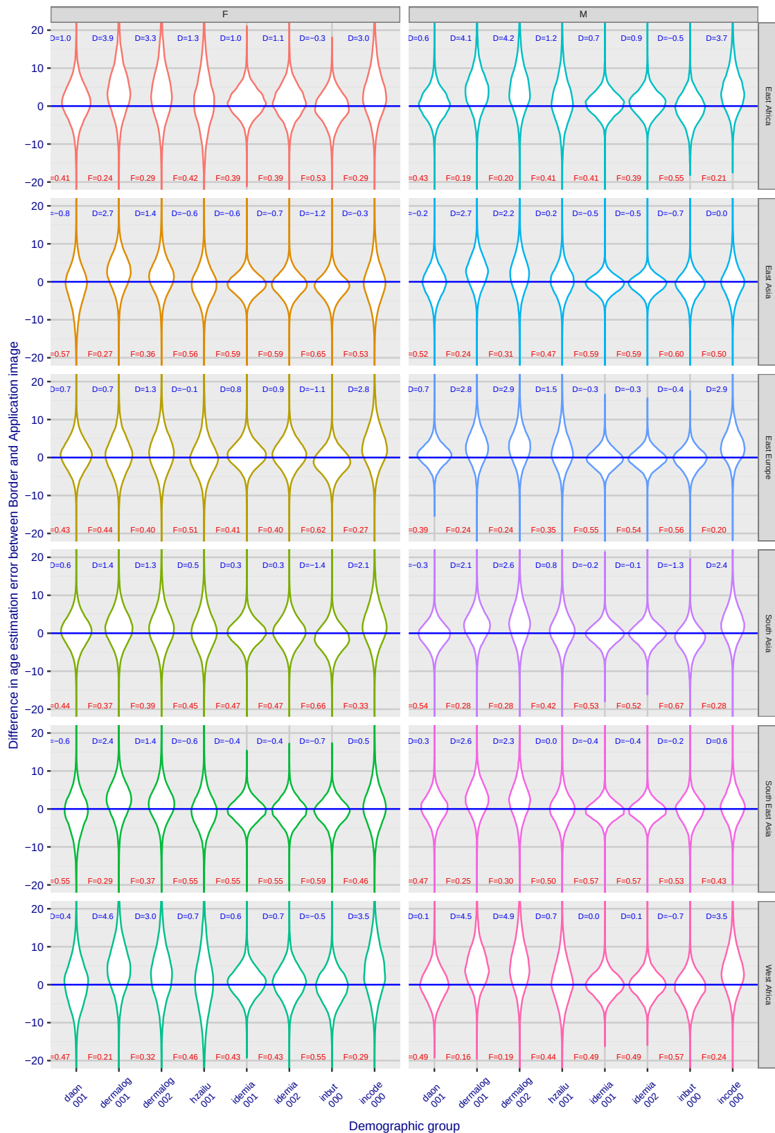
Fig. 97. Distribution of the pairwise age estimation error difference for Border and Application images. Positive values indicate larger error on Border images.
