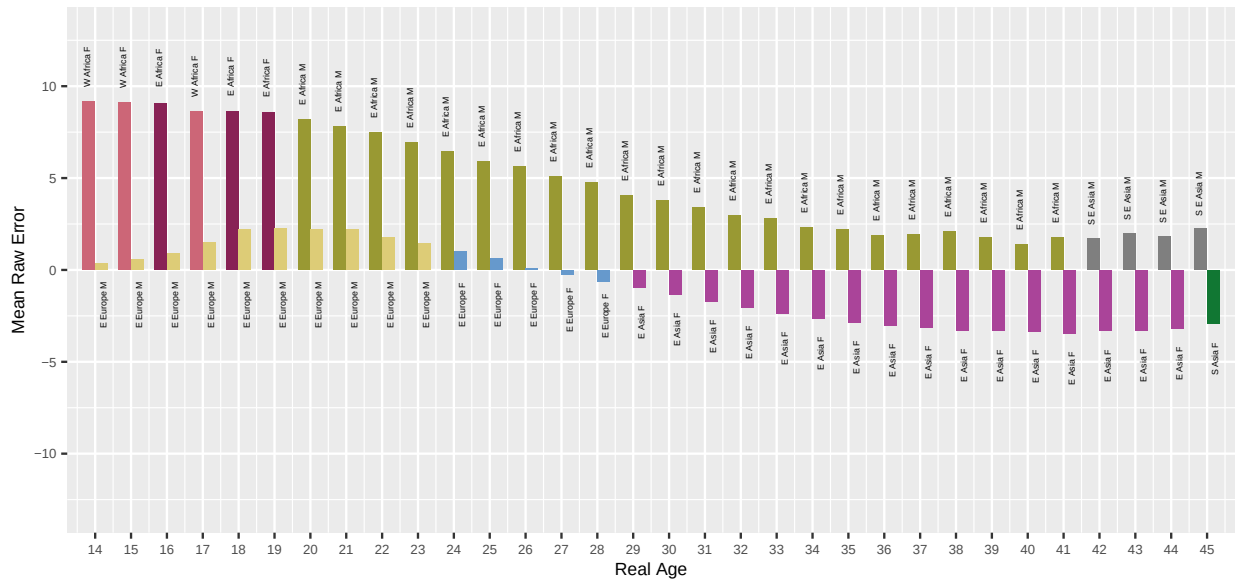
Fig. 85. For algorithm viante-000 applied to Border photos, the bar chart shows which demographic groups have the highest and lowest mean age estimation error, by age. Values closer to zero are better. Positive values are overestimate and negative values are underestimate.
