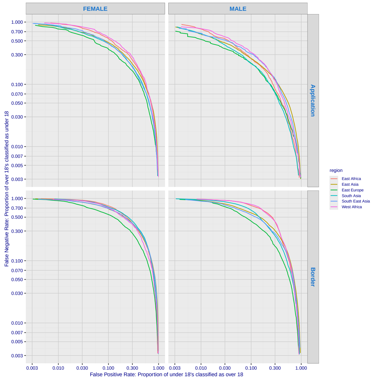
Fig. 129. For algorithm youverse-000 the error tradeoff characteristics show tradeoff between false positive and negative rates as the score confidence threshold is swept across it's full range. FPR quantifies how often the underage are classified above 18; FNR quantifies how those over age are not.
