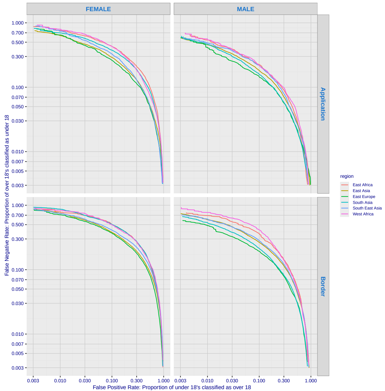
Fig. 119. For algorithm cyberlink-001 the error tradeoff characteristics show tradeoff between false positive and negative rates as the score confidence threshold is swept across it's full range. FPR quantifies how often the underage are classified above 18; FNR quantifies how those over age are not.
