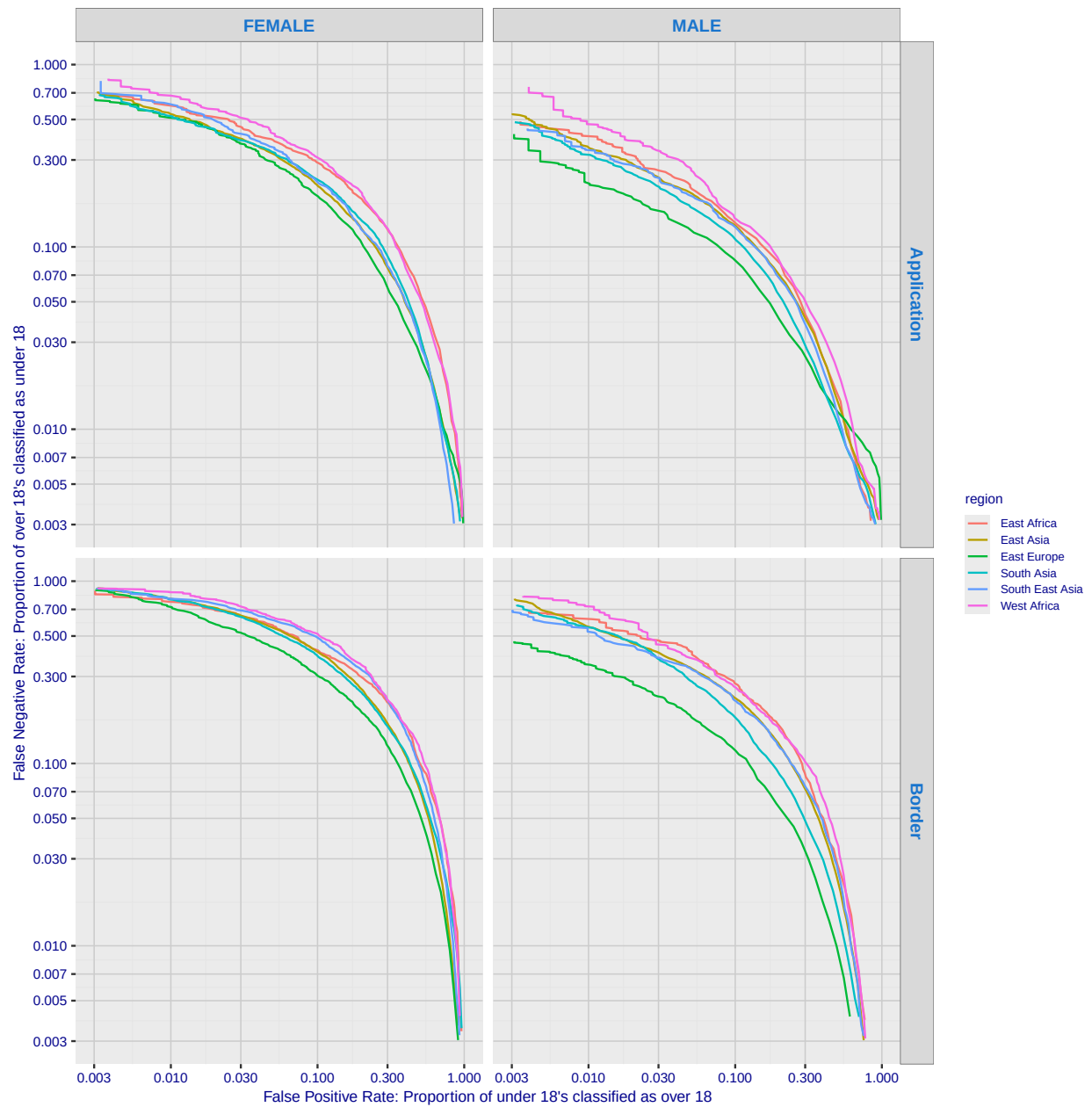
Fig. 127. For algorithm yoti-003 the error tradeoff characteristics show tradeoff between false positive and negative rates as the score confidence threshold is swept across it's full range. FPR quantifies how often the underage are classified above 18; FNR quantifies how those over age are not.
