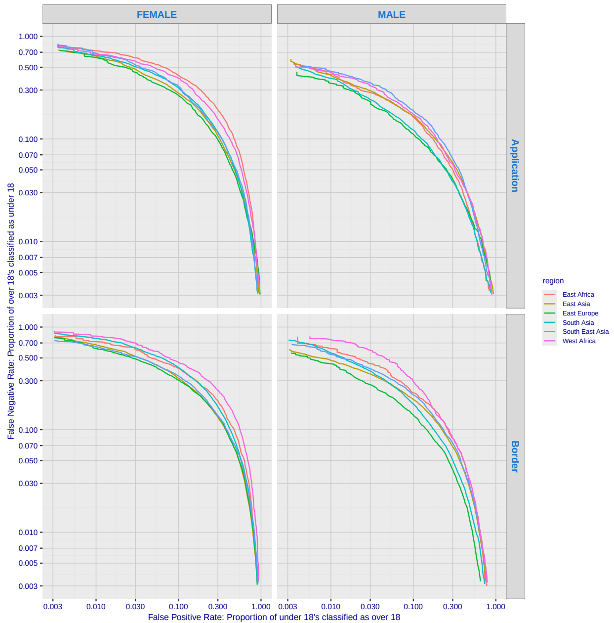
Fig. 118. For algorithm cvut-003 the error tradeoff characteristics show tradeoff between false positive and negative rates as the score confidence threshold is swept across it's full range. FPR quantifies how often the underage are classified above 18; FNR quantifies how those over age are not.
