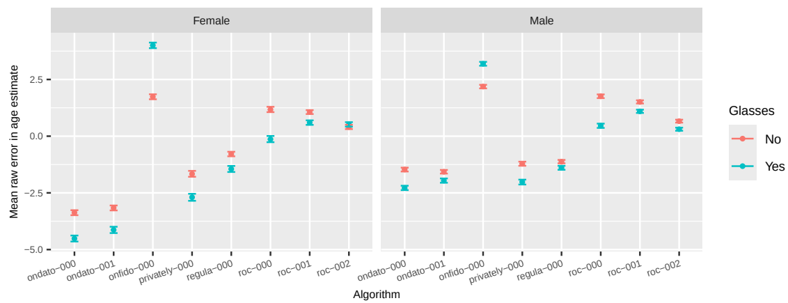
Fig. 100. Mean raw age estimation error for border crossing subjects for whom we have images with and without eyeglasses.
