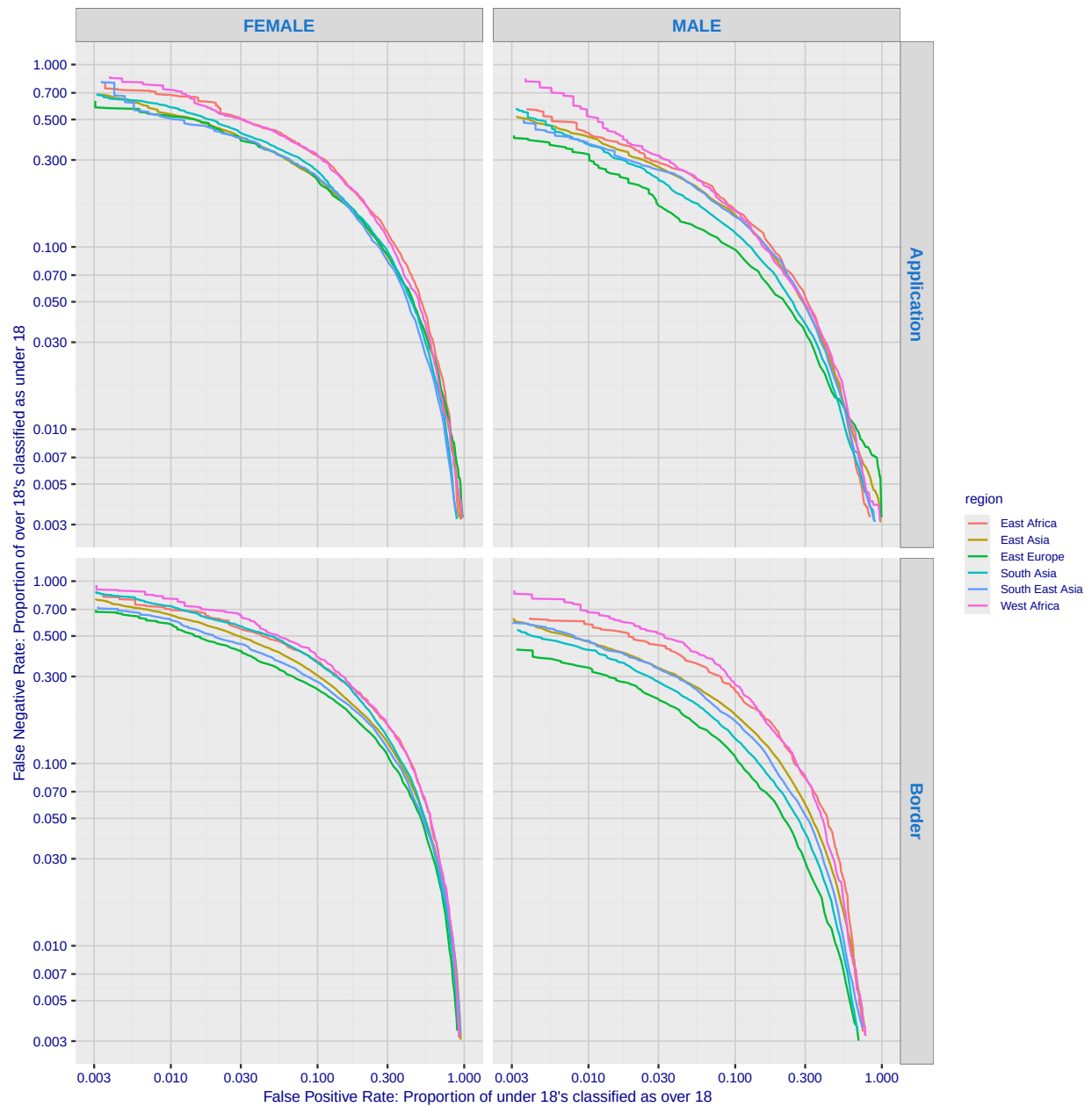
Fig. 114. For algorithm innovatrics-001 the error tradeoff characteristics show tradeoff between false positive and negative rates as the score confidence threshold is swept across it's full range. FPR quantifies how often the underage are classified above 18; FNR quantifies how those over age are not.
