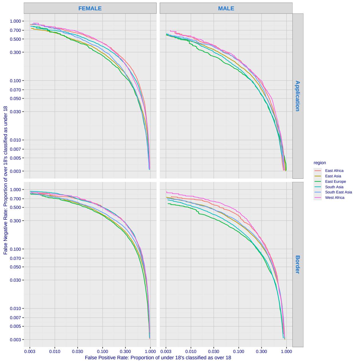
Fig. 112. For algorithm cyberlink-001 the error tradeoff characteristics show tradeoff between false positive and negative rates as the score confidence threshold is swept across it's full range. FPR quantifies how often the underage are classified above 18; FNR quantifies how those over age are not.
