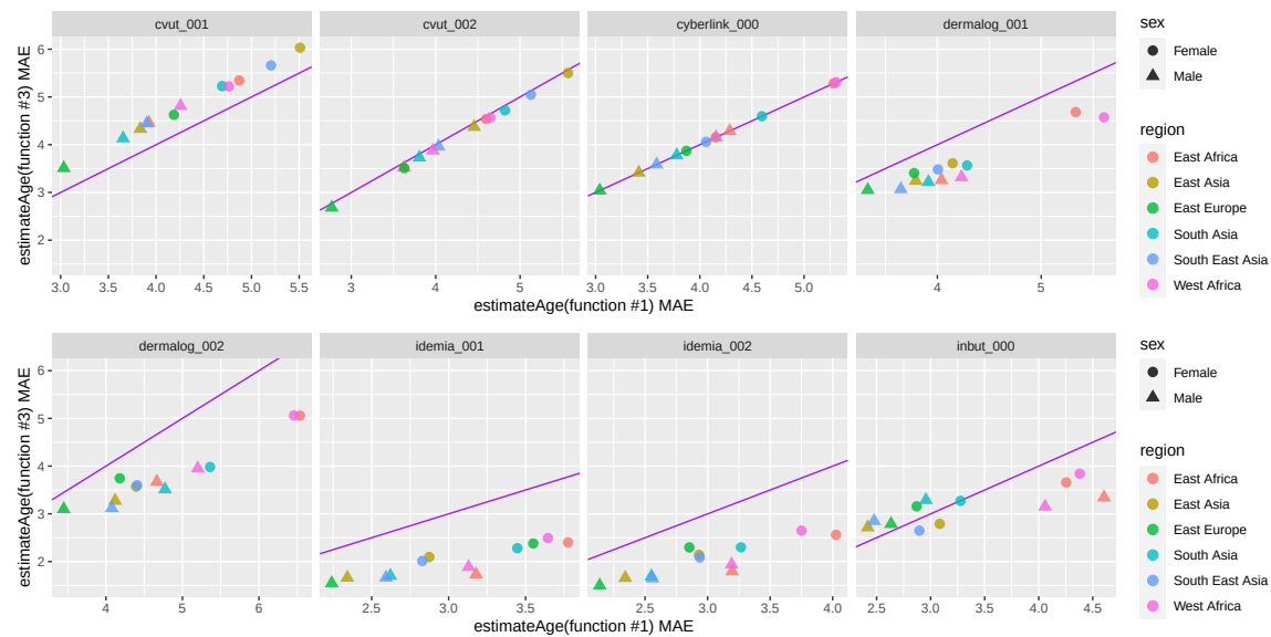
Fig. 107. In this figure, some algorithms show an improved MAE when given a prior image of known age to the second age estimate function. The x-axis represents the MAE for the first age estimation function, which returns the age estimate of a single image. In contrast, the y-axis represents the MAE for the second age estimation function, which returns the age estimate of an image when both the prior image and the known age of the same individual were provided.
