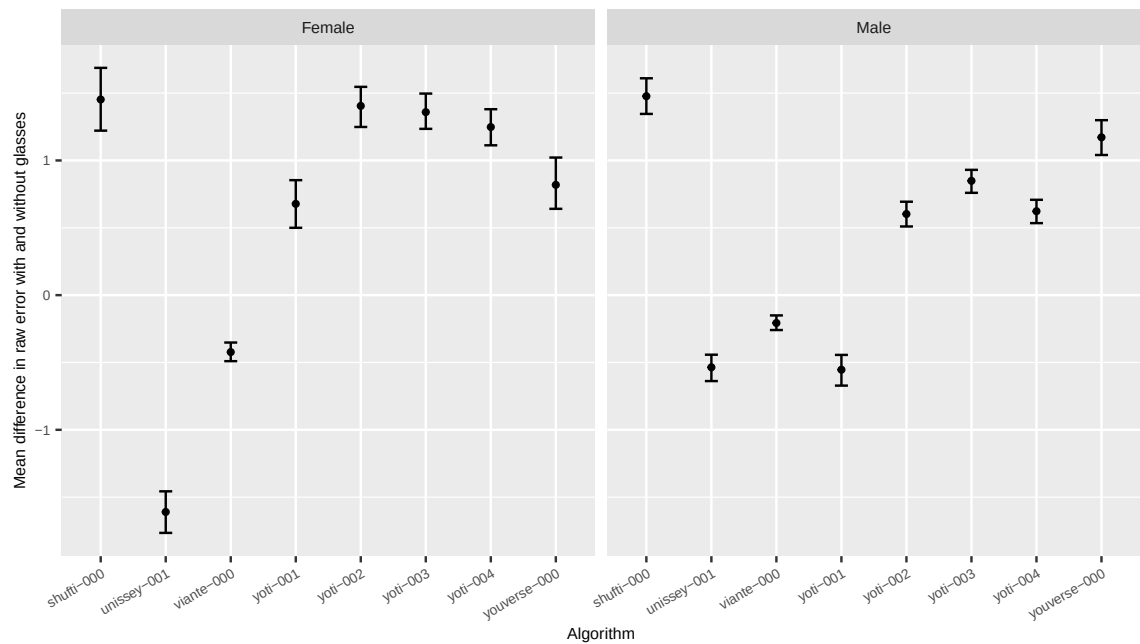
Fig. 106. Difference in age estimation error for border crossing subjects with and without eyeglasses.
