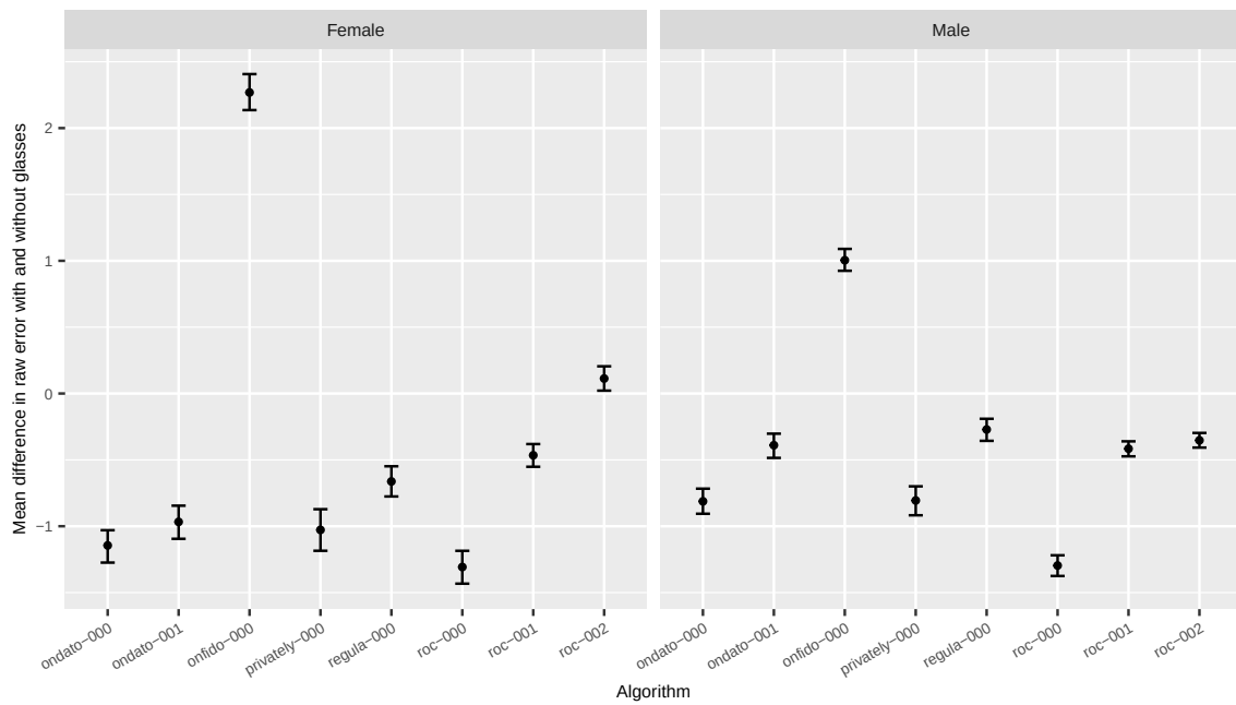
Fig. 105. Difference in age estimation error for border crossing subjects with and without eyeglasses.
