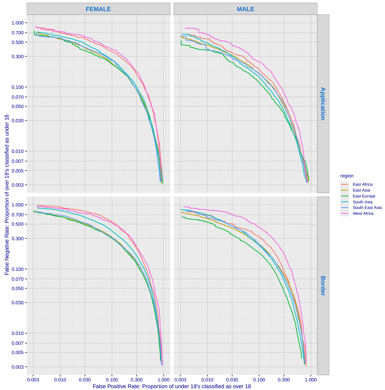
Fig. 110. For algorithm cognitec-000 the error tradeoff characteristics show tradeoff between false positive and negative rates as the score confidence threshold is swept across it's full range. FPR quantifies how often the underage are classified above 18; FNR quantifies how those over age are not.
