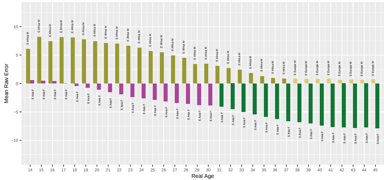
Fig. 25. For algorithm daon-000 applied to Border photos, the bar chart shows which demographic groups have the highest and lowest mean age estimation error, by age. Values closer to zero are better. Positive values are overestimate and negative values are underestimate.
