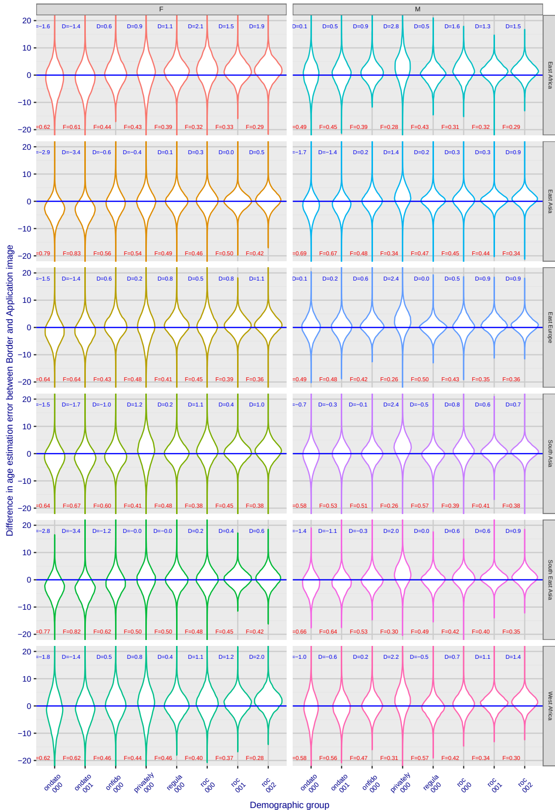
Fig. 95. Distribution of the pairwise age estimation error difference for Border and Application images. Positive values indicate larger error on Border images.
