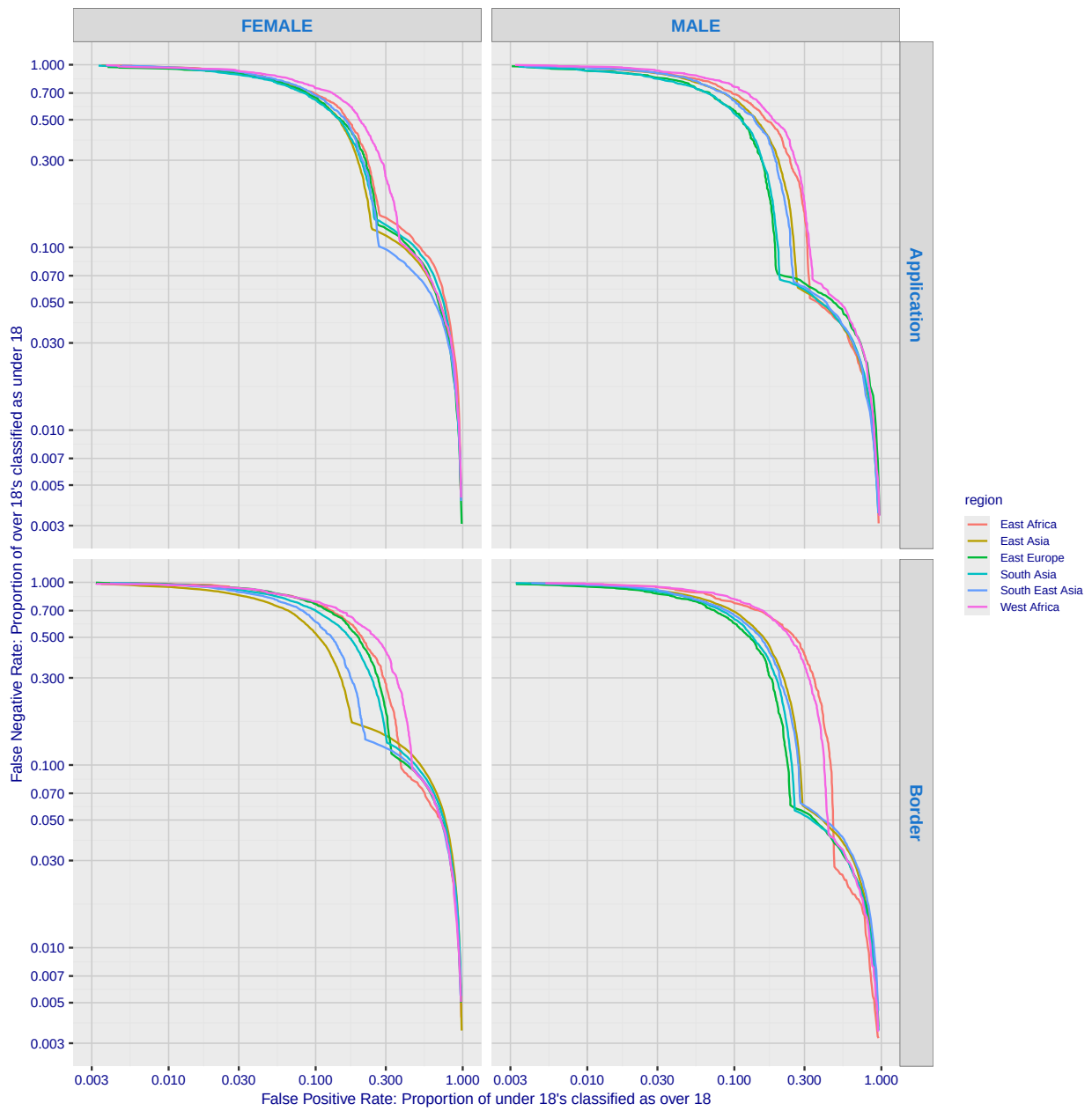
Fig. 113. For algorithm idemia-002 the error tradeoff characteristics show tradeoff between false positive and negative rates as the score confidence threshold is swept across it's full range. FPR quantifies how often the underage are classified above 18; FNR quantifies how those over age are not.
