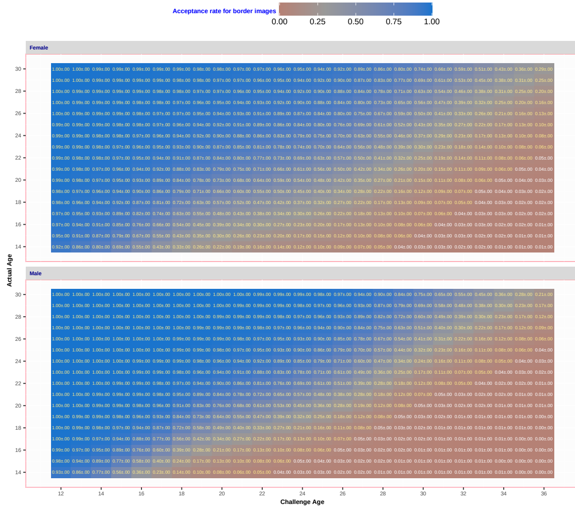
Fig. 57. For algorithm Yoti 001 applied border-crossing photos, the heatmap and text shows proportion of photos of the persons of an actual age are accepted at a particular challenge age.
