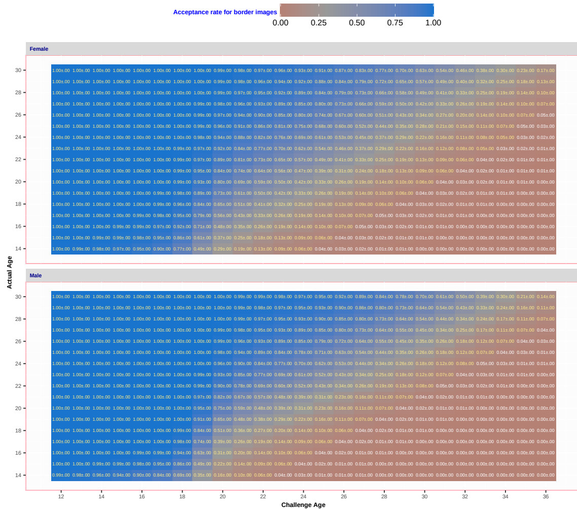
Fig. 55. For algorithm ROC 000 applied border-crossing photos, the heatmap and text shows proportion of photos of the persons of an actual age are accepted at a particular challenge age.
