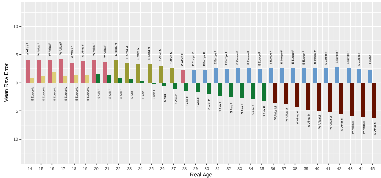
Fig. 37. For algorithm unissey-001 applied to Application photos, the bar chart shows which demographic groups have the highest and lowest mean age estimation error, by age. Values closer to zero are better. Positive values are overestimate and negative values are underestimate.
