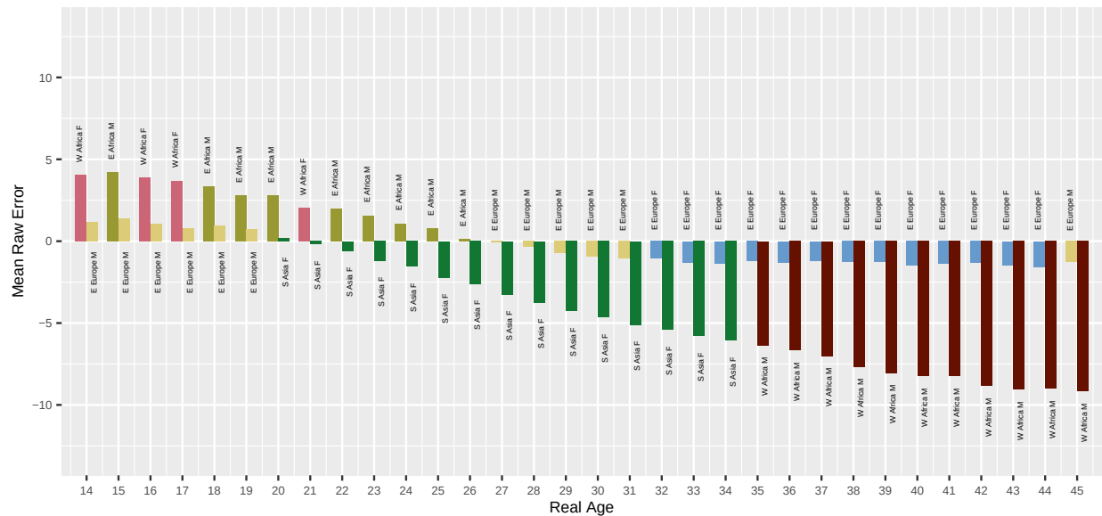
Fig. 38. For algorithm unissey-001 applied to Border photos, the bar chart shows which demographic groups have the highest and lowest mean age estimation error, by age. Values closer to zero are better. Positive values are overestimate and negative values are underestimate.
