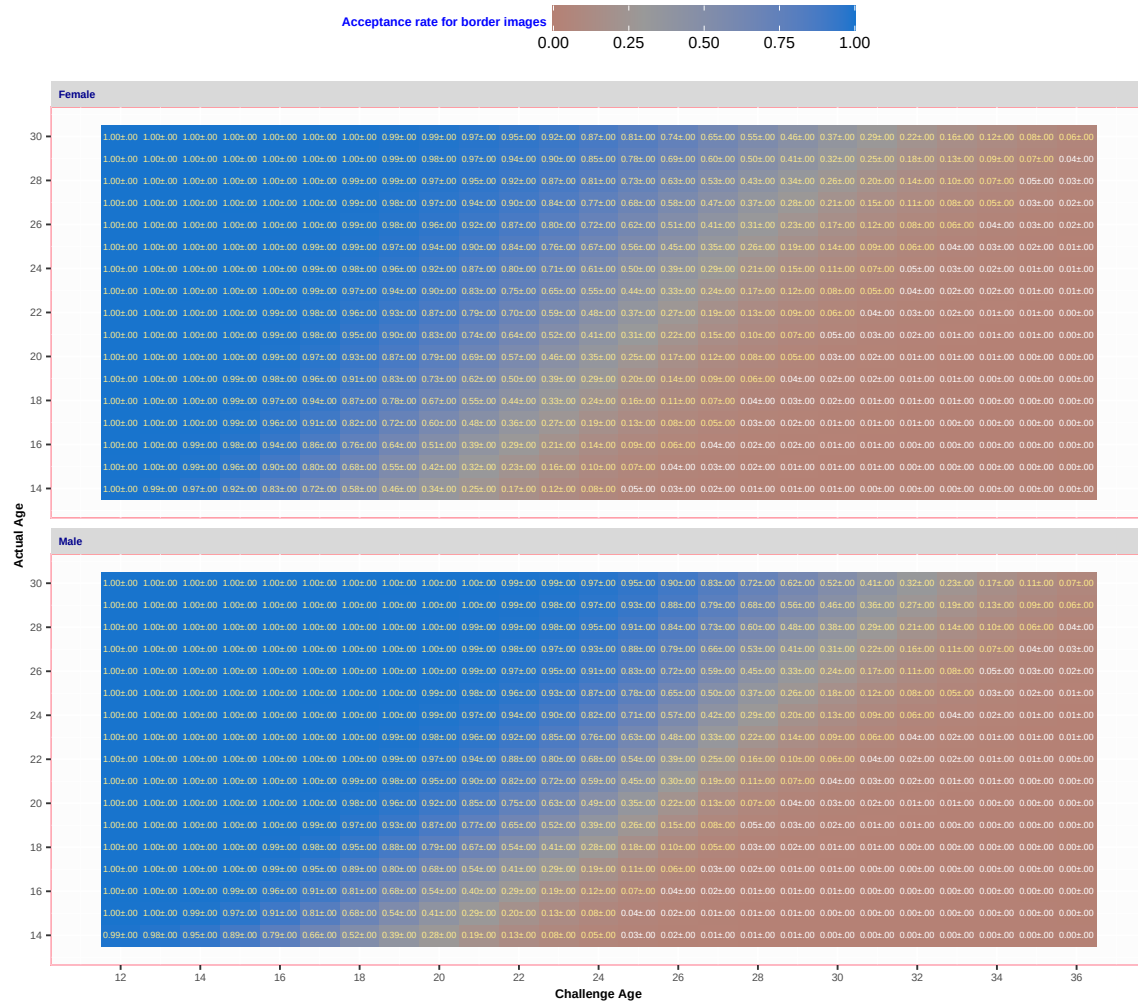
Fig. 50. For algorithm Nominder 000 applied border-crossing photos, the heatmap and text shows proportion of photos of the persons of an actual age are accepted at a particular challenge age.
