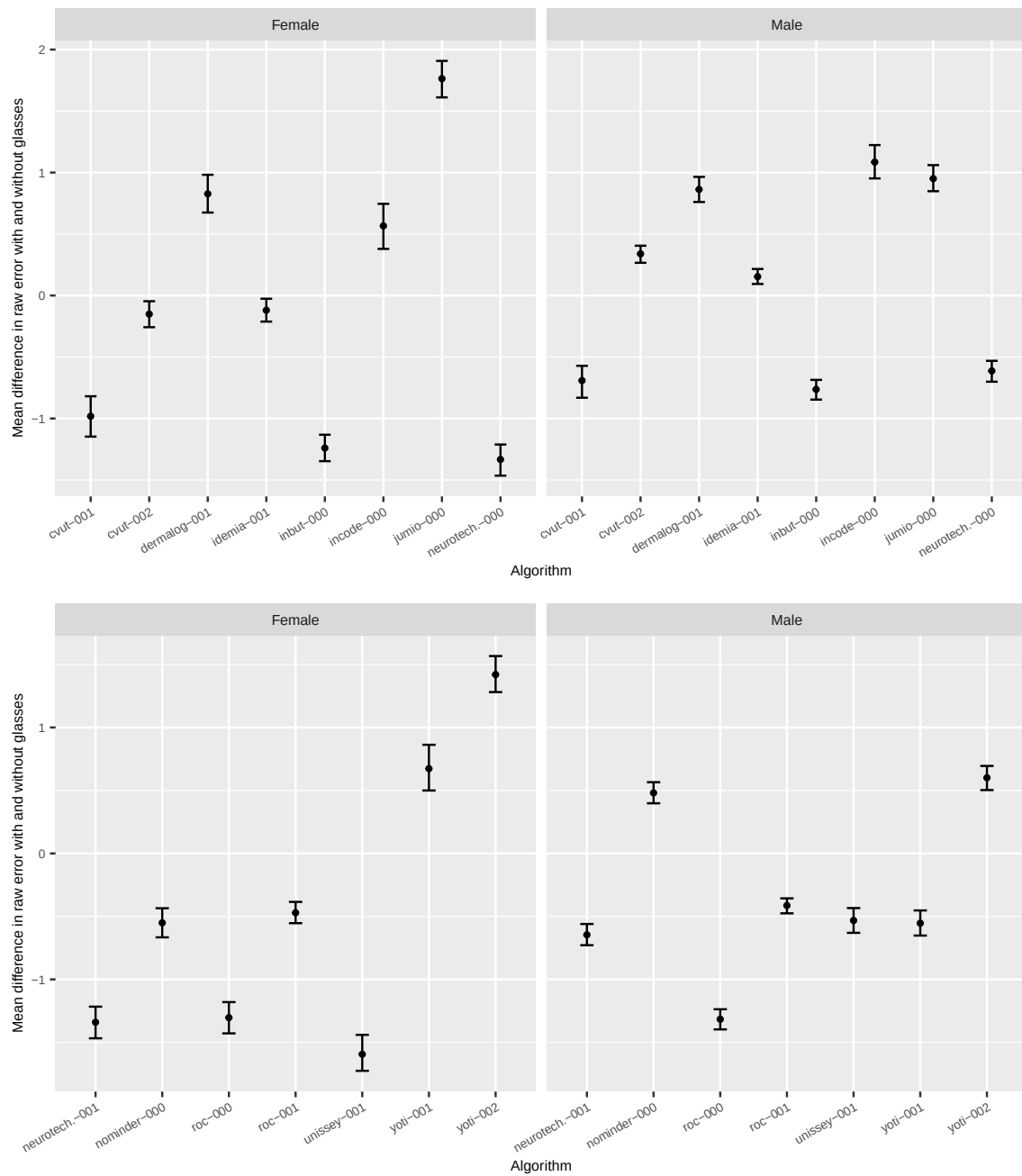
Fig. 43. Difference in age estimation error for border crossing subjects with and without eyeglasses.
