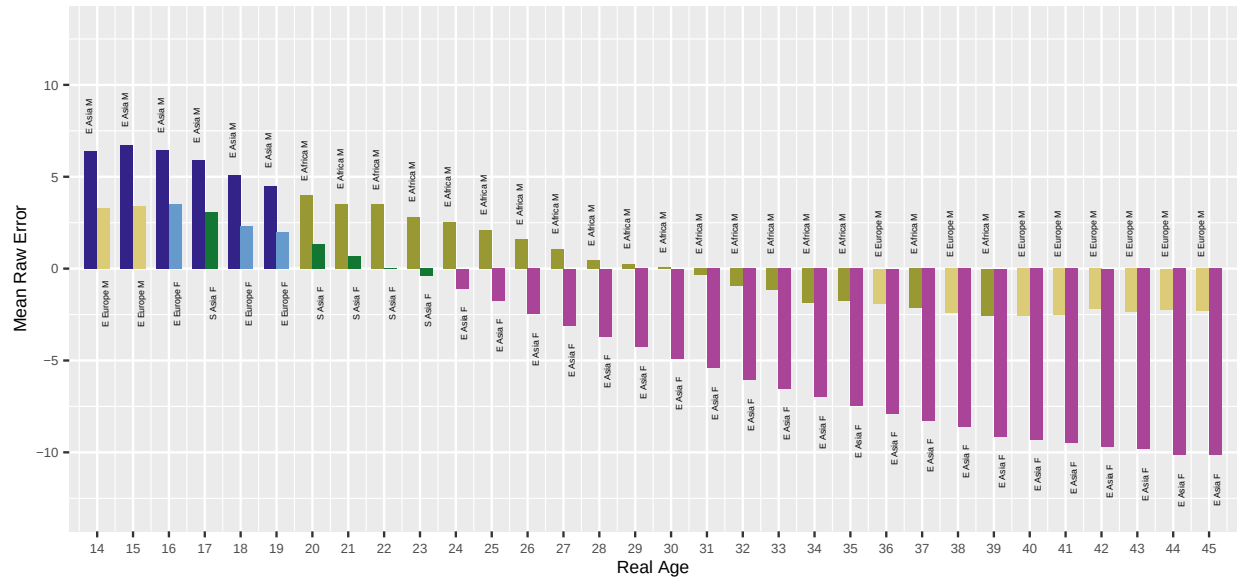
Fig. 28. For algorithm neurotechnology-001 applied to Application photos, the bar chart shows which demographic groups have the highest and lowest mean age estimation error, by age. Values closer to zero are better. Positive values are overestimate and negative values are underestimate.
