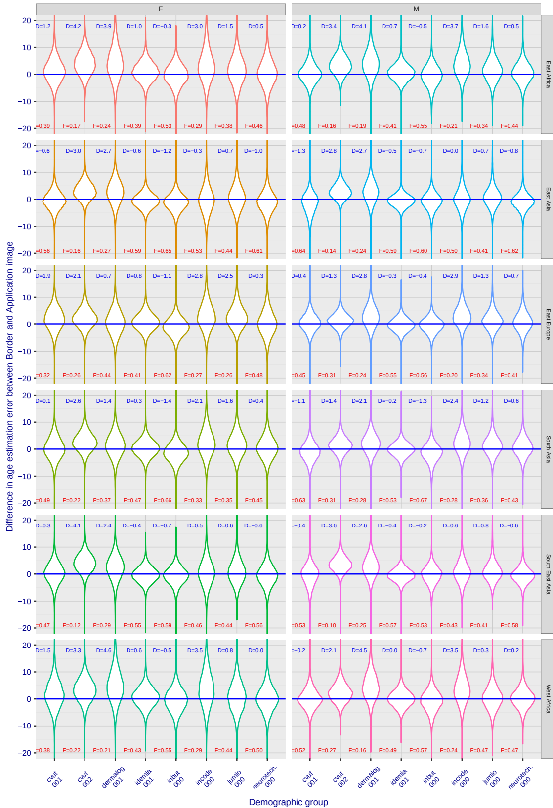
Fig. 40. Distribution of the pairwise age estimation error difference for Border and Application images. Positive values indicate larger error on Border images.
