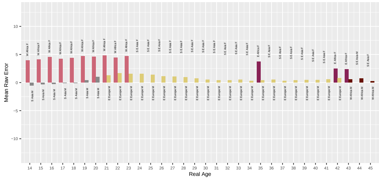
Fig. 37. For algorithm yoti-001 applied to Application photos, the bar chart shows which demographic groups have the highest and lowest mean age estimation error, by age. Values closer to zero are better. Positive values are overestimate and negative values are underestimate.
