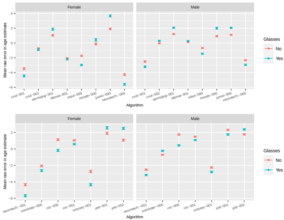
Fig. 42. Mean raw age estimation error for border crossing subjects for whom we have images with and without eyeglasses.
