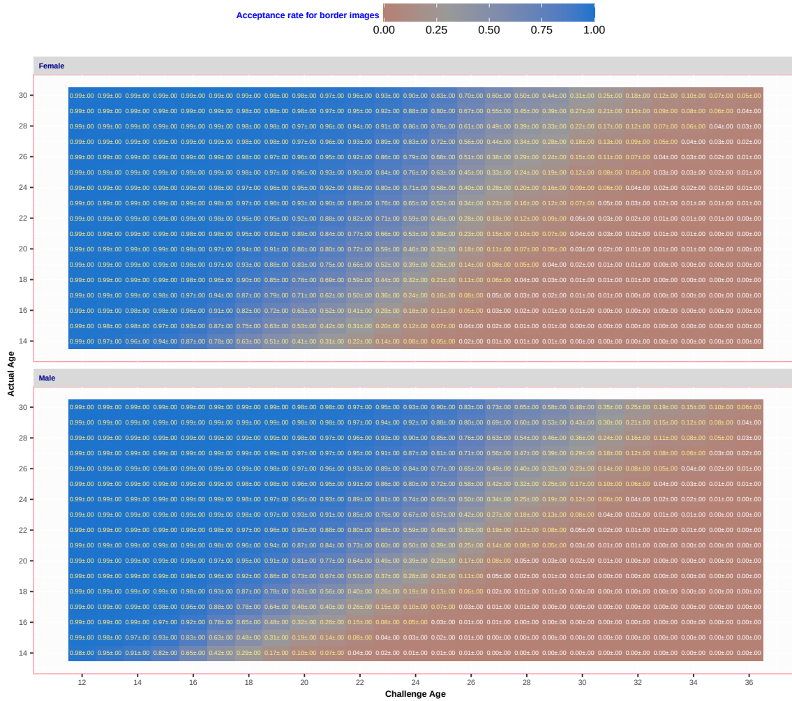
Fig. 44. For algorithm CVUT 001 applied border-crossing photos, the heatmap and text shows proportion of photos of the persons of an actual age are accepted at a particular challenge age.
