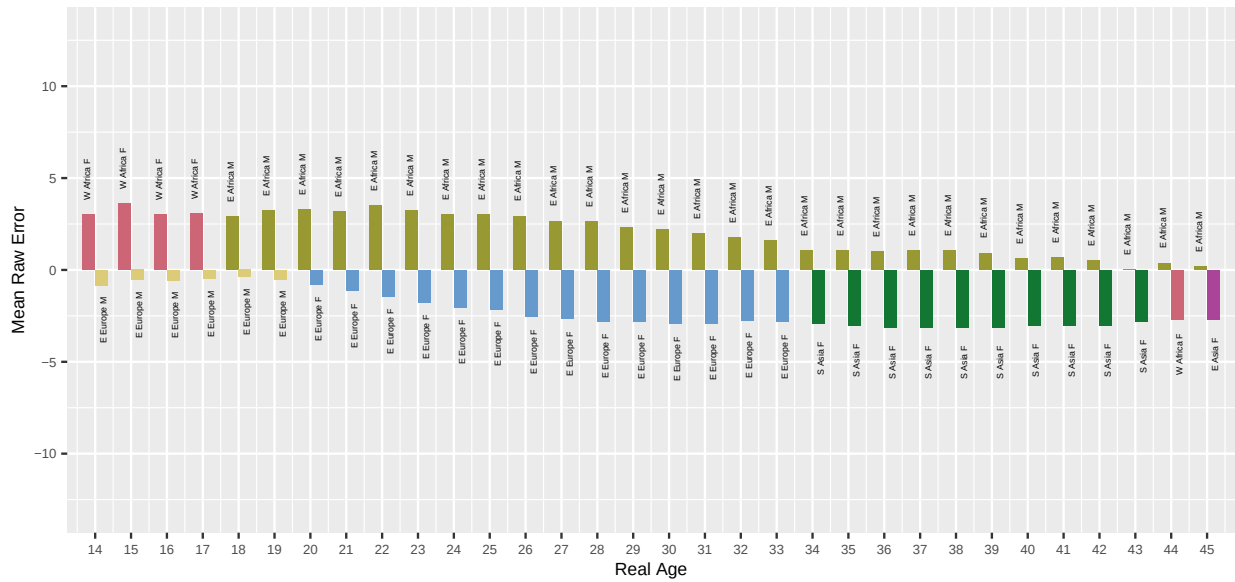
Fig. 19. For algorithm idemia-001 applied to Border photos, the bar chart shows which demographic groups have the highest and lowest mean age estimation error, by age. Values closer to zero are better. Positive values are overestimate and negative values are underestimate.
