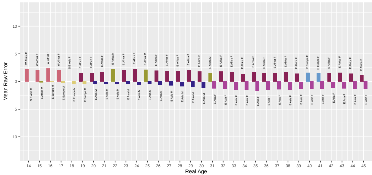
Fig. 22. For algorithm incode-000 applied to Application photos, the bar chart shows which demographic groups have the highest and lowest mean age estimation error, by age. Values closer to zero are better. Positive values are overestimate and negative values are underestimate.
