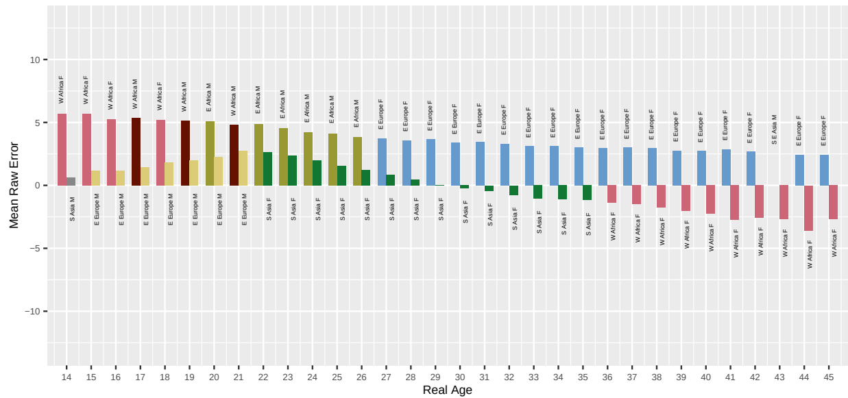
Fig. 38. For algorithm yoti-001 applied to Border photos, the bar chart shows which demographic groups have the highest and lowest mean age estimation error, by age. Values closer to zero are better. Positive values are overestimate and negative values are underestimate.
