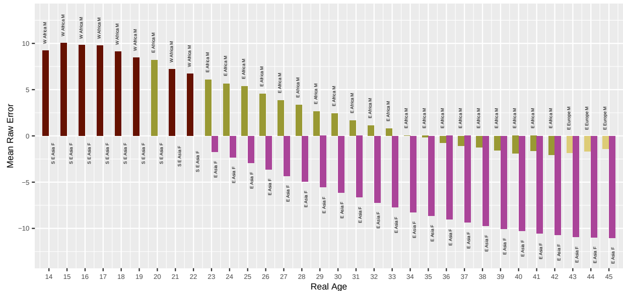
Fig. 27. For algorithm neurotechnology-000 applied to Border photos, the bar chart shows which demographic groups have the highest and lowest mean age estimation error, by age. Values closer to zero are better. Positive values are overestimate and negative values are underestimate.
