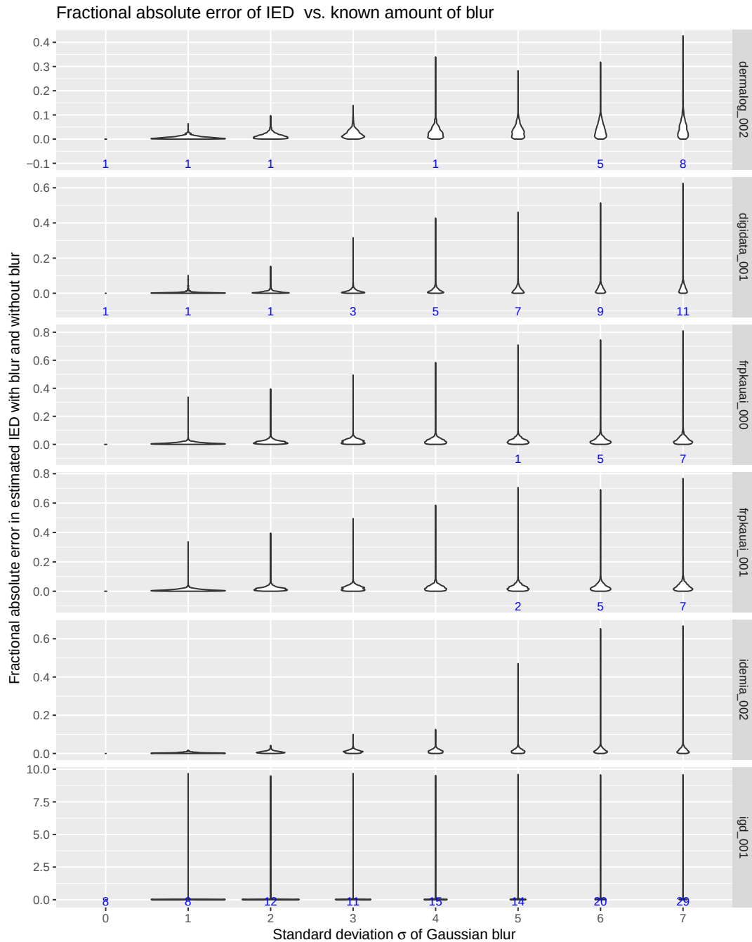
(a) Fractional absolute value of error in inter-eye distance estimates vs. \sigma parameter of Gaussian blur.
