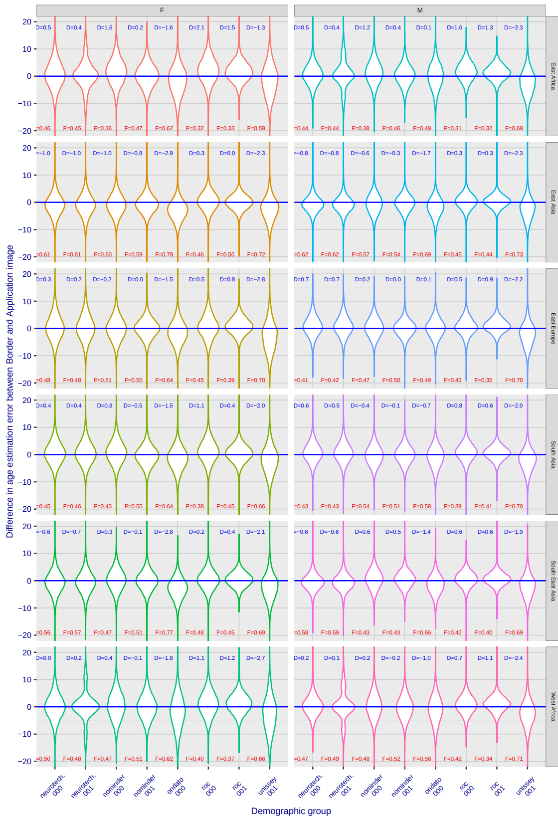
Fig. 46. Distribution of the pairwise age estimation error difference for Border and Application images. Positive values indicate larger error on Border images.
