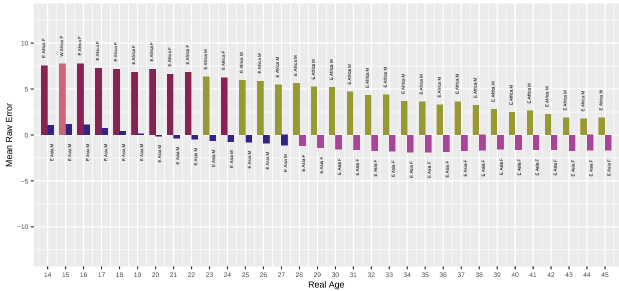
Fig. 25. For algorithm incode-000 applied to Border photos, the bar chart shows which demographic groups have the highest and lowest mean age estimation error, by age. Values closer to zero are better. Positive values are overestimate and negative values are underestimate.
