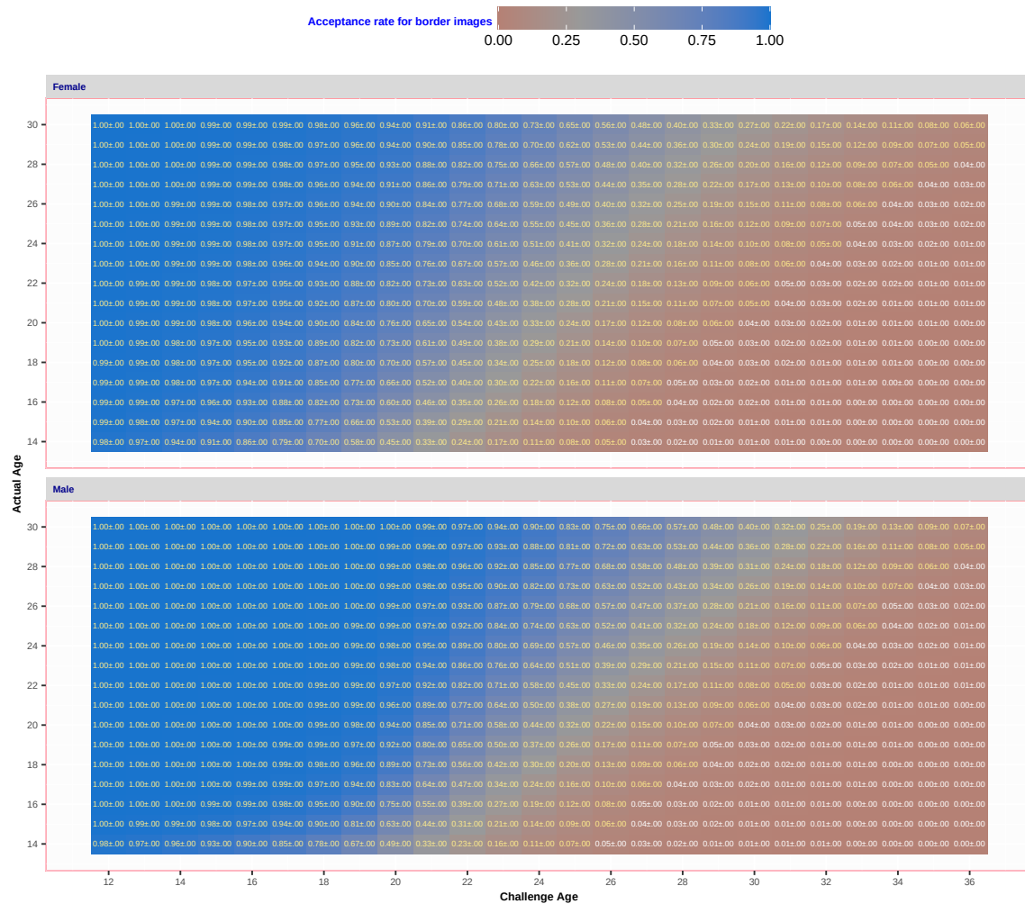
Fig. 54. For algorithm Neurotechnology 000 applied border-crossing photos, the heatmap and text shows proportion of photos of the persons of an actual age are accepted at a particular challenge age.
