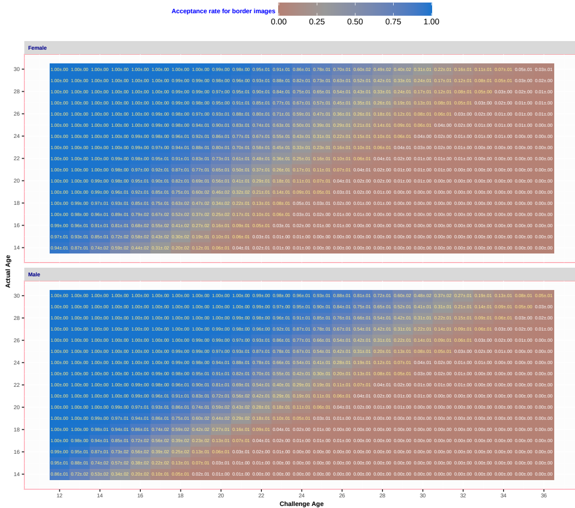
Fig. 52. For algorithm Idemia 001 applied border-crossing photos, the heatmap and text shows proportion of photos of the persons of an actual age are accepted at a particular challenge age.
