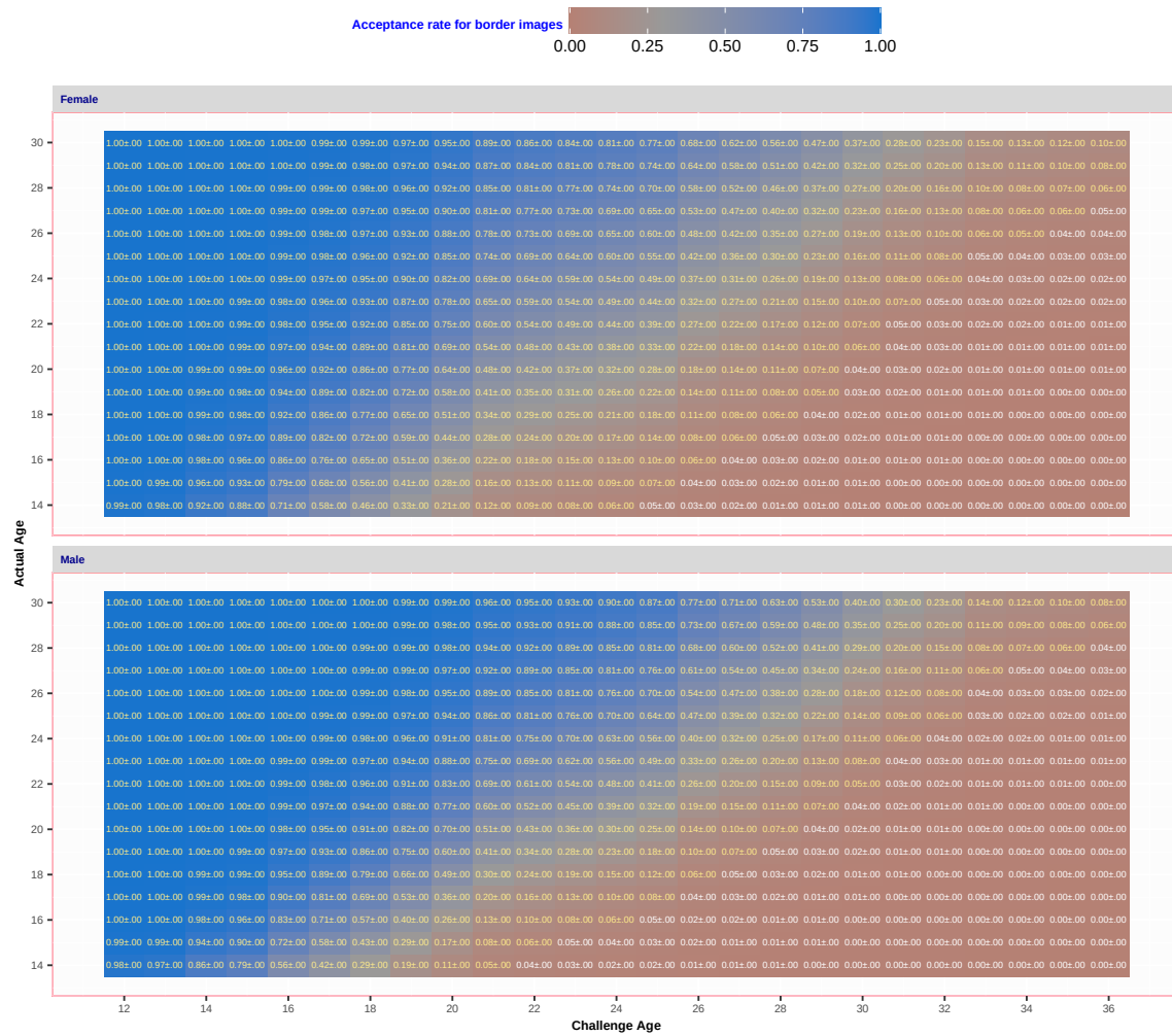
Fig. 58. For algorithm Unissey 001 applied border-crossing photos, the heatmap and text shows proportion of photos of the persons of an actual age are accepted at a particular challenge age.
