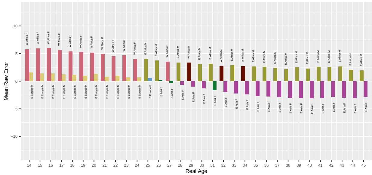
Fig. 35. For algorithm ondato-000 applied to Application photos, the bar chart shows which demographic groups have the highest and lowest mean age estimation error, by age. Values closer to zero are better. Positive values are overestimate and negative values are underestimate.
