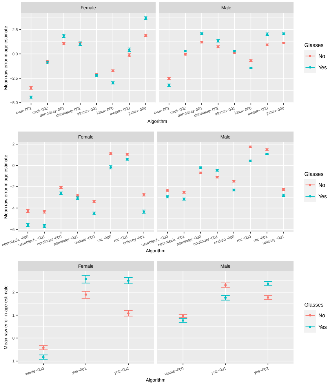
Fig. 48. Mean raw age estimation error for border crossing subjects for whom we have images with and without eyeglasses.
