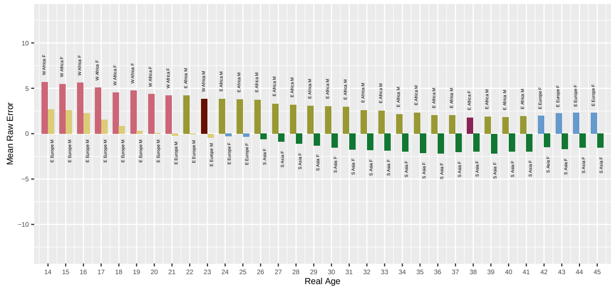
Fig. 36. For algorithm roc-000 applied to Application photos, the bar chart shows which demographic groups have the highest and lowest mean age estimation error, by age. Values closer to zero are better. Positive values are overestimate and negative values are underestimate.
