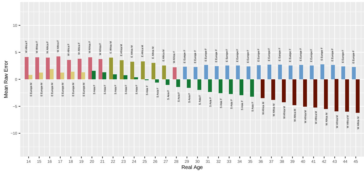
Fig. 39. For algorithm unissey-001 applied to Application photos, the bar chart shows which demographic groups have the highest and lowest mean age estimation error, by age. Values closer to zero are better. Positive values are overestimate and negative values are underestimate.
