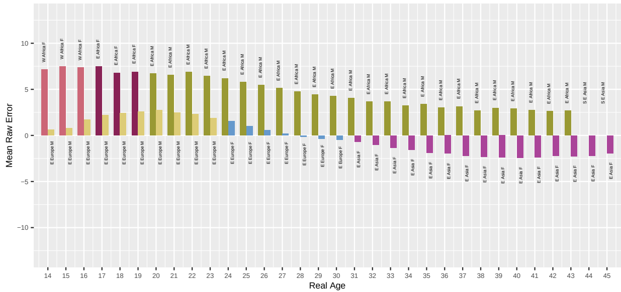
Fig. 41. For algorithm viante-000 applied to Application photos, the bar chart shows which demographic groups have the highest and lowest mean age estimation error, by age. Values closer to zero are better. Positive values are overestimate and negative values are underestimate.
