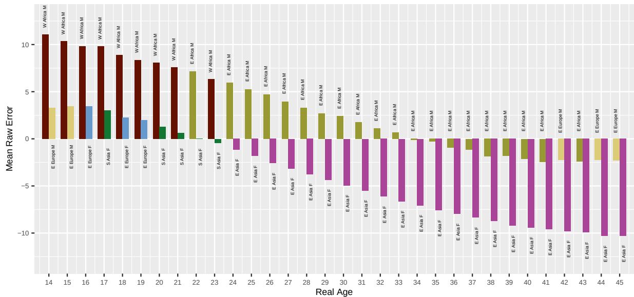
Fig. 28. For algorithm neurotechnology-000 applied to Application photos, the bar chart shows which demographic groups have the highest and lowest mean age estimation error, by age. Values closer to zero are better. Positive values are overestimate and negative values are underestimate.
