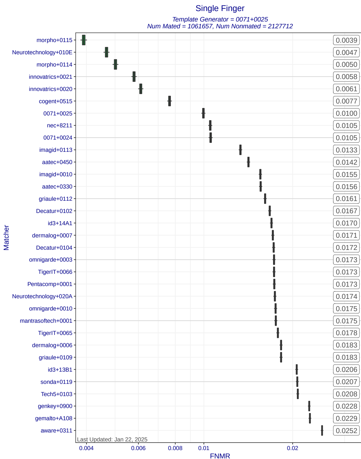
Figure 5: Single Finger FNMNRs at FMR=0.0001 when MINEX III compliant matchers compare templates created by template generator 0071+0025. Each box represents uncertainty about the true FNMR. The box edges mark the 50% confidence intervals while the whiskers mark the 90% confidence intervals. The numbers on the right show the actual computed FNMRs.
