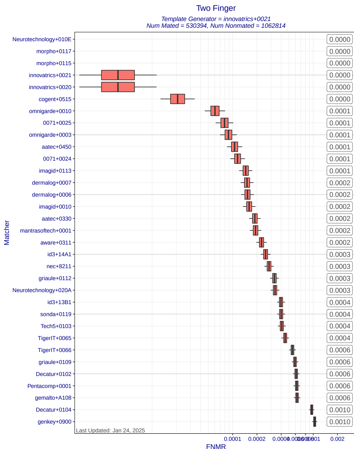
Figure 7: Two Finger FNMR at FMR=0.01 when different matchers compare templates created by template generator innovatrics+0021. Each box represents uncertainty about the true FNMR. The box edges mark the 50% confidence intervals while the whiskers mark the 90% confidence intervals. The numbers on the right show the actual computed FNMRs. Score-level fusion is achieved by averaging the scores for left and right index fingers.
