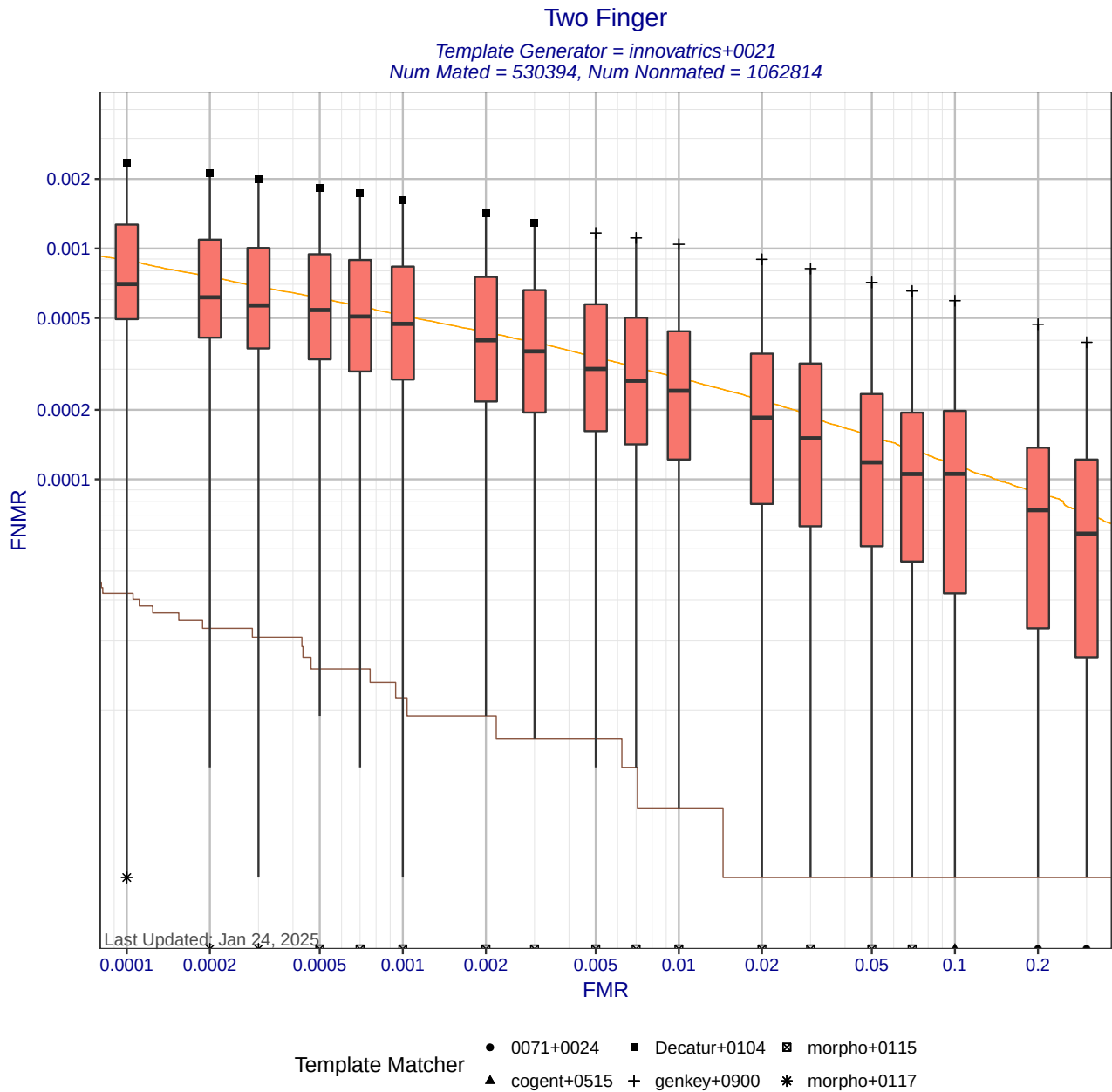
Figure 6: Two Finger DET statistics for template generator innovatrics+0021. Each box shows the distribution of FNMNRs at a fixed FMR across different matchers. The whisker ends show the minimum and maximum FNMNRs. The brown curve shows the DET curve when the matcher and template generators were submitted by the same participant. The orange DET curve shows pooled performance when all matchers use templates created by innovatrics+0021. Score-level fusion is achieved by averaging the scores for left and right index fingers.
