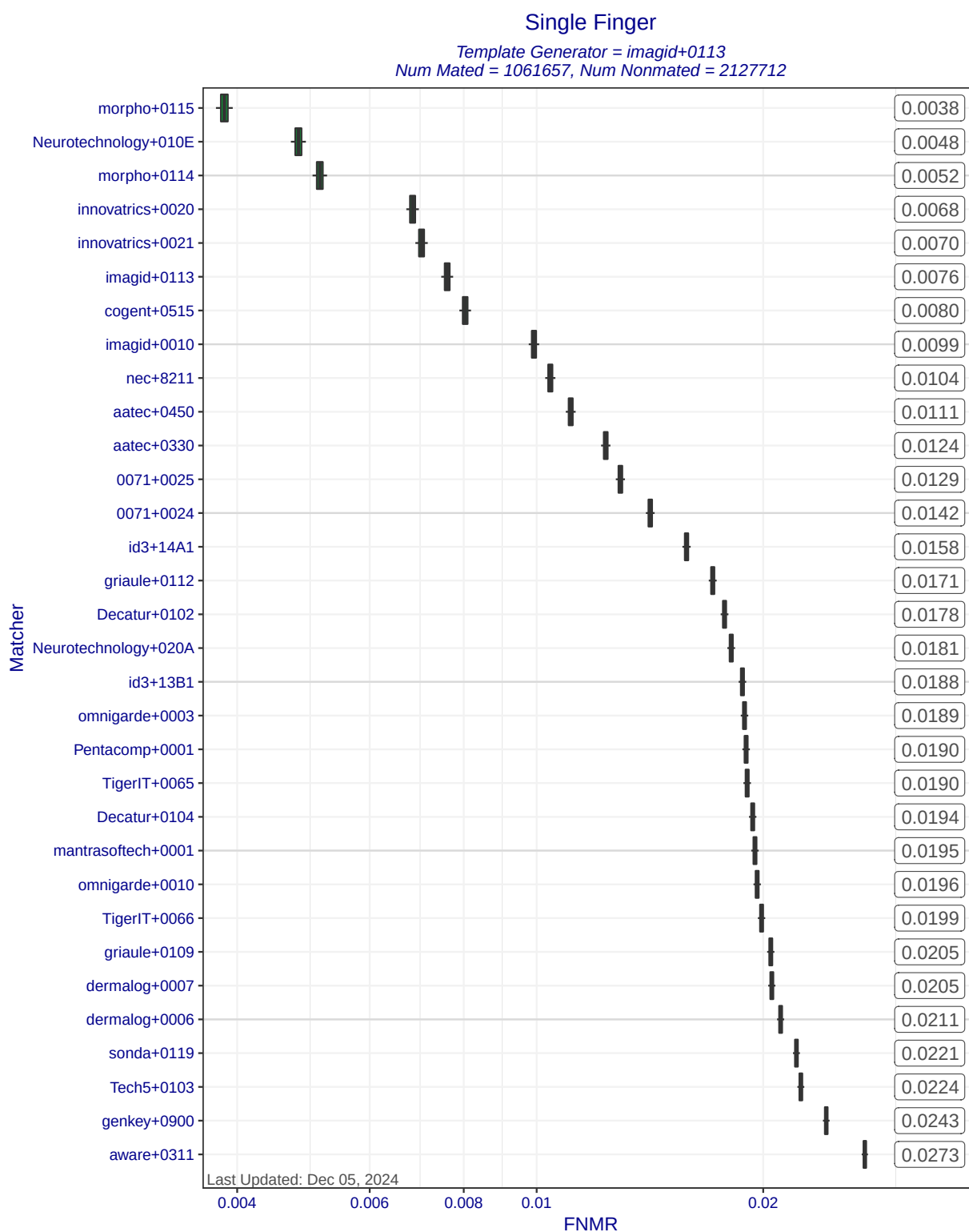
Figure 5: Single Finger FNMRS at FMR=0.0001 when MINEX III compliant matchers compare templates created by template generator imagid+0113. Each box represents uncertainty about the true FNMRS. The box edges mark the 50% confidence intervals while the whiskers mark the 90% confidence intervals. The numbers on the right show the actual computed FNMRS.
