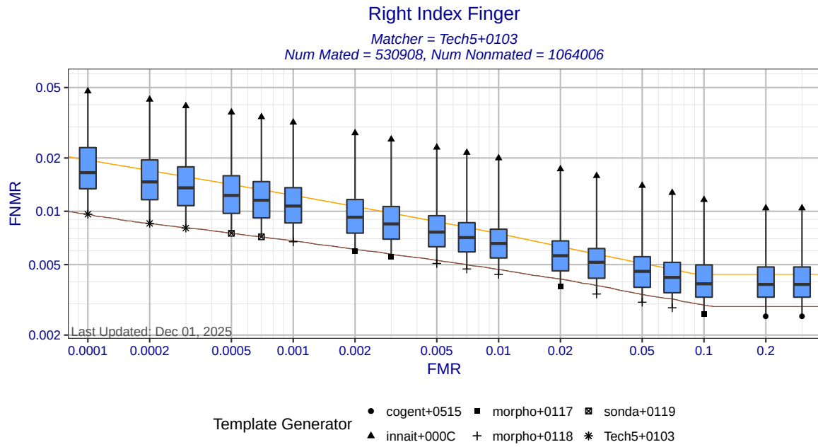
Figure 3: Right index finger DET statistics for matcher Tech5+0103. Each box shows the distribution of FNRs at a fixed FMR across all MINEX III compliant template generators. The ends of the whiskers show the minimum and maximum FNRs. The orange DET curve shows pooled performance against all template generators.
