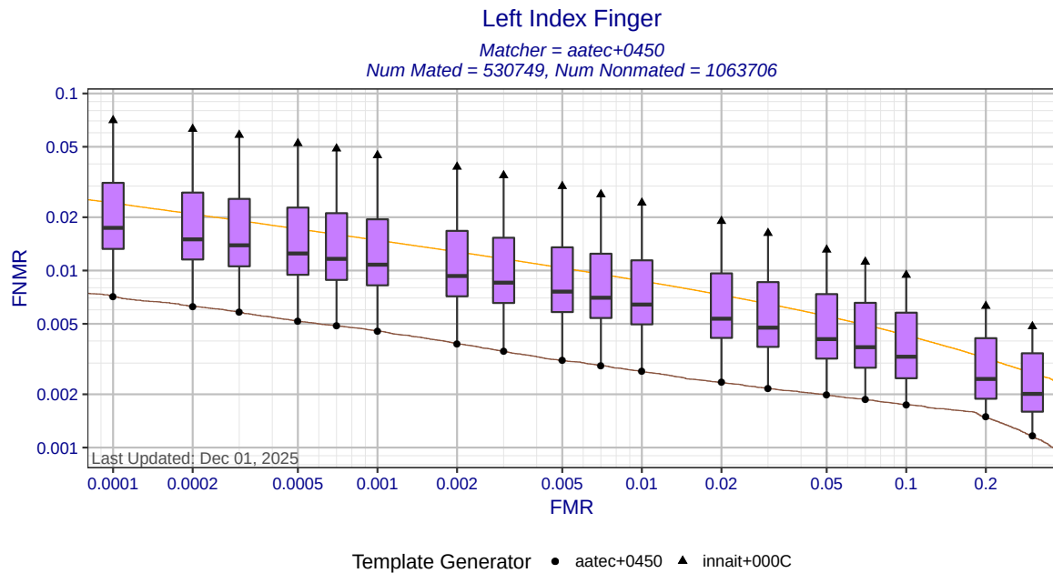
Figure 4: Left index finger DET statistics for matcher aatec+0450. Each box shows the distribution of FNMRs at a fixed FMR across all MINEX III compliant template generators. The ends of the whiskers show the minimum and maximum FNMRs. The orange DET curve shows pooled performance against all template generators.
