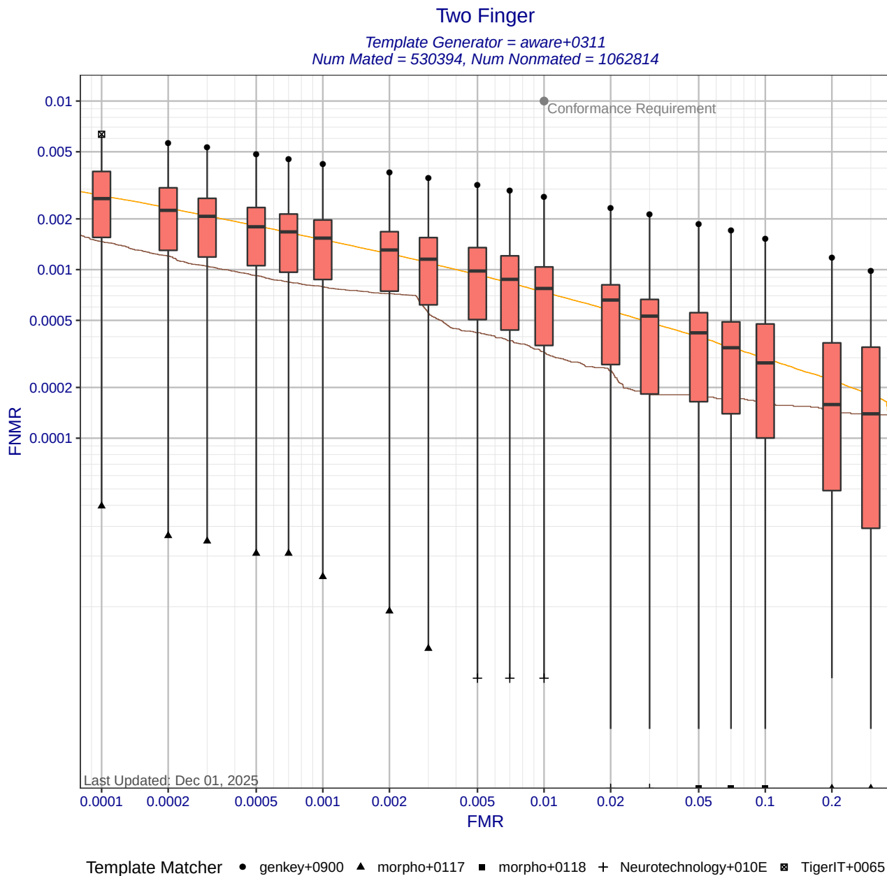
Figure 6: Two Finger DET statistics for template generator aware+0311. Each box shows the distribution of FNRs at a fixed FMR across different matchers. The whisker ends show the minimum and maximum FNRs. The brown curve shows the DET curve when the matcher and template generators were submitted by the same participant. The orange DET curve shows pooled performance when all matchers use templates created by aware+0311. Score-level fusion is achieved by averaging the scores for left and right index fingers.
