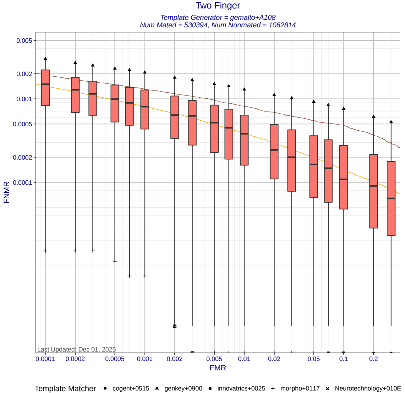
Figure 6: Two Finger DET statistics for template generator gemalto+A108. Each box shows the distribution of FNMIRs at a fixed FMR across different matchers. The whisker ends show the minimum and maximum FNMIRs. The brown curve shows the DET curve when the matcher and template generators were submitted by the same participant. The orange DET curve shows pooled performance when all matchers use templates created by gemalto+A108. Score-level fusion is achieved by averaging the scores for left and right index fingers.
