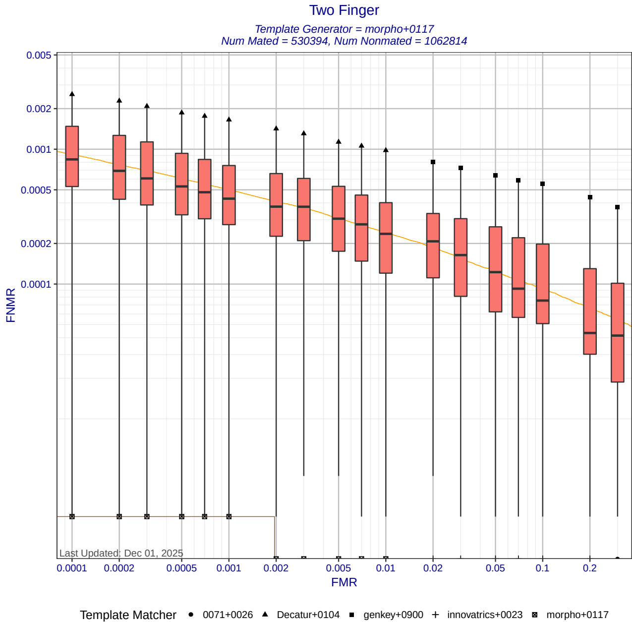
Figure 6: Two Finger DET statistics for template generator morpho+0117. Each box shows the distribution of FNMNRs at a fixed FMR across different matchers. The whisker ends show the minimum and maximum FNMNRs. The brown curve shows the DET curve when the matcher and template generators were submitted by the same participant. The orange DET curve shows pooled performance when all matchers use templates created by morpho+0117. Score-level fusion is achieved by averaging the scores for left and right index fingers.
