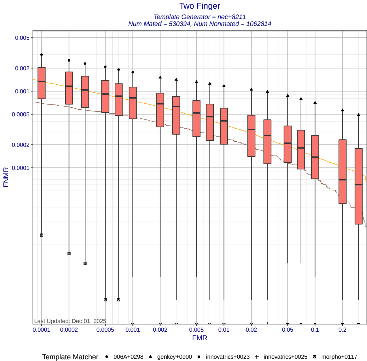
Figure 6: Two Finger DET statistics for template generator nec+8211. Each box shows the distribution of FNMNRs at a fixed FMR across different matchers. The whisker ends show the minimum and maximum FNMNRs. The brown curve shows the DET curve when the matcher and template generators were submitted by the same participant. The orange DET curve shows pooled performance when all matchers use templates created by nec+8211. Score-level fusion is achieved by averaging the scores for left and right index fingers.
