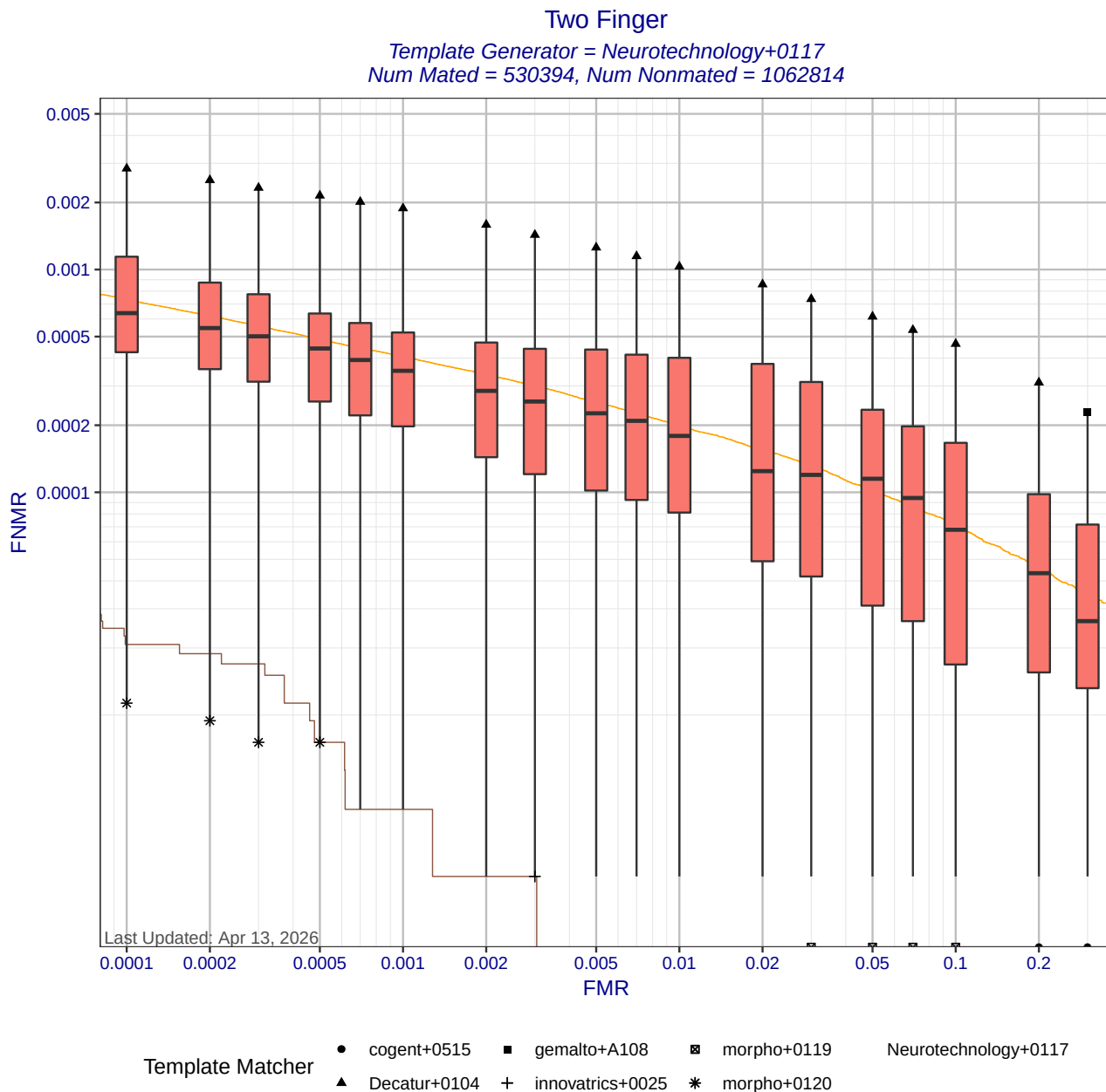
Figure 6: Two Finger DET statistics for template generator Neurotechnology+0117. Each box shows the distribution of FNMNRs at a fixed FMR across different matchers. The whisker ends show the minimum and maximum FNMNRs. The brown curve shows the DET curve when the matcher and template generators were submitted by the same participant. The orange DET curve shows pooled performance when all matchers use templates created by Neurotechnology+0117. Score-level fusion is achieved by averaging the scores for left and right index fingers.
