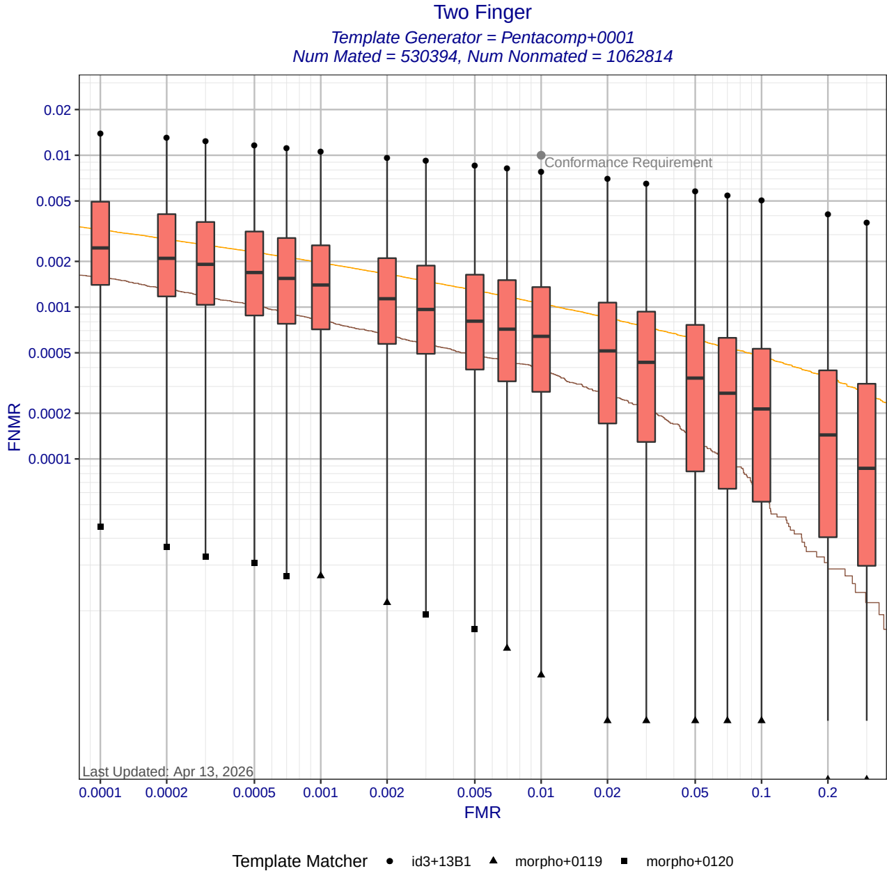
Figure 6: Two Finger DET statistics for template generator Pentacomp+0001. Each box shows the distribution of FNMNRs at a fixed FMR across different matchers. The whisker ends show the minimum and maximum FNMNRs. The brown curve shows the DET curve when the matcher and template generators were submitted by the same participant. The orange DET curve shows pooled performance when all matchers use templates created by Pentacomp+0001. Score-level fusion is achieved by averaging the scores for left and right index fingers.
