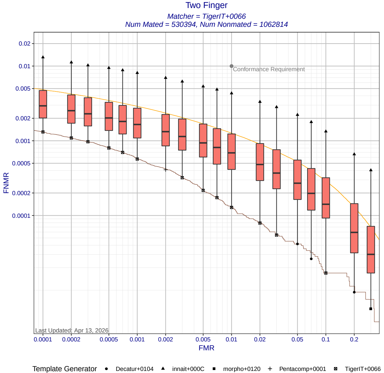
Figure 7: Two finger DET statistics for matcher TigerIT+0066. Each box shows the distribution of FNMRs at a fixed FMR across all MINEX III compliant template generators. The whisker ends show the minimum and maximum FNMRs. The orange DET curve shows pooled performance against all template generators. Score-level fusion is achieved by averaging the scores for left and right index fingers.
