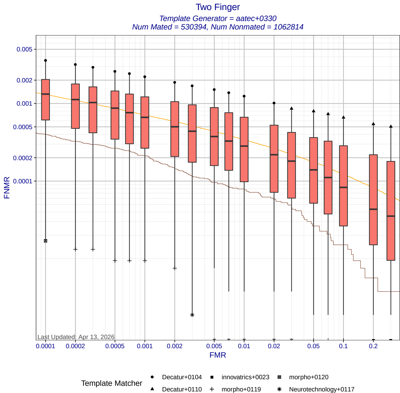
Figure 6: Two Finger DET statistics for template generator aatec+0330. Each box shows the distribution of FNRs at a fixed FMR across different matchers. The whisker ends show the minimum and maximum FNRs. The brown curve shows the DET curve when the matcher and template generators were submitted by the same participant. The orange DET curve shows pooled performance when all matchers use templates created by aatec+0330. Score-level fusion is achieved by averaging the scores for left and right index fingers.
