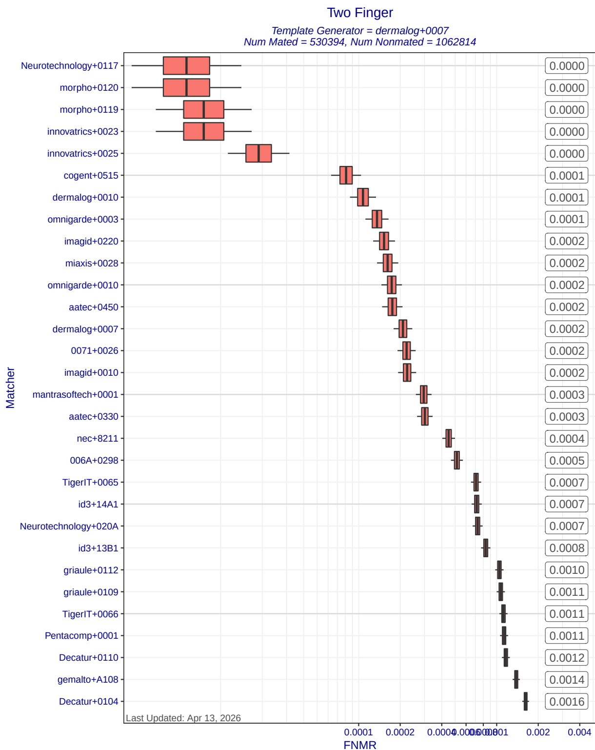
Figure 7: Two Finger FNMR at FMR=0.01 when different matchers compare templates created by template generator dermalog+0007. Each box represents uncertainty about the true FNMR. The box edges mark the 50% confidence intervals while the whiskers mark the 90% confidence intervals. The numbers on the right show the actual computed FNMRs. Score-level fusion is achieved by averaging the scores for left and right index fingers.
