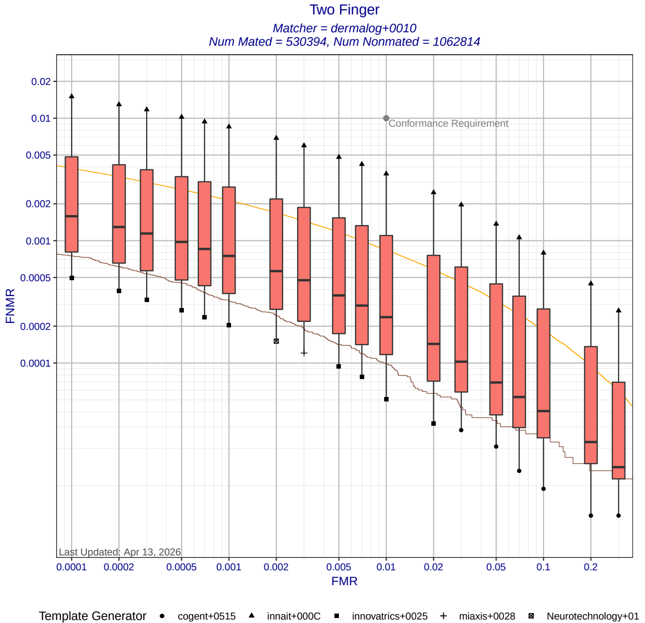
Figure 7: Two finger DET statistics for matcher dermalog+0010. Each box shows the distribution of FNMRs at a fixed FMR across all MINEX III compliant template generators. The whisker ends show the minimum and maximum FNMRs. The orange DET curve shows pooled performance against all template generators. Score-level fusion is achieved by averaging the scores for left and right index fingers.
