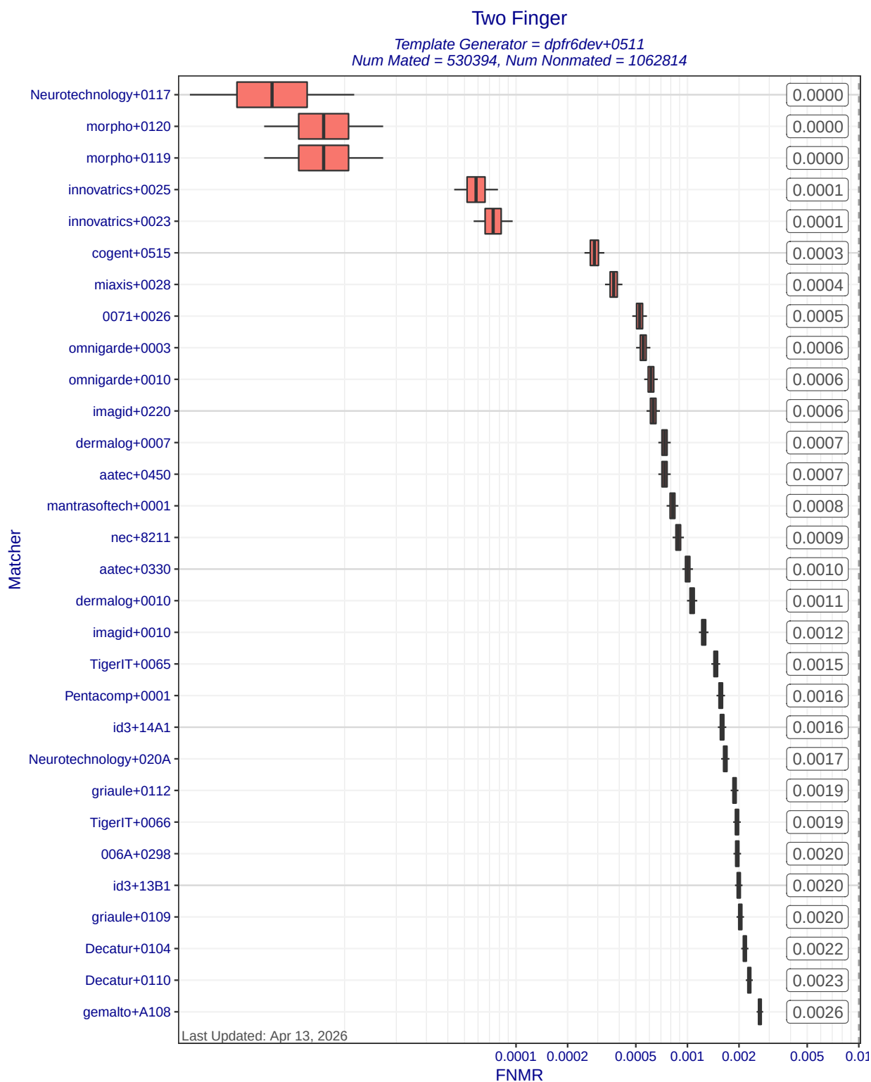
Figure 7: Two Finger FNMR at FMR=0.01 when different matchers compare templates created by template generator dpfr6dev+0511. Each box represents uncertainty about the true FNMR. The box edges mark the 50% confidence intervals while the whiskers mark the 90% confidence intervals. The numbers on the right show the actual computed FNMRs. Score-level fusion is achieved by averaging the scores for left and right index fingers.
