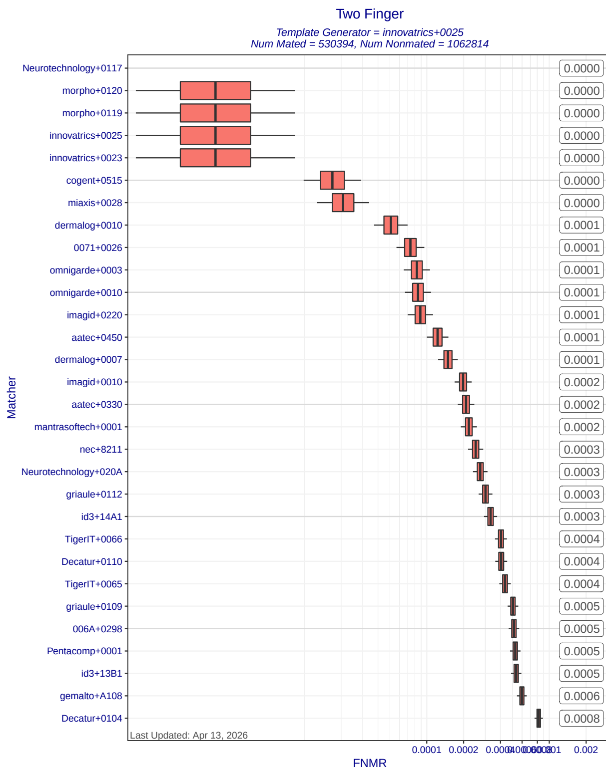
Figure 7: Two Finger FNMR at FMR=0.01 when different matchers compare templates created by template generator innovatrics+0025. Each box represents uncertainty about the true FNMR. The box edges mark the 50% confidence intervals while the whiskers mark the 90% confidence intervals. The numbers on the right show the actual computed FNMRs. Score-level fusion is achieved by averaging the scores for left and right index fingers.
