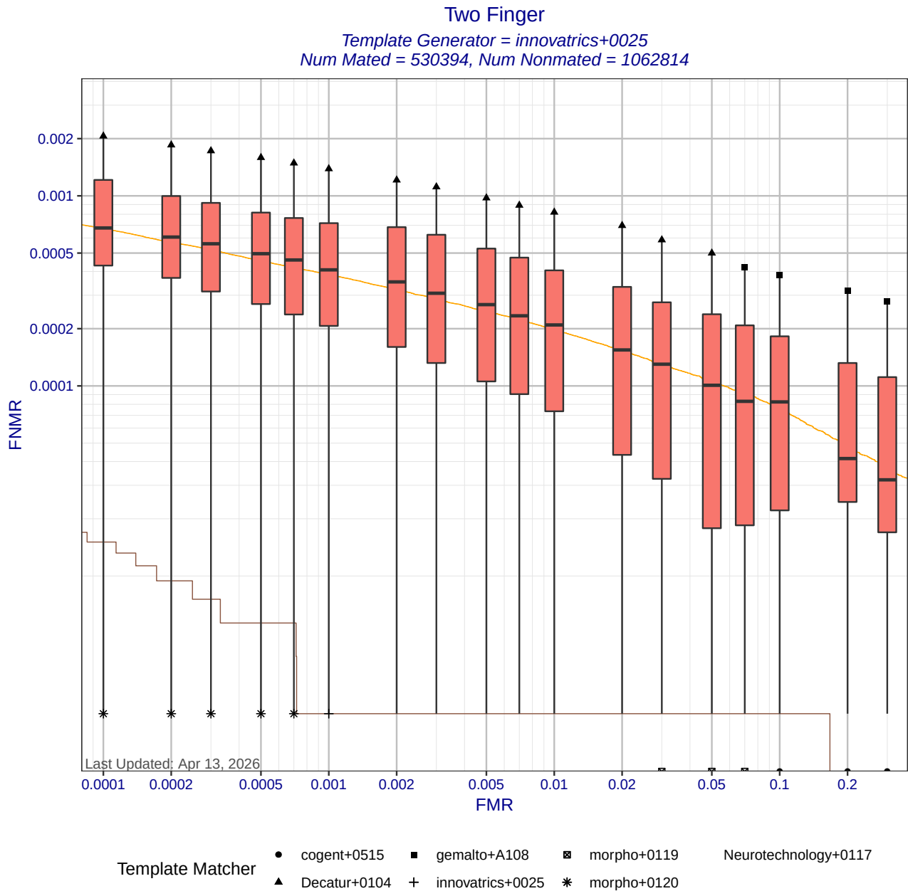
Figure 6: Two Finger DET statistics for template generator innovatrics+0025. Each box shows the distribution of FNMNRs at a fixed FMR across different matchers. The whisker ends show the minimum and maximum FNMNRs. The brown curve shows the DET curve when the matcher and template generators were submitted by the same participant. The orange DET curve shows pooled performance when all matchers use templates created by innovatrics+0025. Score-level fusion is achieved by averaging the scores for left and right index fingers.
