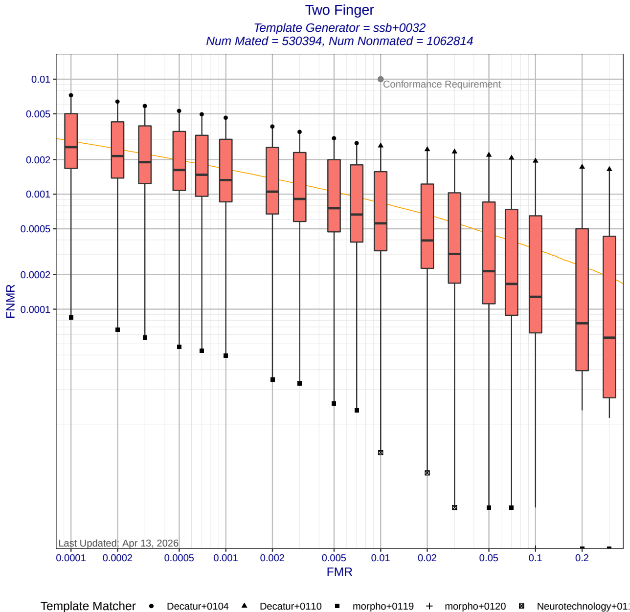
Figure 6: Two Finger DET statistics for template generator ssb+0032. Each box shows the distribution of FNMNRs at a fixed FMR across different matchers. The whisker ends show the minimum and maximum FNMNRs. The orange DET curve shows pooled performance when all matchers use templates created by ssb+0032. Score-level fusion is achieved by averaging the scores for left and right index fingers.
