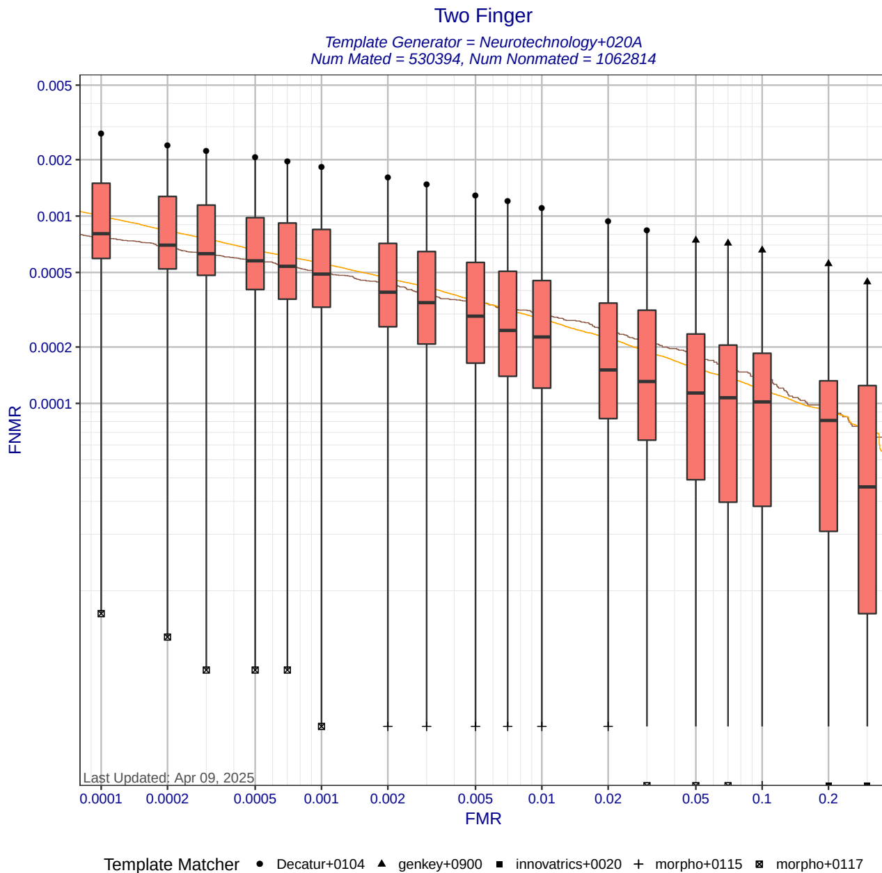
Figure 6: Two Finger DET statistics for template generator Neurotechnology+020A. Each box shows the distribution of FNMNRs at a fixed FMR across different matchers. The whisker ends show the minimum and maximum FNMNRs. The brown curve shows the DET curve when the matcher and template generators were submitted by the same participant. The orange DET curve shows pooled performance when all matchers use templates created by Neurotechnology+020A. Score-level fusion is achieved by averaging the scores for left and right index fingers.
