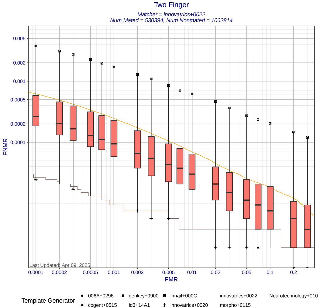
Figure 7: Two finger DET statistics for matcher innovatrics+0022. Each box shows the distribution of FNMRs at a fixed FMR across all MINEX III compliant template generators. The whisker ends show the minimum and maximum FNMRs. The orange DET curve shows pooled performance against all template generators. Score-level fusion is achieved by averaging the scores for left and right index fingers.
