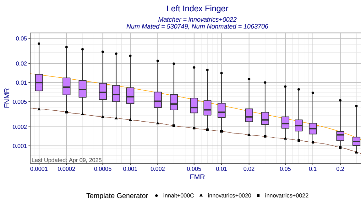
Figure 4: Left index finger DET statistics for matcher innovatrics+0022. Each box shows the distribution of FNRs at a fixed FMR across all MINEX III compliant template generators. The ends of the whiskers show the minimum and maximum FNRs. The orange DET curve shows pooled performance against all template generators.
