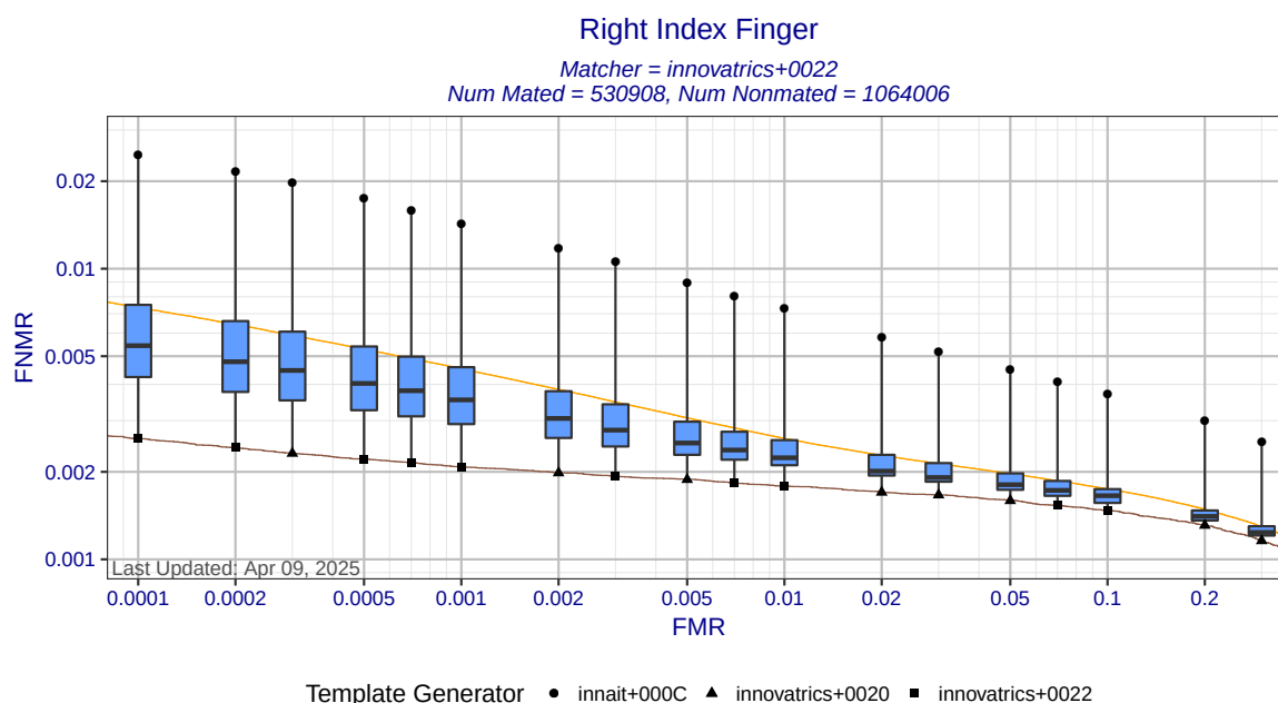
Figure 3: Right index finger DET statistics for matcher innovatrics+0022. Each box shows the distribution of FNRs at a fixed FMR across all MINEX III compliant template generators. The ends of the whiskers show the minimum and maximum FNRs. The orange DET curve shows pooled performance against all template generators.
