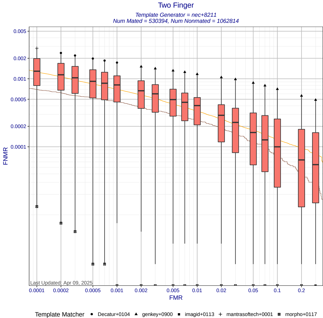
Figure 6: Two Finger DET statistics for template generator nec+8211. Each box shows the distribution of FNMIRs at a fixed FMR across different matchers. The whisker ends show the minimum and maximum FNMIRs. The brown curve shows the DET curve when the matcher and template generators were submitted by the same participant. The orange DET curve shows pooled performance when all matchers use templates created by nec+8211. Score-level fusion is achieved by averaging the scores for left and right index fingers.
