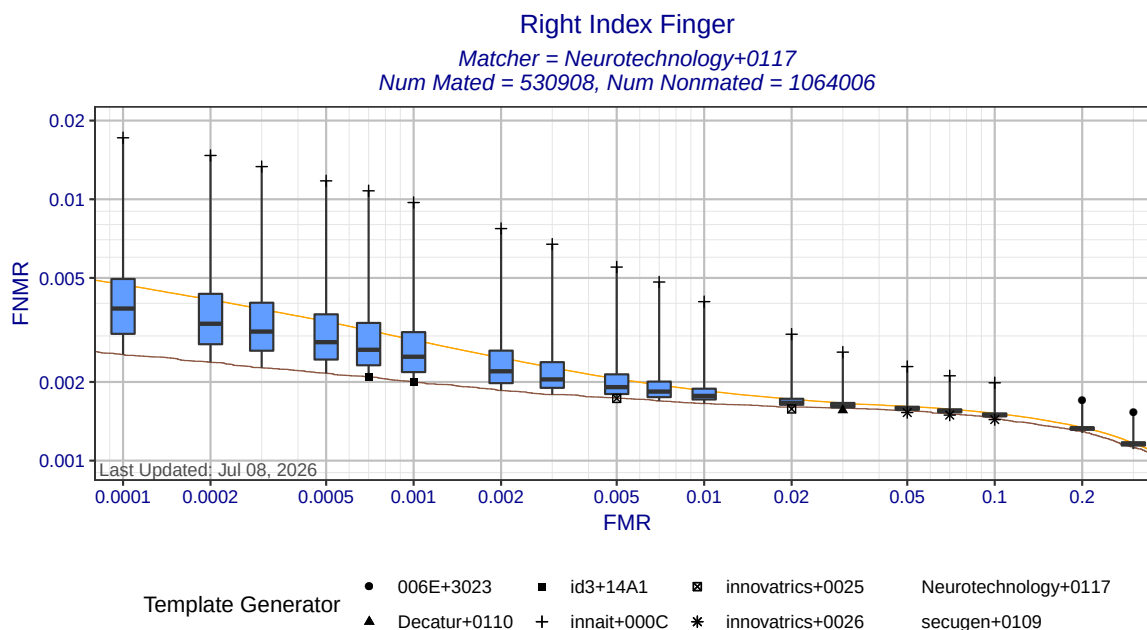
Figure 3: Right index finger DET statistics for matcher Neurotechnology+0117. Each box shows the distribution of FNR at a fixed FMR across all MINEX III compliant template generators. The ends of the whiskers show the minimum and maximum FNRs. The orange DET curve shows pooled performance against all template generators.
