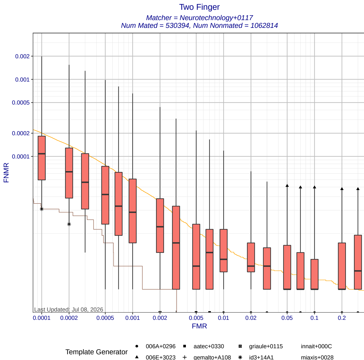
Figure 7: Two finger DET statistics for matcher Neurotechnology+0117. Each box shows the distribution of FNMRs at a fixed FMR across all MINEX III compliant template generators. The whisker ends show the minimum and maximum FNMRs. The orange DET curve shows pooled performance against all template generators. Score-level fusion is achieved by averaging the scores for left and right index fingers.
