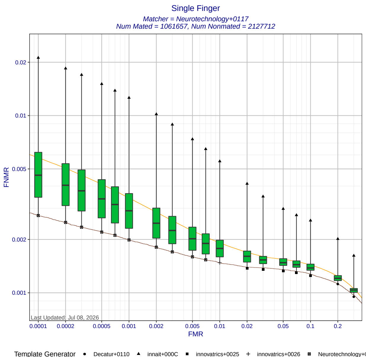
Figure 2: Single finger DET statistics for matcher Neurotechnology+0117. Each box shows the distribution of FNMRs at a fixed FMR across all MINEX III compliant template generators. The ends of the whiskers show the minimum and maximum FNMRs. The orange DET curve shows pooled performance against all template generators.
