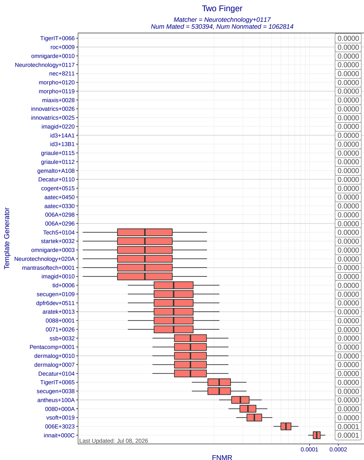
Figure 8: Two finger FNMR at FMR=0.01 when matcher Neurotechnology+0117 compares templates created by different template generators. Each box represents uncertainty about the true FNMR. The box edges mark the 50% confidence intervals while the whiskers mark the 90% confidence intervals. The numbers on the right show the actual computed FNMRs. Score-level fusion is achieved by averaging the scores for left and right index fingers.
