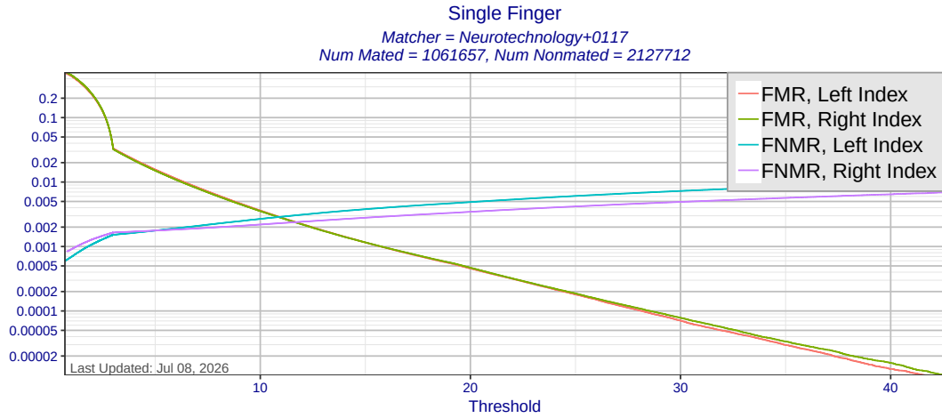
Figure 11: Single finger FMR and FNMR as a function of score threshold for matcher Neurotechnology+0117 using templates created by all MINEX III compliant template generators. Separate curves are presented for left and right index fingers.
