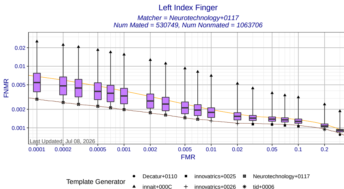
Figure 4: Left index finger DET statistics for matcher Neurotechnology+0117. Each box shows the distribution of FNRs at a fixed FMR across all MINEX III compliant template generators. The ends of the whiskers show the minimum and maximum FNRs. The orange DET curve shows pooled performance against all template generators.
