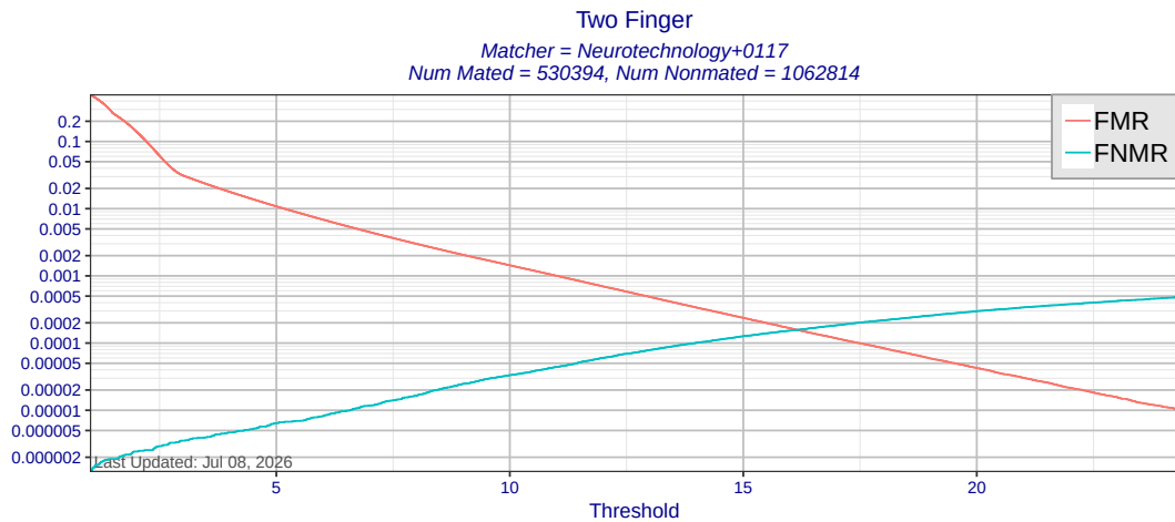
Figure 12: Two finger FMR and FNMR as a function of score threshold for matcher Neurotechnology+0117 using templates created by all MINEX III compliant template generators. Score-level fusion is achieved by averaging scores for the left and right index fingers.
