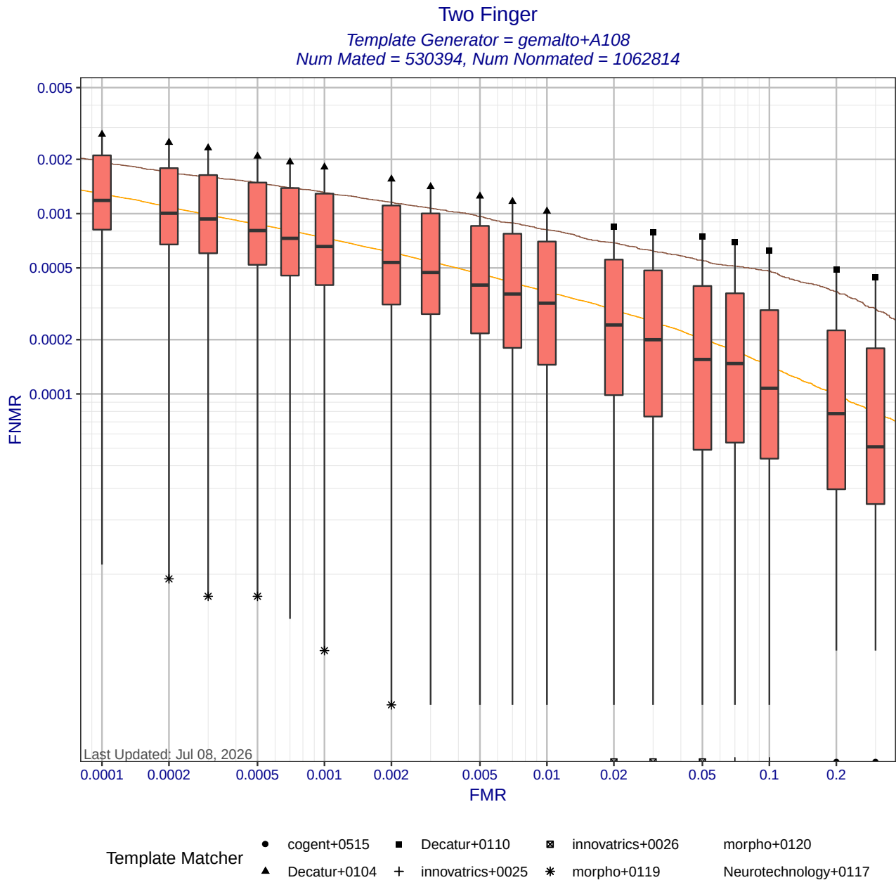
Figure 6: Two Finger DET statistics for template generator gemalto+A108. Each box shows the distribution of FNRs at a fixed FMR across different matchers. The whisker ends show the minimum and maximum FNRs. The brown curve shows the DET curve when the matcher and template generators were submitted by the same participant. The orange DET curve shows pooled performance when all matchers use templates created by gemalto+A108. Score-level fusion is achieved by averaging the scores for left and right index fingers.
