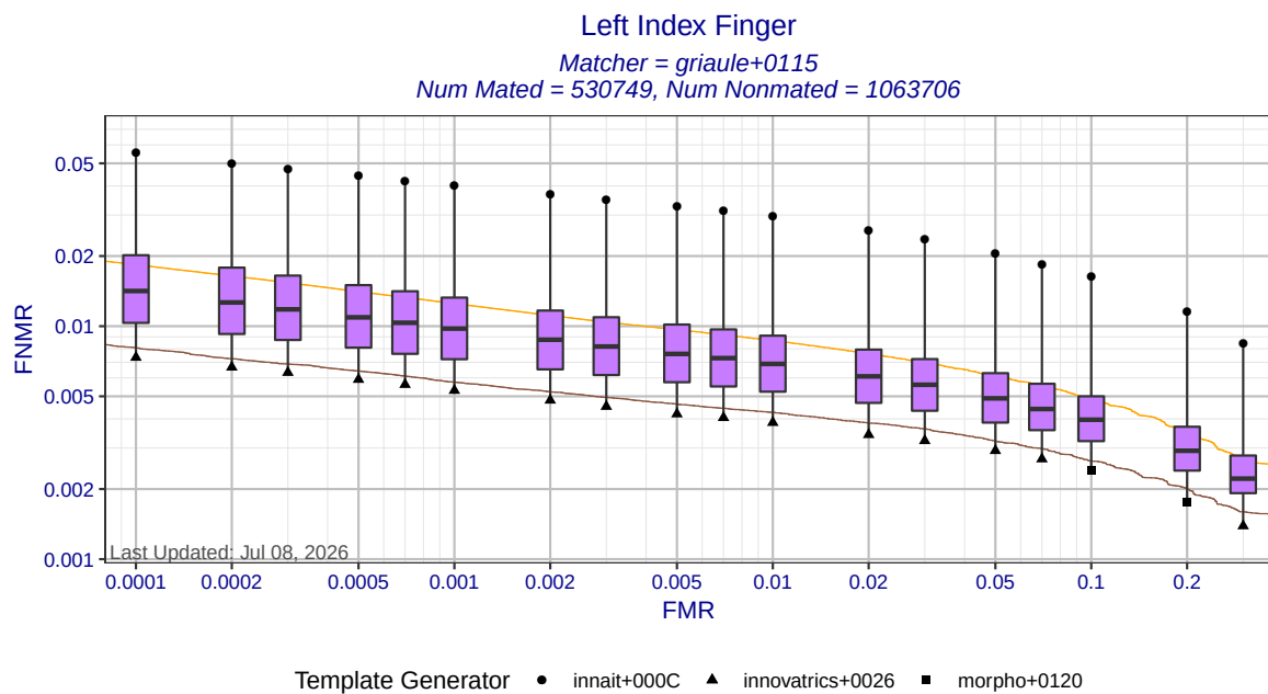
Figure 4: Left index finger DET statistics for matcher griaule+0115. Each box shows the distribution of FNRs at a fixed FMR across all MINEX III compliant template generators. The ends of the whiskers show the minimum and maximum FNRs. The orange DET curve shows pooled performance against all template generators.
