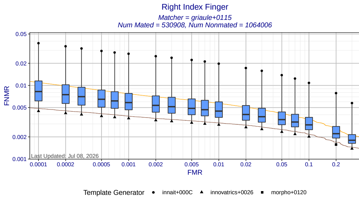
Figure 3: Right index finger DET statistics for matcher griaule+0115. Each box shows the distribution of FNR at a fixed FMR across all MINEX III compliant template generators. The ends of the whiskers show the minimum and maximum FNRs. The orange DET curve shows pooled performance against all template generators.
